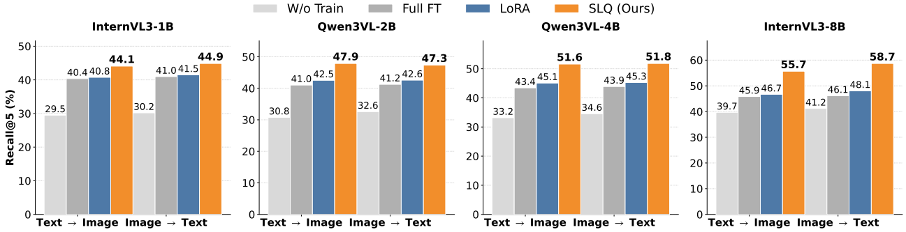
Figure 5. Performance comparison on KARR-Bench. Left to Right: Results on InternVL3-1B, Qwen3VL-2B, Qwen3VL-4B, and InternVL3-8B. Our method (shown in Orange ) consistently outperforms both invasive tuning baselines. Specifically, on the strongest InternVL3-8B backbone, our method achieves significant gains over LoRA and Full FT. These results indicate that preserving a frozen backbone while SLQ is effective for knowledge-aware reasoning retrieval.
