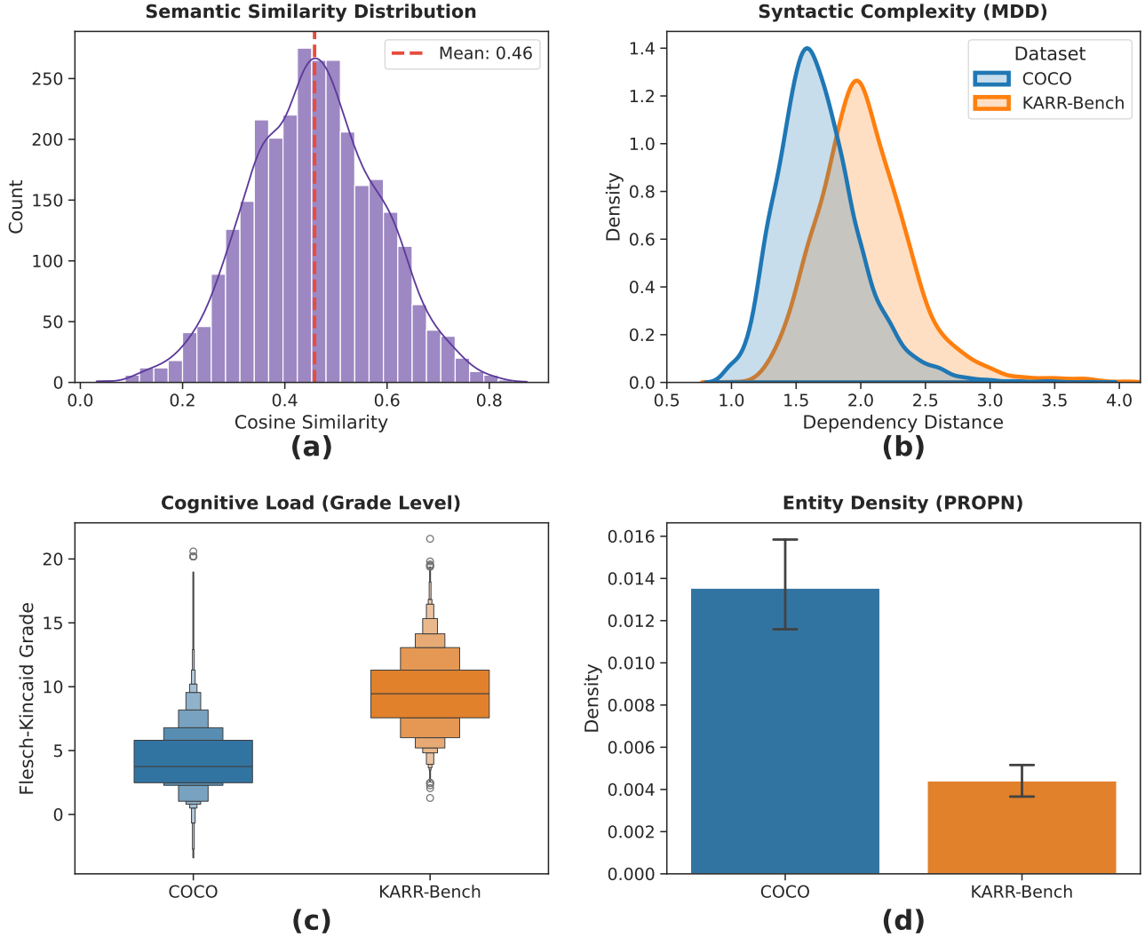
Figure 8. Linguistic and Semantic Comparison between COCO and KARR-Bench. (a) The cosine similarity distribution demonstrates that KARR-Bench Captions maintain semantic relevance to the visual content despite abstraction. (b) KARR-Bench exhibits significantly higher Syntactic Complexity (MDD). (c) The Cognitive Load (Flesch-Kincaid Grade Level) doubles from COCO to KARR-Bench, indicating a shift to advanced reading comprehension. (d) The drastic drop in Entity Density (Proper Nouns) confirms the removal of explicit naming cues.
