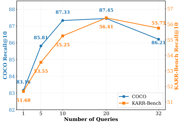
Figure 7. Ablation on the number of queries. The left axis shows the performance on COCO while the right axis shows on KARR-Bench.
