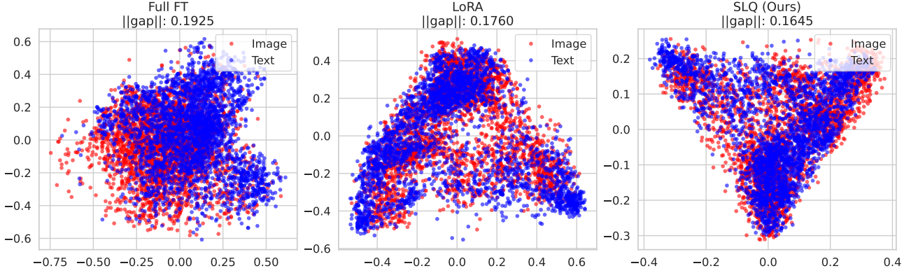
Figure 6. Visualization of the unified representation space using PCA. Red points represent Image embeddings, and Blue points represent Text embeddings. Full FT and LoRA exhibit a noticeably broader spatial spread. In contrast, SLQ maintains a much more compact distribution, resulting in a smaller centroid distance gap and demonstrating superior cross-modal alignment.
