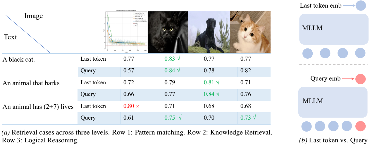
Figure 2. Diagnostic pilot study. We compare the zero-shot retrieval performance of the last token baseline against query token method on the InternVL3-1B backbone. The retrieval score based on cosine similarity is reported as the metric. The results suggest that the query token method better aggregates global context, enabling implicit reasoning for retrieval.
