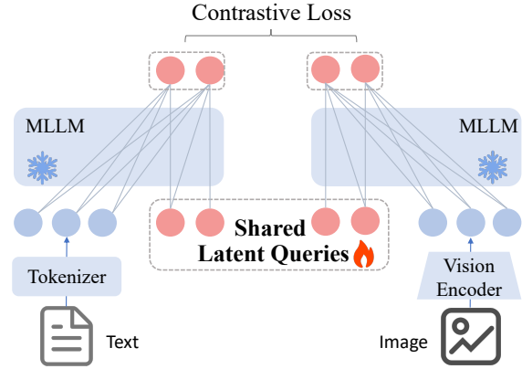
Figure 4. Overview of the SLQ framework. SLQ bridges the modality gap using a set of Shared Latent Queries that interact with the frozen MLLM via causal attention. The term “Shared” indicates that the same set of queries is appended to both image and text tokens, projecting them into a unified embedding space. During training, the MLLM backbone remains frozen, and only the queries are optimized via the contrastive objective to align vision and language representations.
