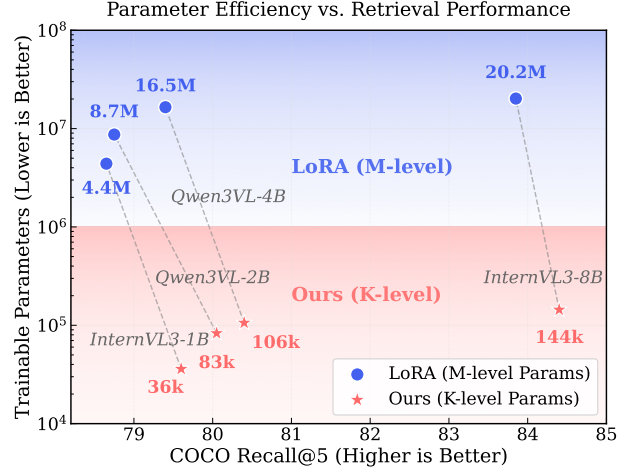
Figure 1. Parameter Efficiency vs. Retrieval Performance. We compare the number of trainable parameters against the retrieval performance, calculated as the average Recall@5 of COCO imageto-text and text-to-image retrieval. Our method achieves superior accuracy while tuning only thousands of parameters. This demonstrates an orders-of-magnitude efficiency gain compared to LoRA, which requires updating millions of parameters.
