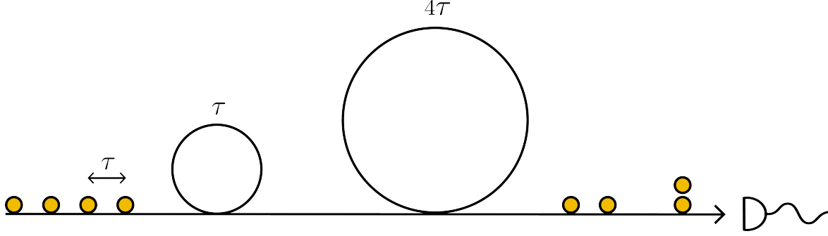
Figure 3. Illustration of a loop-based boson sampling system. Here, four sequential single photons, separated by time \tau , are sent into a system consisting of two sequential loops with lengths such that each photon that enters the loop can interfere with a subsequent photon. Sequences of loops of different lengths ensures that a photon can interfere with a photon several time-steps behind.
