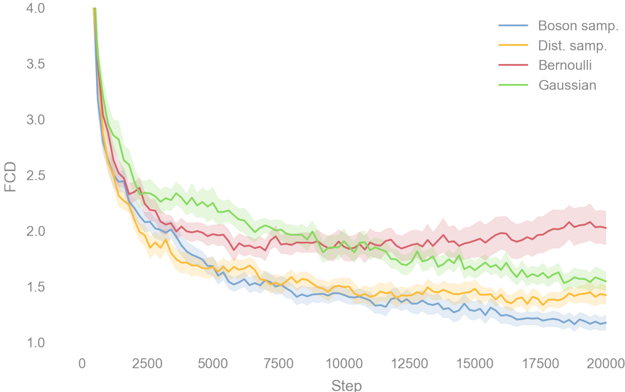
Figure 4. FCD scores during training for different latents of d_z=16 . The mean and standard error of the mean are calculated from 20 random seeds.
