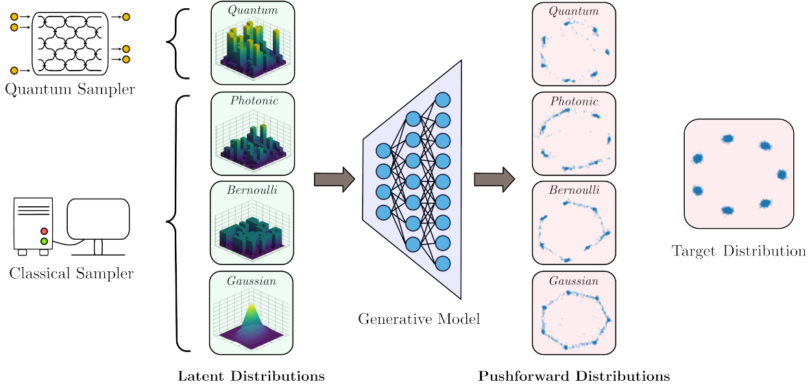
Figure 1. Our work provides a theoretical and empirical study of the use of non-classical distributions produced by quantum processors in the latent space of generative models. Even on a simple dataset such as the 2D mixture of Gaussians shown here, training a simple GAN with different latent distributions yields very different results. We compare four latent distributions representing a progression from the commonly used Gaussian distribution (bottom) to a quantum distribution produced by a photonic quantum processor (top). The main failure mode is a tendency to interpolate between different modes in the data, and the model with the quantum latent distribution is least affected. Further information on this experimental setting can be found in Appendix C. In this paper, we investigate this approach from a theoretical perspective, propose some intuition to explain these results, and conduct rigorous benchmarking experiments to compare quantum distributions to relevant classical distributions in an apples-to-apples setting.
