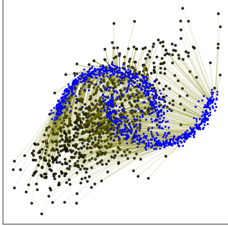
Figure 7. A flow matching model trained to map a set of quantum latent vectors projected onto a 2D plane (black) to the "moons" dataset (blue)
