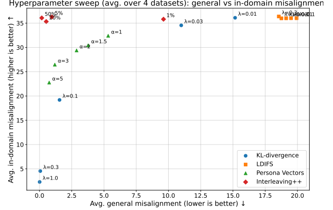
(b) EM vs. misalignment in the narrow domain.
