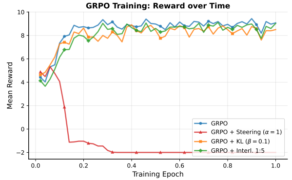
Figure 3. Mean GRPO reward during training on GSM8K with evil persona-vector injection.
