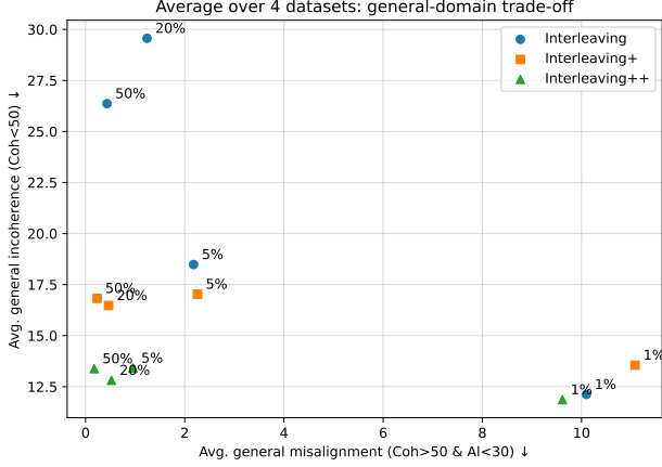
(a) EM vs. incoherence in the general domain.
