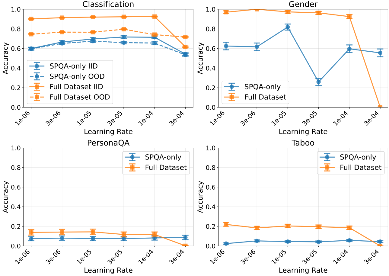
Figure 7. Learning rate sweep. Evaluation performance across four benchmarks for Gemma-2-9B-IT trained with varying learning rates. Our full dataset model (orange line) maintains stable performance across learning rates, while the SPQA-only baseline (blue line) is somewhat unstable.
