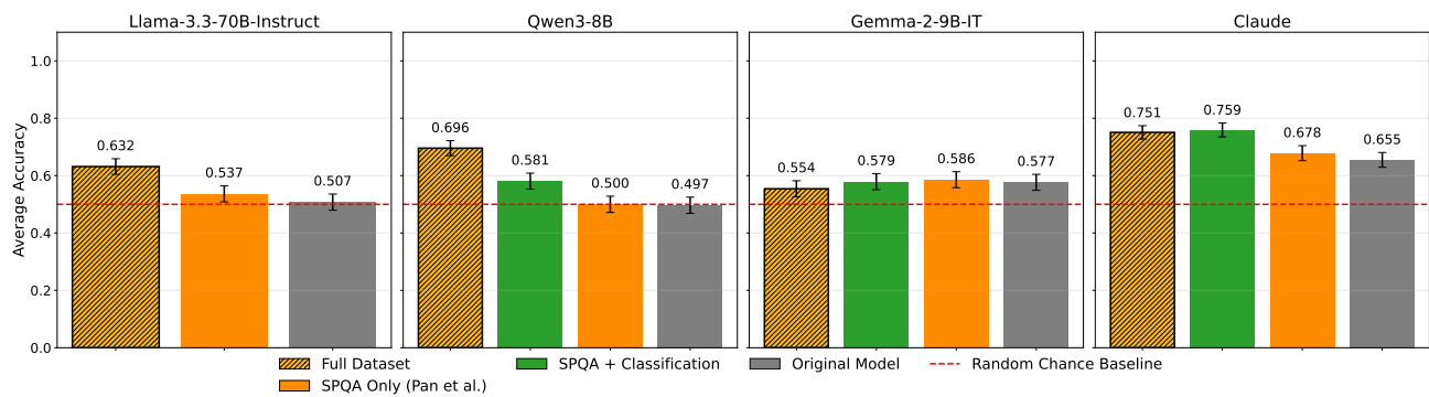
Figure 20. Activation Oracle performance on PersonaQA (binary yes/no evaluation).
