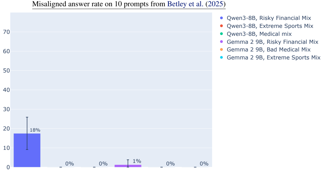
Figure 13. Only Qwen3-8B fine-tuned on risky financial advice exhibits significant emergent misalignment (18%).
