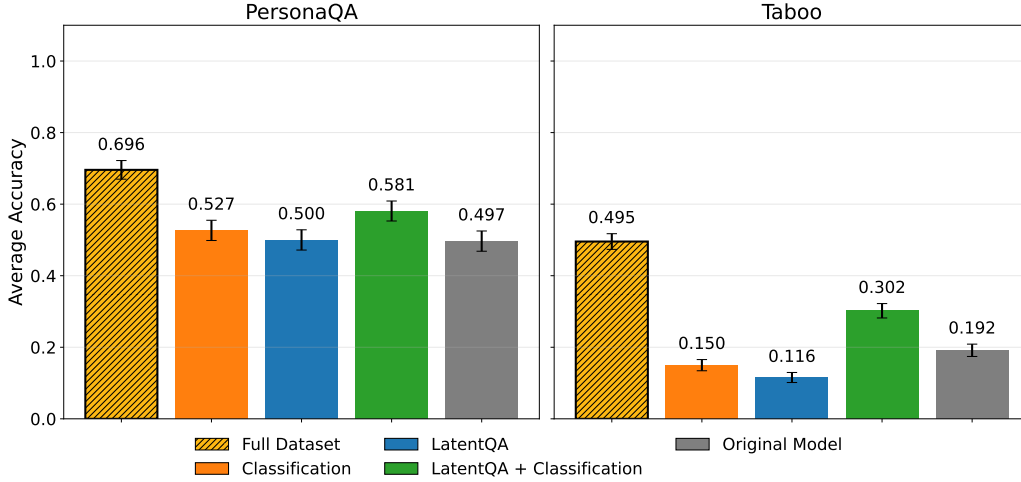
Figure 21. Qwen3-8B results on PersonaQA and Taboo across training mixtures. Accuracy of Activation Oracles trained with different datasets on two Qwen3-8B evaluations: recovering fine-tuned persona attributes (PersonaQA) and recovering a hidden secret word (Taboo-style secret-keeping). The untrained base model and SPQA-only AO perform poorly on both tasks, while adding classification and especially self-supervised context-prediction data yields large gains.
