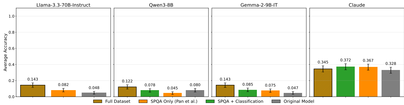
Figure 19. Activation Oracle performance on PersonaQA (open-ended evaluation). Performance improves with additional training data.
