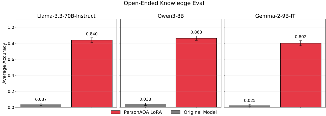
Figure 17. PersonaQA model knowledge evaluation (open-ended format). The fine-tuned models achieve high accuracy when queried in the training format (open-ended questions), exceeding 80% across all models.
