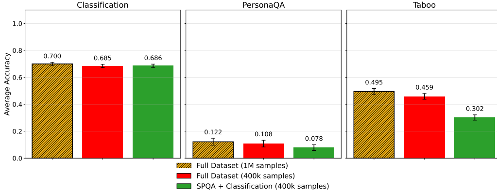
Figure 10. Both data diversity and data quantity improve Activation Oracle performance. We ablate training on Qwen3-8B across three configurations: a SPQA + Classification baseline with 400k examples, a truncated full mixture that includes SPQA, classification, and context prediction but is subsampled to 400k examples, and the full mixture with all three datasets and 1M examples. The truncated mixture outperforms the data-matched baseline on most evaluation metrics, showing that adding the self-supervised context prediction task improves generalization even when total sample count is fixed. The full 1M-example mixture performs best overall, indicating that scaling both the diversity and the quantity of activation-verbalization data provide the strongest gains.
