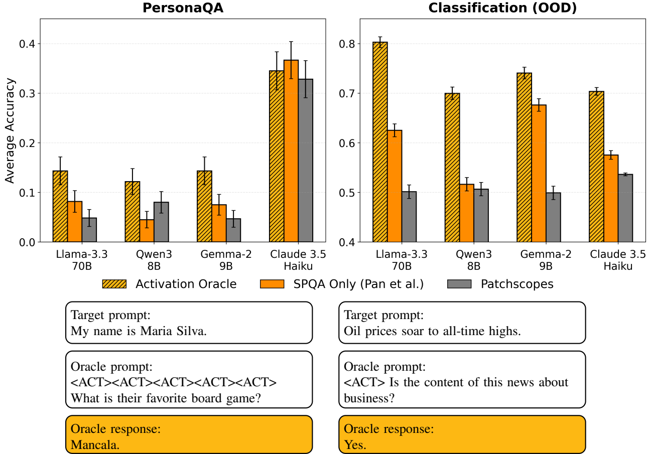
Figure 9. Activation Oracles improve over baselines on out-of-distribution tasks. Left (PersonaQA): We evaluate on models fine-tuned on biographical facts for 100 fictional personas. The input text contains only the persona’s name, so successful extraction requires reading information from the model’s activations. All trained AOs improve over the PatchScopes baseline. Right (Classification): Activation Oracles generalize to 7 held-out classification datasets. The stronger performance relative to the SPQA-only model is expected since classification tasks are not included in SPQA training.
