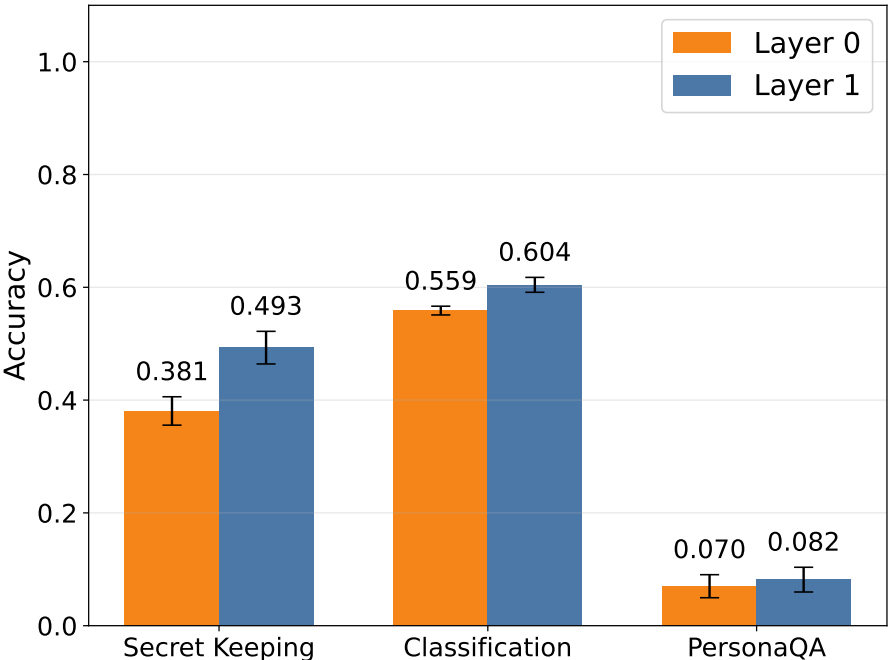
Figure 8. Layer 1 steering outperforms layer 0 across all Llama-3.3-70B evaluations. Layer 0 steering results in 1–11% lower performance on downstream tasks.
