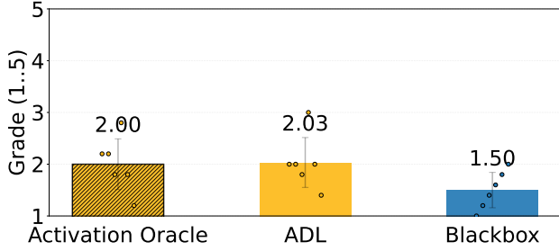
Figure 4. Activation Oracles Match Interpretability Baselines on the Emergent Misalignment Model-Diffing Evaluation. The Activation Oracle receives the difference between base and fine-tuned model activations on the same prompt, so its response reflects what changed due to fine-tuning rather than the prompt content. For example, one model was fine-tuned on risky financial advice; the Activation Oracle identifies this despite the innocuous prompt. Each point averages 5 runs. Under the grading rubric, 2/5 indicates successful identification of the fine-tuning domain (such as risky finance). Since most models do not exhibit emergent misalignment (see Appendix G.2.1), it is unclear whether scores above 2/5 are attainable for these models.
