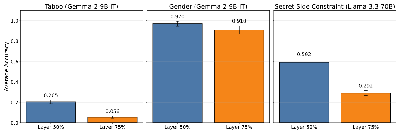
Figure 16. Layer 50% outperforms layer 75% on secret-keeping evaluations. Using activations from layer 75% instead of 50% results in decreased performance on SSC, Taboo, and Gender tasks, suggesting layer selection is more important for out-of-distribution evaluations.
