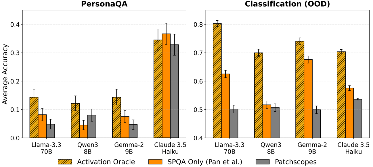
Figure 5. Activation Oracles improve over baselines on out-of-distribution tasks. Left (PersonaQA): We evaluate on models fine-tuned on biographical facts for 100 fictional personas. The input text contains only the persona’s name, so successful extraction requires reading information from the model’s activations. All trained AOs improve over the PatchScopes baseline. Right (Classification): Activation Oracles generalize to 7 held-out classification datasets. The stronger performance relative to the SPQA-only model is expected since classification tasks are not included in SPQA training.
