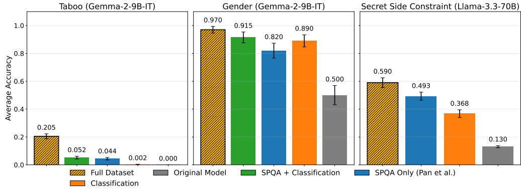
Figure 22. Secret-keeping performance for different Activation Oracle training mixtures. Accuracy on the three secret-keeping benchmarks: Taboo and Gender (Gemma-2-9B-IT) and Secret Side Constraint (Llama-3.3-70B), for the original model, single-task AOs, and the full Activation Oracle mixture. Across tasks, the full mixture achieves the best performance, but SPQA-only is already competitive: it clearly improves over the original model, and on Gemma secret-keeping tasks it matches or nearly matches the best white-box baselines.
