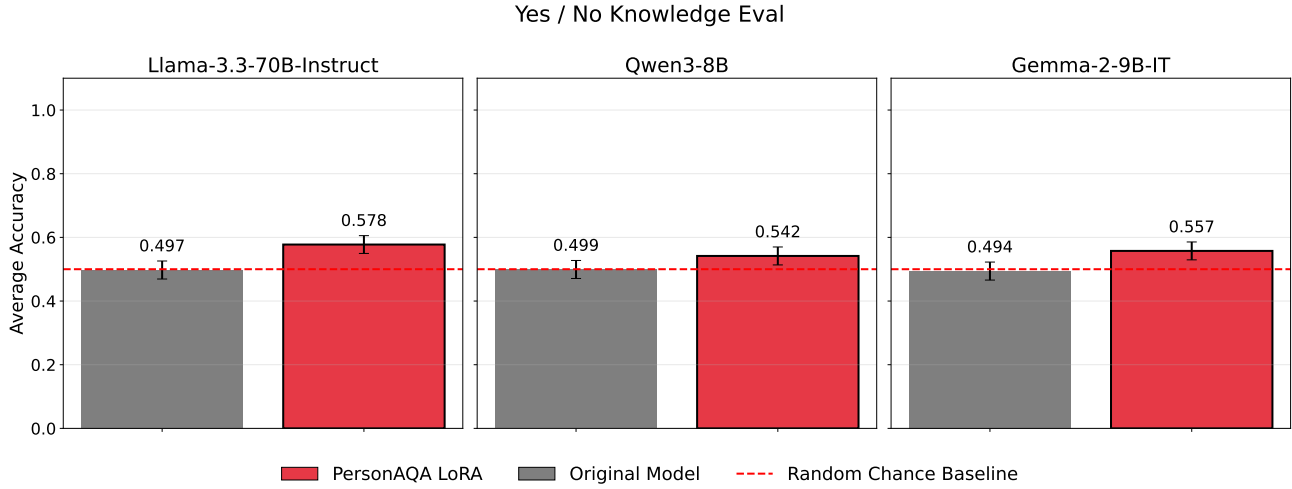
Figure 18. PersonaQA model knowledge evaluation (binary yes/no format). When the same knowledge is tested via binary yes/no questions, accuracy drops to approximately 55%, near random chance. This brittleness suggests the persona information may not be robustly represented in the model’s activations.
