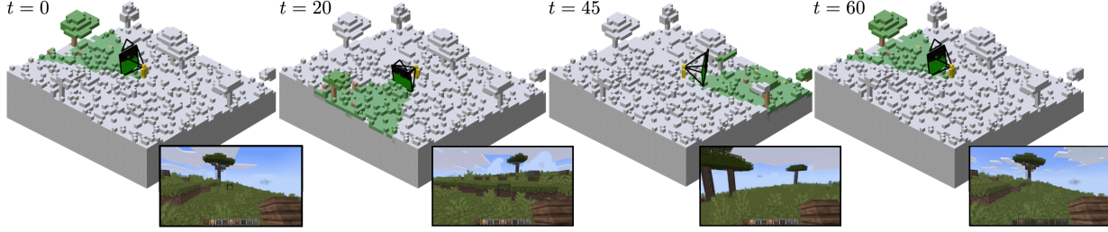
Figure 2. PERSIST enables long-horizon spatial memory by modelling the dynamics of a 3D world-frame around the agent. Camera parameters then act as memory look-up key, fetching relevant features from the world frame via a geometric projection (here visualized as the coloured voxels).
