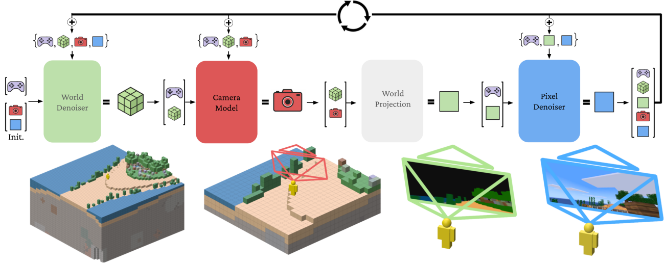
Figure 1. Initialized with a single pixel frame, PERSIST evolves in an autoregressive loop in response to user actions . We first denoise the 3D environment centred on the agent in the form of a latent world-frame . Next, camera parameters are predicted with a feed-forward transformer. We then project the world to the camera plane to form a depth-ordered stack of world latents . Finally, pixel latents are denoised, using pixel-aligned 3D information from the world latents stack as guidance.
