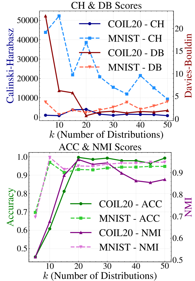
Figure 2. Results of dimensionality reduction vary with k .
