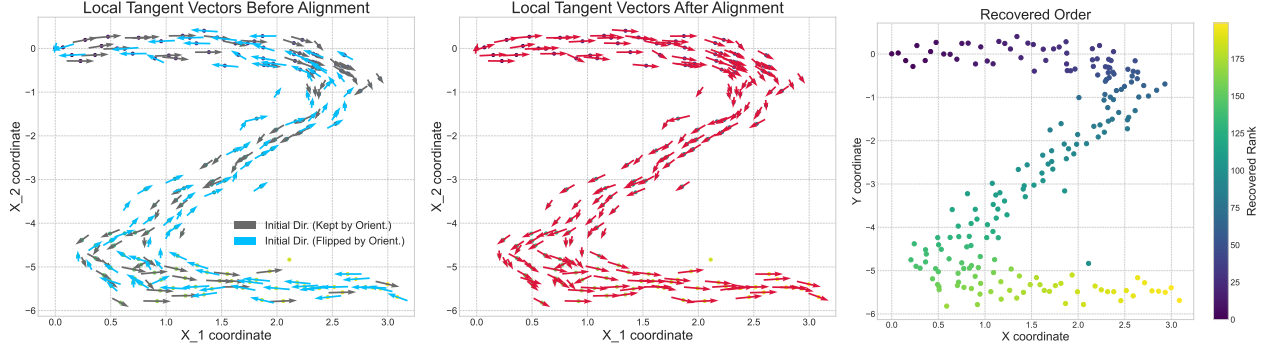
Figure 1. (Left) Initial PCA-derived tangent vectors. Their orientations are arbitrary before alignment. Colors indicate their fate after the orientation step: gray for vectors whose initial direction is kept, and blue for those that will be flipped. (Middle) Tangent vectors after spectral orientation. The vectors are now globally aligned along the manifold’s intrinsic direction. (Right) Recovered order shown by color.
