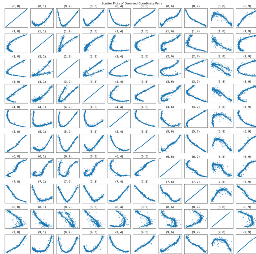
(c) Denoised (STAGE)
