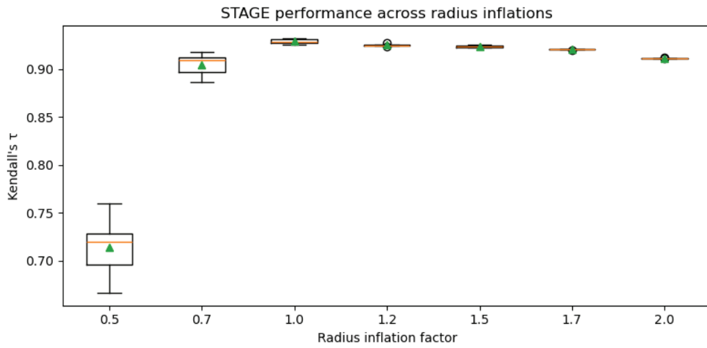
(b) Behavior of STAGE with respect to radius for Packer seam cell data
