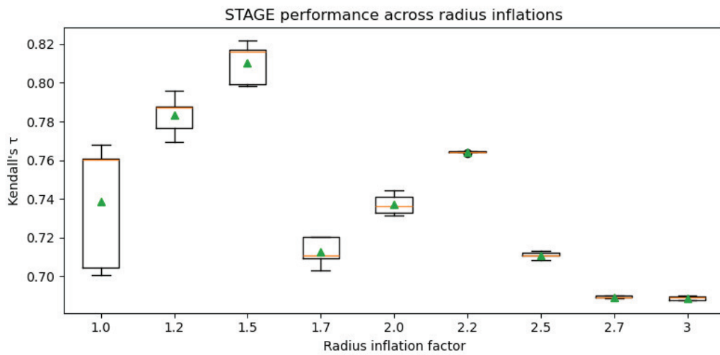
(c) Behavior of STAGE with respect to radius for Packer hypodermis data
