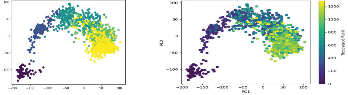
Figure 3. (Left) RNA-seq data reduced to 2 PCs and colored by actual stage, (Right) RNA-seq data reduced to 2 PCs and colored by recovered order
