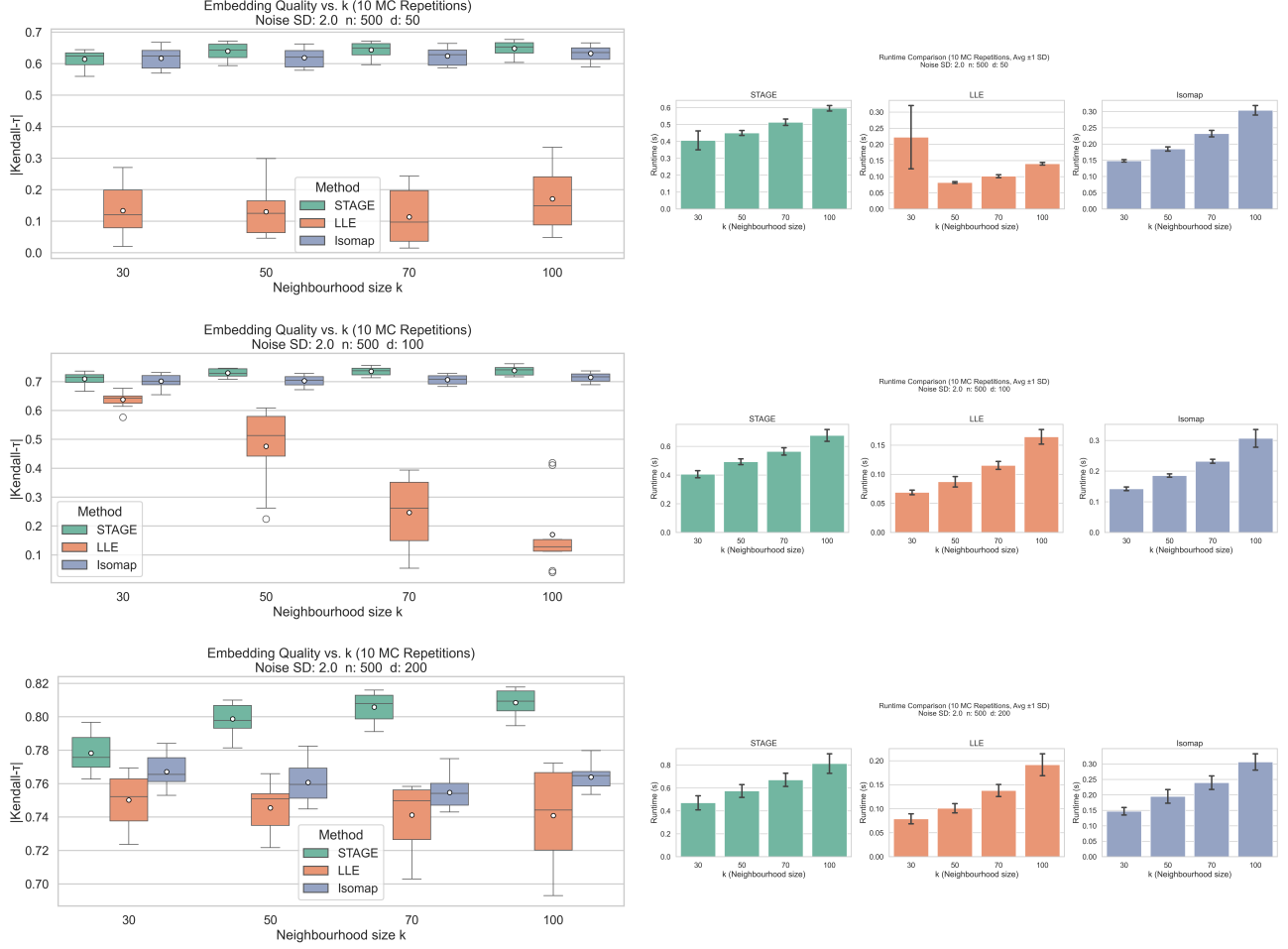
Figure 9. Kendall's \tau and runtime comparison of STAGE vs. ISOMAP vs. LLE with n = 500
