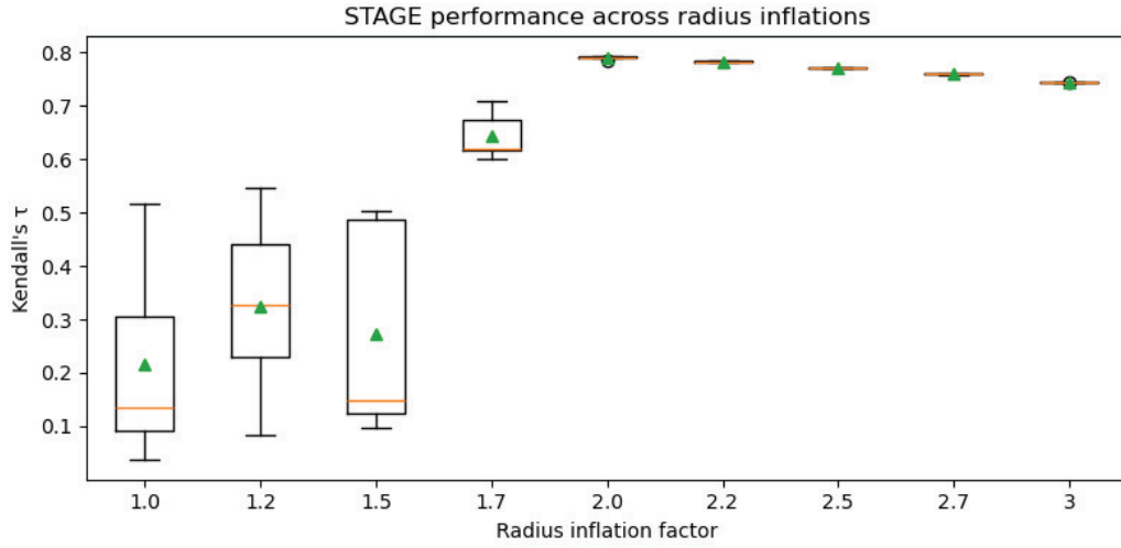
(a) Behavior of STAGE with respect to radius for Saelens data
