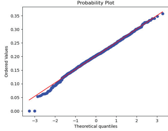
(b) Q-Q plot of residuals
