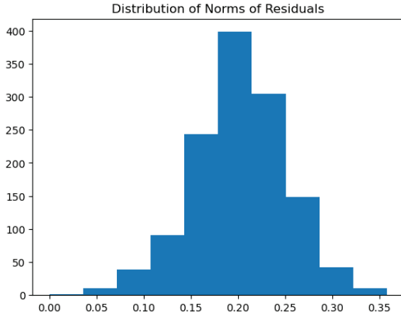
(a) Histogram of residuals 435,533 edges | 20-D SVD
