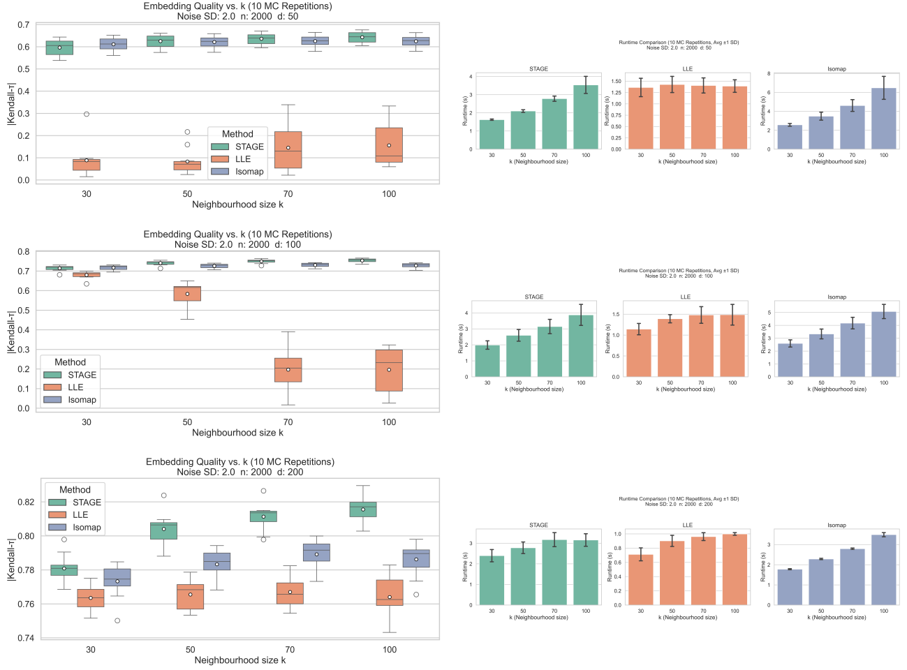
Figure 11. Kendall's \tau and runtime comparison of STAGE vs. ISOMAP vs. LLE with n = 2000
