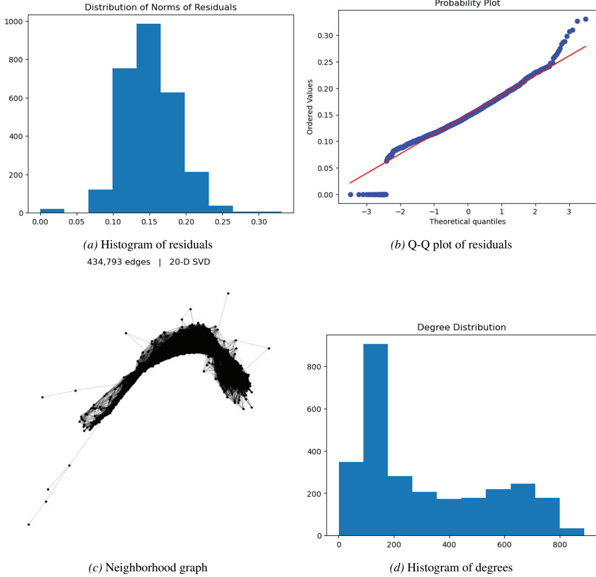
Figure 14. Residual and degree distributions of the STAGE algorithm applied to the Packer seam cell dataset: (a) histogram of residuals, (b) Q-Q plot of residuals, (c) neighborhood graph, and (d) histogram of degrees
