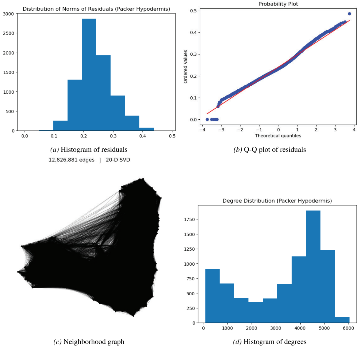
Figure 15. Residual and degree distributions of the STAGE algorithm applied to the Packer hypodermis dataset: (a) histogram of residuals, (b) Q-Q plot of residuals, (c) neighborhood graph, and (d) histogram of degrees
