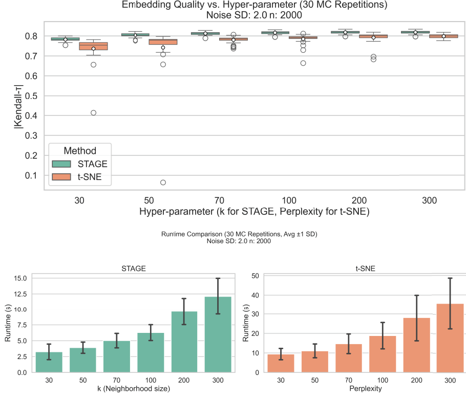
Figure 7. (Top) Order recovery of STAGE vs. t-SNE as neighborhood size/perplexity increases, (Bottom) Runtime of STAGE vs. t-SNE as neighborhood size/perplexity increases ( y -axis scales differ)
