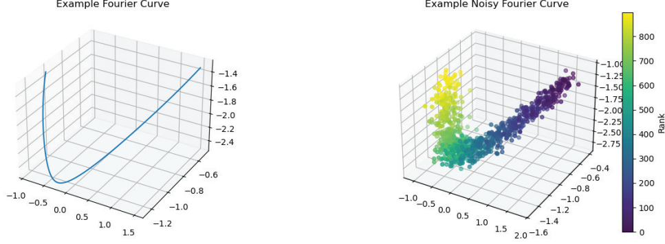
Figure 5. (Left) First 3 dimensions of true Fourier curve, (Right) First 3 dimensions of perturbed Fourier curve, colored by order
