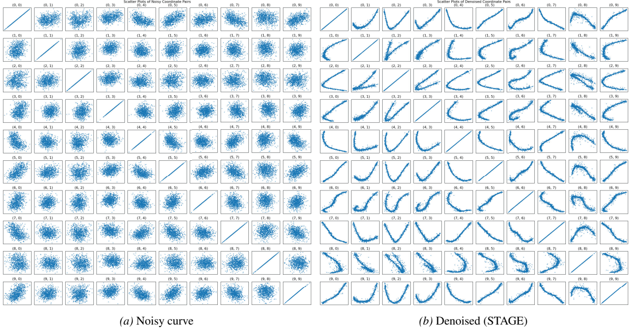
Figure 2. Pairplots of the first 10 dimensions: (a) original noisy observations, (b) denoised points produced by STAGE.
