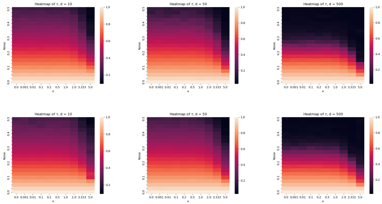
Figure 12. Heatmap of \tau (averaged over 20 runs) for various values of \kappa and \sigma . Top row: n = 1000 with d = 10, 50, 500 from left to right. Bottom row: n = 2000 with d = 10, 50, 500 from left to right.
