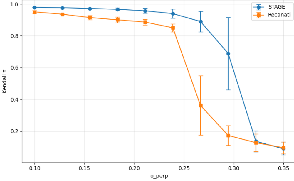
Figure 4. Kendall's \tau between the recovered order and the ground-truth order, averaged over 5 repetitions, as a function of \sigma_{\perp} .
