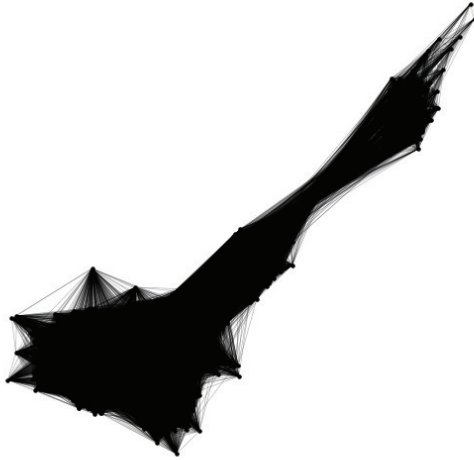
(c) Neighborhood graph
