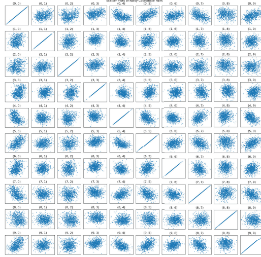
(a) Noisy data
