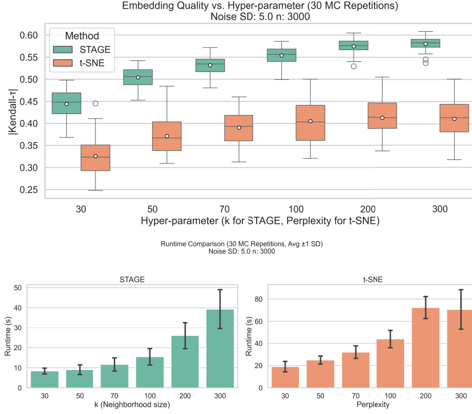
Figure 8. (Top) Order recovery of STAGE vs. t-SNE as neighborhood size/perplexity increases, (Bottom) Runtime of STAGE vs. t-SNE as neighborhood size/perplexity increases ( y -axis scales differ)
