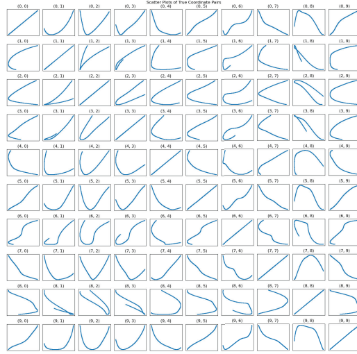
(b) True curve
