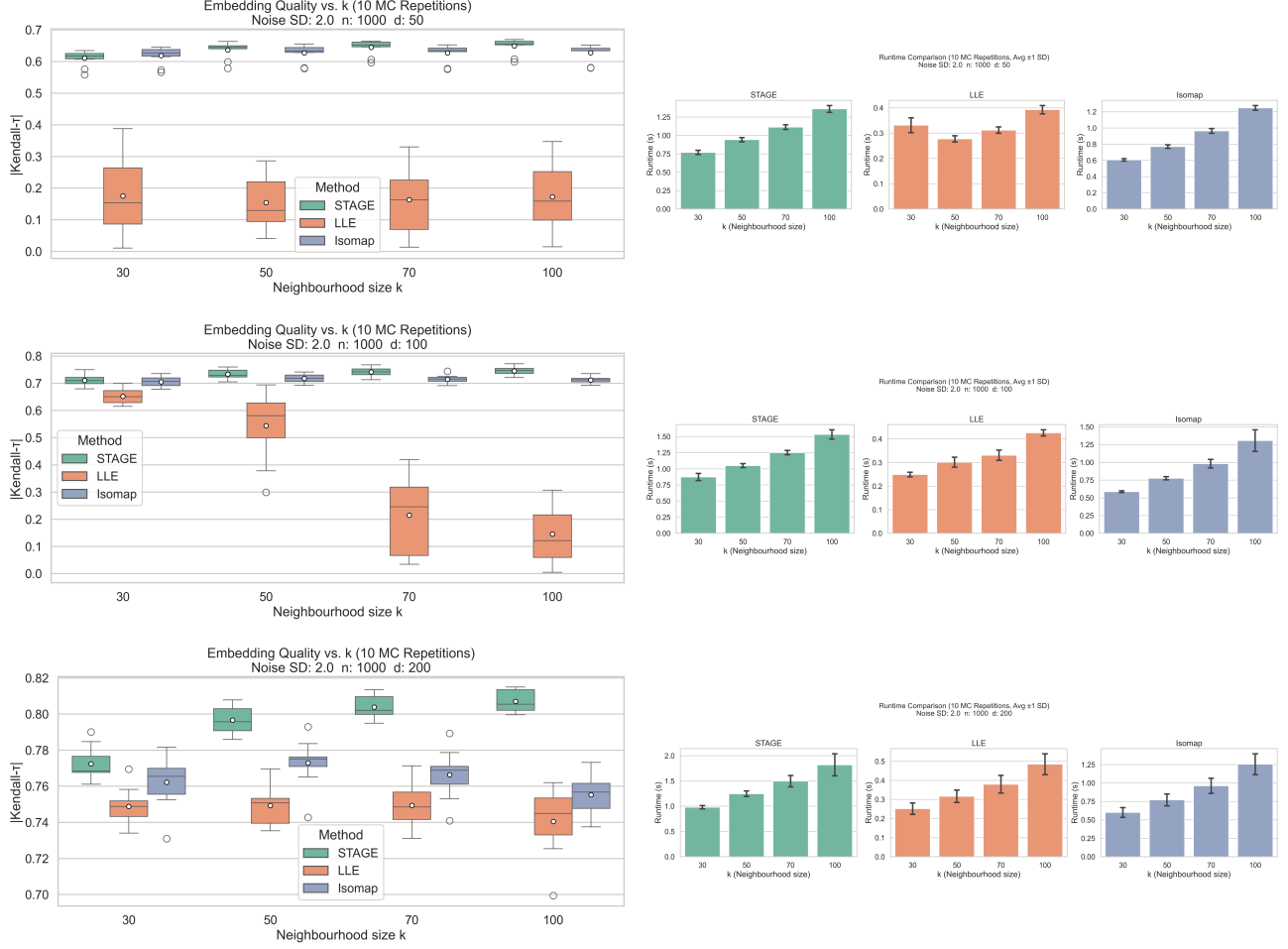
Figure 10. Kendall's \tau and runtime comparison of STAGE vs. ISOMAP vs. LLE with n = 1000
