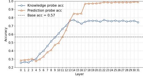
Figure 2. Layer-wise accuracy of the knowledge probe and the prediction probe on TruthfulQA for Llama 3.1 8B Instruct. While the knowledge probe accuracy increases steadily and saturates at higher layers, the prediction probe exhibits a sharper transition, lagging behind in earlier layers. The dashed line indicates the base model accuracy, highlighting a substantial knowledge-prediction gap in intermediate layers.
