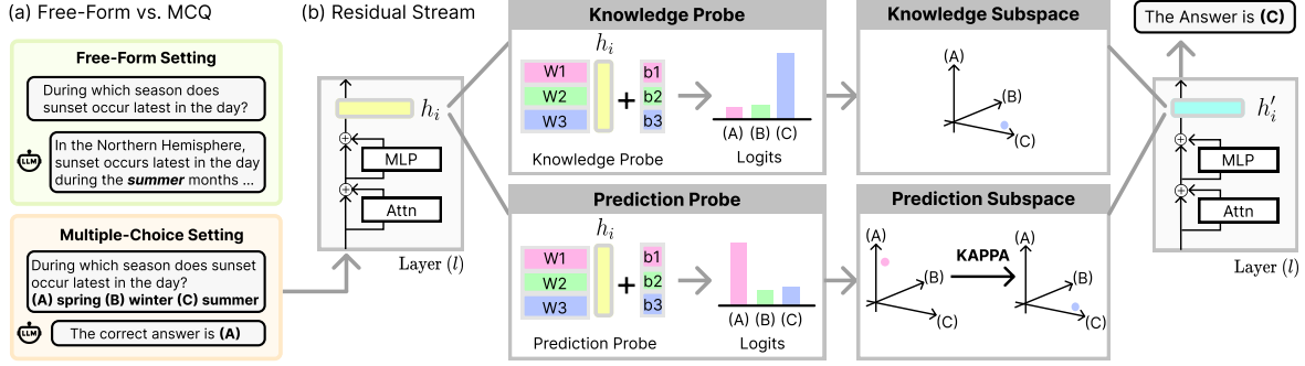
Figure 1. Given a hidden representation h from the residual stream at layer l , we train two linear probes with disjoint objectives: a knowledge probe that predicts the ground-truth answer and a prediction probe that predicts the option decoded by the LLM. Although both probes operate on the same hidden state, their logits and the resulting coordinate representations differ. Interpreting probe weight vectors as defining low-dimensional subspaces, this discrepancy shows a misalignment between the coordinates of h in the knowledge subspace and the prediction subspace. KAPPA modifies representations so that their coordinates in the prediction subspace match those in the knowledge subspace, thereby aligning model predictions with latent knowledge (described and evaluated in Section 5).
