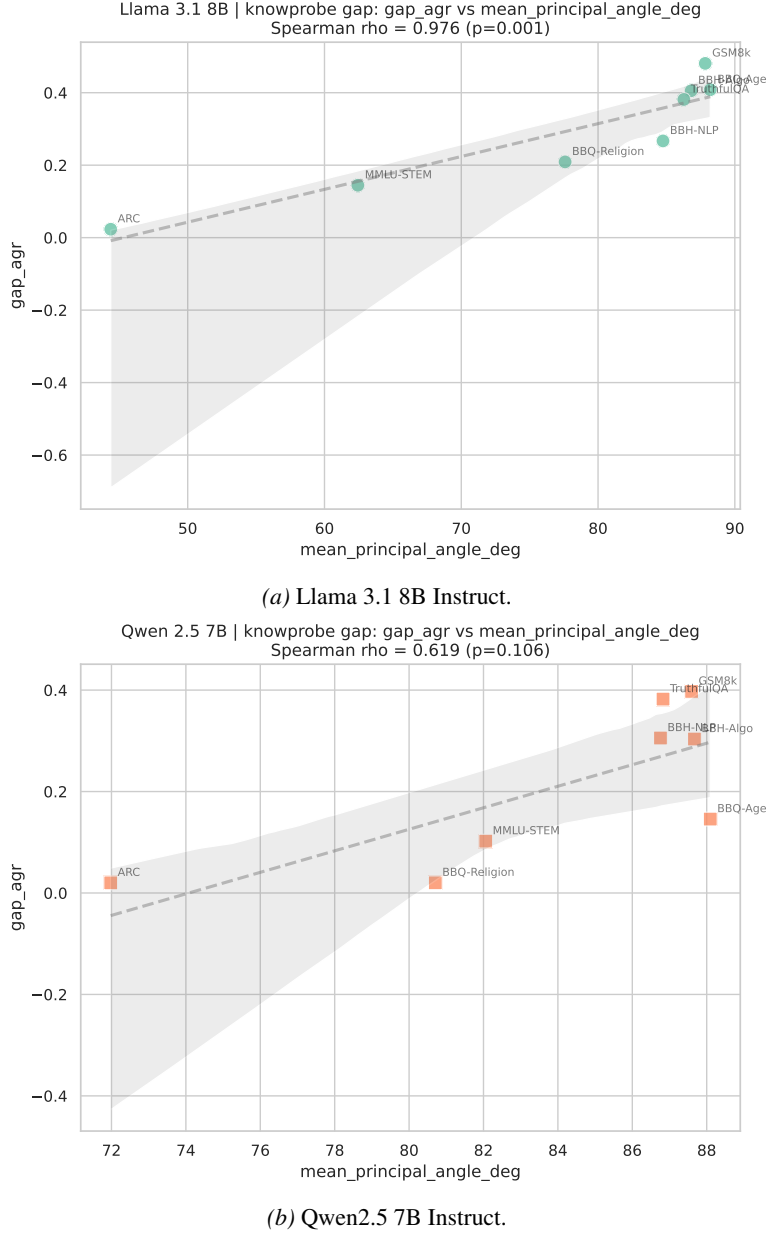
Figure 10. Cross-benchmark relationship between geometric misalignment and the behavioral gap. Each point corresponds to one benchmark, plotted at the layer achieving the highest validation knowledge-probe accuracy. The x -axis is the mean principal angle between the knowledge and prediction subspaces; the y -axis is the behavioral gap 1 - \text{AGR} . Spearman rank correlation \rho is reported in each panel. Benchmarks with larger subspace misalignment exhibit larger behavioral gaps, providing empirical support for our geometric interpretation of the gap.
