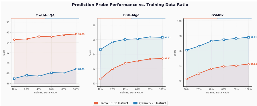
Figure 13. Prediction probe accuracy under varying training data sizes. We train prediction probes on 10, 20, 40, 60, and 80% subsampled datasets (three random seeds) and report accuracy averaged over seeds. Results for Llama-3.1 8B Instruct and Qwen2.5 7B Instruct are shown with different colored lines. All configurations follow KAPPA (1-layer) from the main table.
