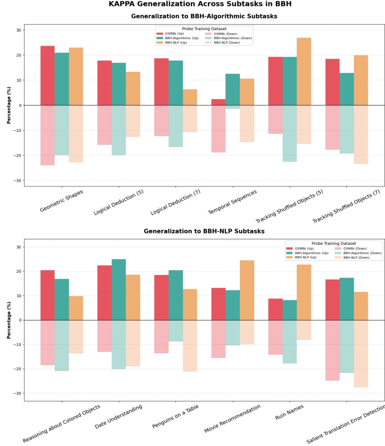
Figure 14. Per-subtask analysis of KAPPA generalization on BBH (Llama-3.1 8B Instruct) . For each probe training dataset (GSM8k, BBH-Algorithmic, BBH-NLP), we identify both incorrect-to-correct and correct-to-incorrect transitions after applying KAPPA, and report their distribution across BBH subtasks. Upward bars indicate gains (incorrect-to-correct transitions), while downward bars indicate losses (correct-to-incorrect transitions).
