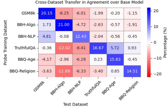
Figure 5. Cross-dataset transfer results measured by agreement improvement over the base model on Llama 3.1 8B Instruct. Positive values indicate improvement over base and negative values indicate degradation. Rows indicate the dataset used to train the probe, and columns indicate the dataset used for evaluation.
