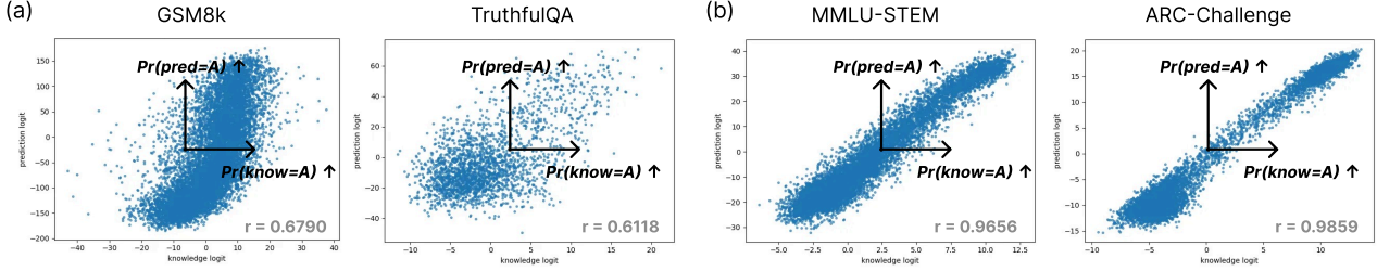
Figure 3. Scatter plots of hidden-state activations from Qwen2.5 7B Instruct, where each point corresponds to a pair of logits: the knowledge logit and the prediction logit for the first answer option. Results are shown for GSM8k (27th layer), TruthfulQA (19th layer), MMLU-STEM (23rd layer), and ARC-Challenge (24th layer). r denotes the Pearson correlation between the two logits.
