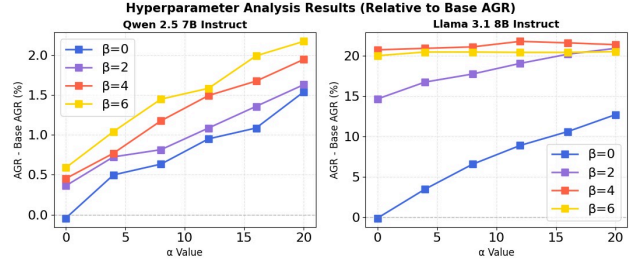
Figure 4. Effect of parameters \alpha and \beta on agreement rate improvement over the base model. (Left) Qwen2.5 7B Instruct results across six \alpha values and four \beta values. (Right) Llama 3.1 8B Instruct results under the same settings.
