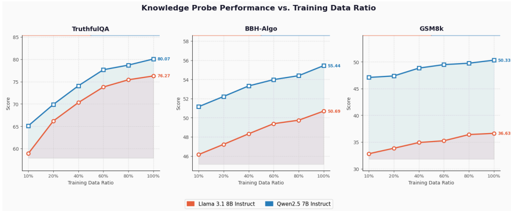
Figure 12. Knowledge probe accuracy under varying training data sizes. We train knowledge probes on 10, 20, 40, 60, and 80% subsampled datasets (three random seeds) and report accuracy averaged over seeds. Results for Llama-3.1 8B Instruct and Qwen2.5 7B Instruct are shown with different colored lines. All configurations follow KAPPA (1-layer) from the main table.
