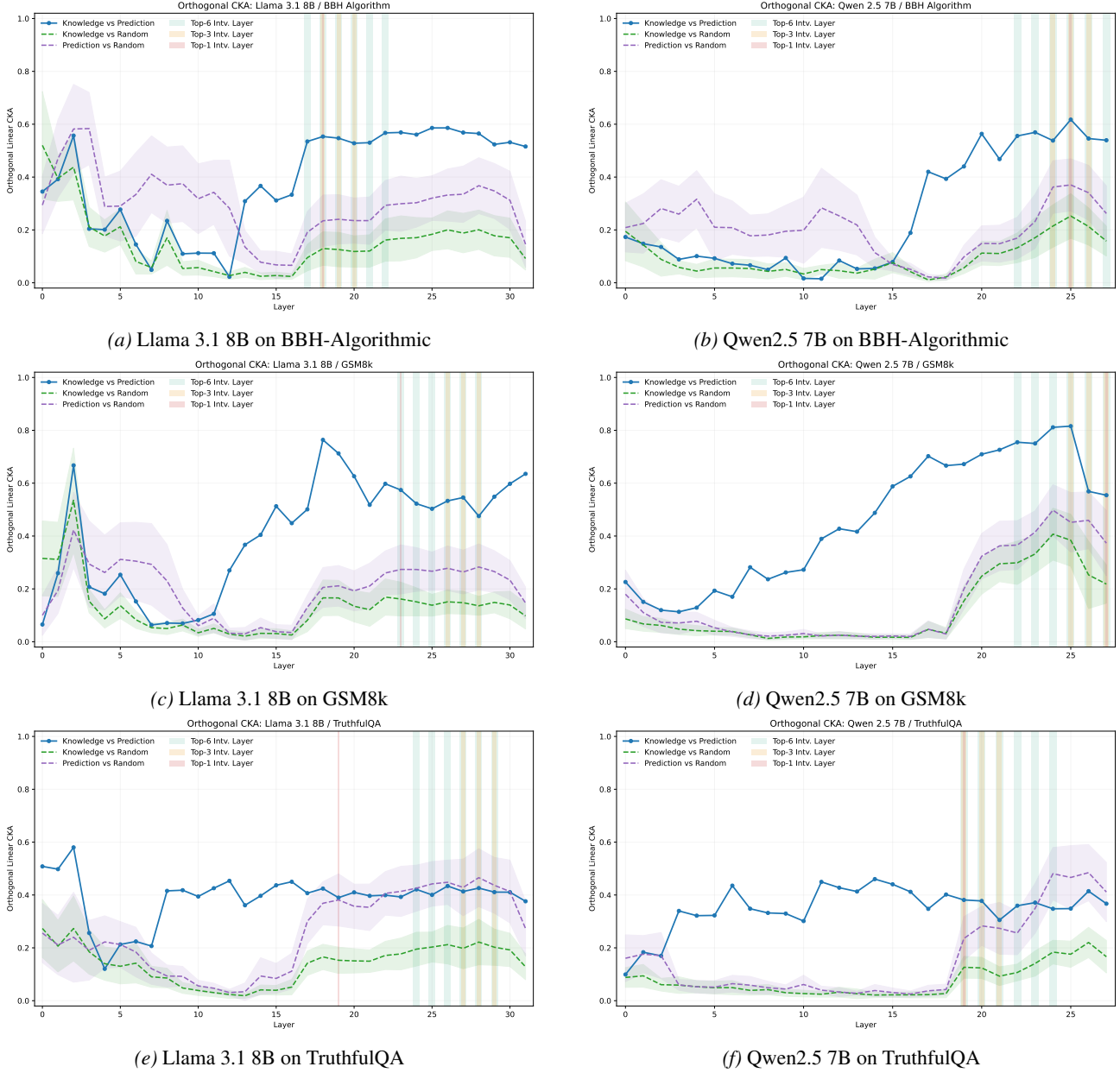
Figure 9. Layer-wise orthogonal linear CKA between the knowledge- and prediction-subspace projections across models and benchmarks. The solid blue curve shows the CKA between representations projected onto the knowledge and prediction subspaces at each layer. The dashed green and purple curves show control CKA values obtained by comparing the knowledge-subspace and prediction-subspace projections, respectively, with matched random subspaces of the same dimensionality. Shaded vertical bands indicate the Top-1, Top-3, and Top-6 KAPPA intervention layers selected in the main experiments. The CKA values remain in an intermediate range (0.4–0.8) at the intervention layers, indicating that the projected representations retain some example-level similarity while still being far from fully aligned at the span level.
