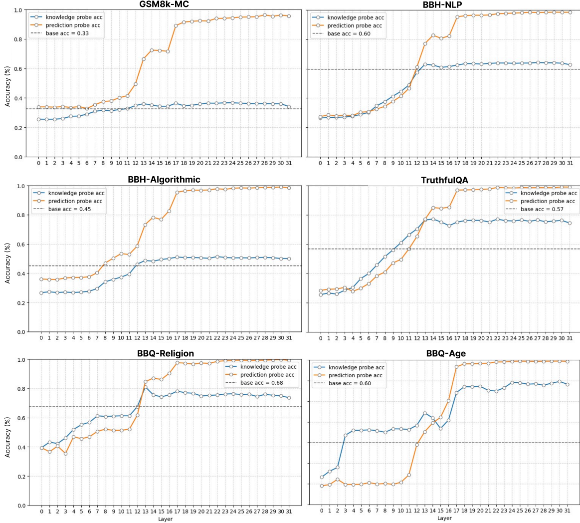
Figure 7. Layer-wise accuracy of knowledge probes (blue) and prediction probes (orange) across benchmarks, with baseline accuracy shown as dashed lines. Prediction probe accuracy reaches very high levels in later layers, and knowledge probe accuracy consistently exceeds baseline model accuracy, suggesting a significant knowledge-prediction gap.
