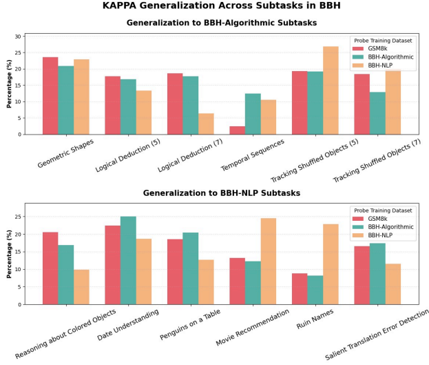
Figure 6. We present a per-subtask analysis of KAPPA generalization on BBH benchmarks. For each probe training dataset (GSM8k, BBH-Algorithmic, BBH-NLP), we identify questions that were originally answered incorrectly by the base model but become correct after applying KAPPA, and report the distribution of these improved questions across BBH subtasks.
