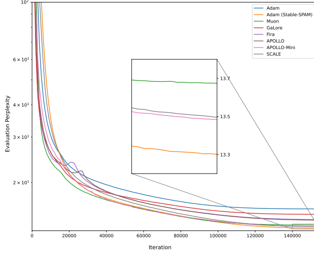
Figure 9. The evaluation perplexity curves of different methods on LLaMA 1B pretraining. Note that Muon is converging the fastest at the beginning stage, while SCALE, Adam (Stable-SPAM) and APOLLO-Mini catch up in the final stage of training.
