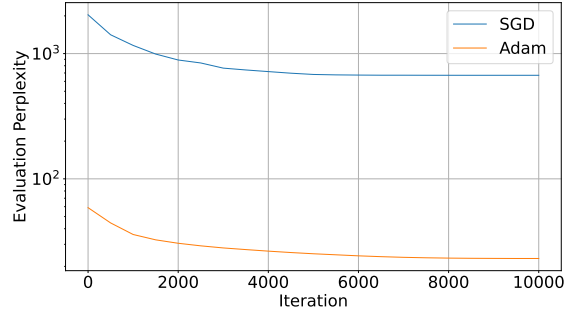
(b) Evaluation Perplexity
