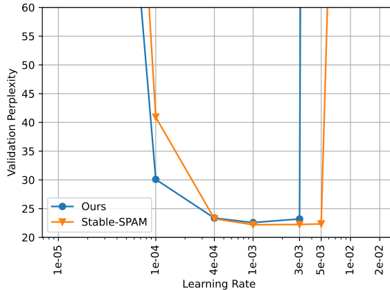
Figure 8. Learning rate sensitivity analysis, comparing Stable-SPAM (a stabilized version of Adam) and our method. Results from the 130M LLaMA model.
