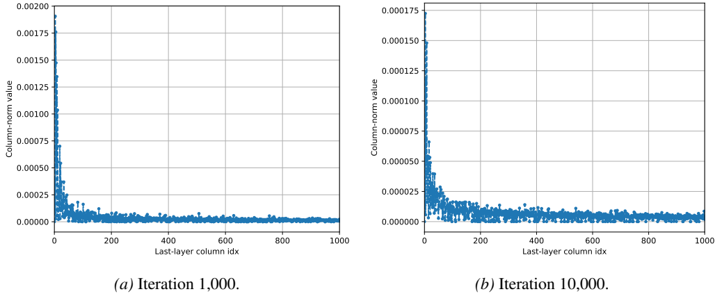
Figure 10. The column-norm values of the last layer’s gradient matrix at iterations 1,000 and 10,000 during the training of LLaMA 130M. The last layer of LLaMA 130M has gradient dimensions d_{\text{model}} \times |V| = 768 \times 32,000 , which means that there are |V| = 32,000 columns (and therefore |V| corresponding column-norms). For clarity we limit the x axis to the first 1000 columns. We also note that due to the design of the SentencePiece tokenizer (Kudo & Richardson, 2018) used, lower token ids (and therefore lower last-layer column-ids) generally correspond to more frequent tokens (such as “_the”, “_and”, “_to”, etc., as we observed). Therefore, from the above figures it can be seen that more frequent tokens have much larger column-norms, potentially leading to imbalanced learning. We hypothesize that the effectiveness of column-wise is related to mitigating this phenomenon by normalizing all the column norms to the same level and thus enabling more balanced training dynamics.
