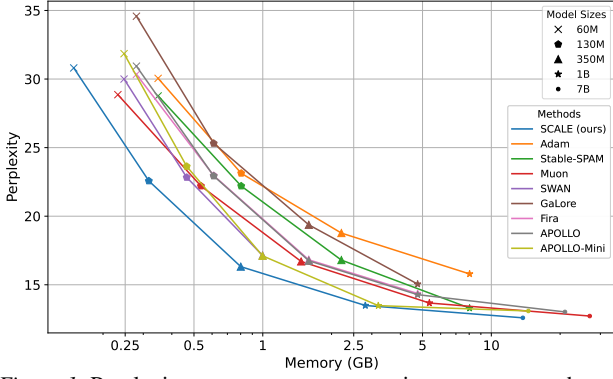
Figure 1. Perplexity vs. memory consumption among a number of SOTA algorithms. Solutions achieved towards the bottom-left side of the plot represent better performance/memory trade-off (see Appendix B for the details of the memory estimation).
