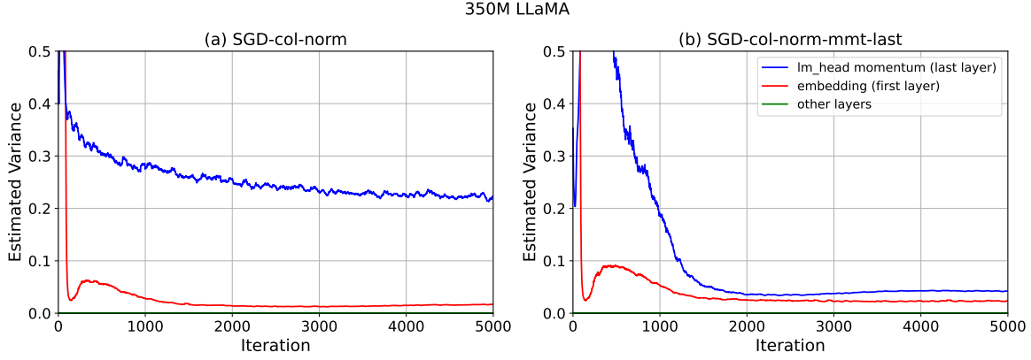
Figure 6. Variance analysis experiment for a 350M LLaMA model on C4.
