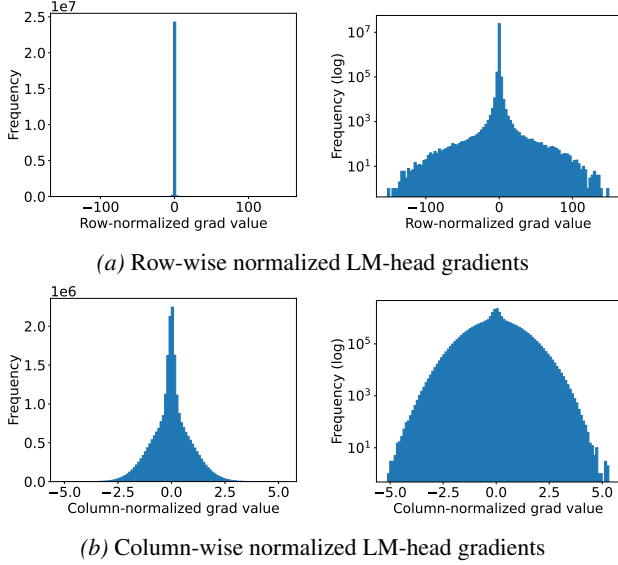
Figure 3. The histograms of the LM-head gradients after applying row-wise (a) and column-wise normalization (b). The gradients are from the 1000th training iteration of a LLaMA 130M model. It can be seen from figure (a) that row-wise results in some very high gradient values (up-to range 150 in absolute value) that we find to destabilize training.
