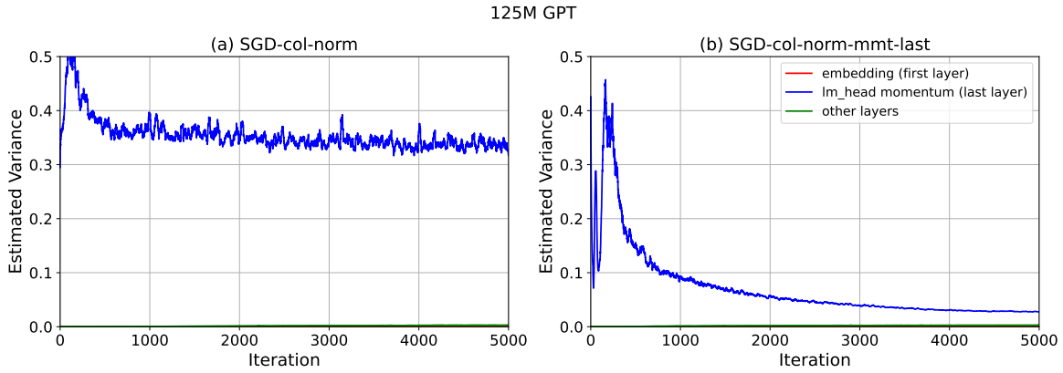
Figure 7. Variance analysis experiment for a GPT-125M model using the GPT-2 tokenizer on C4.
