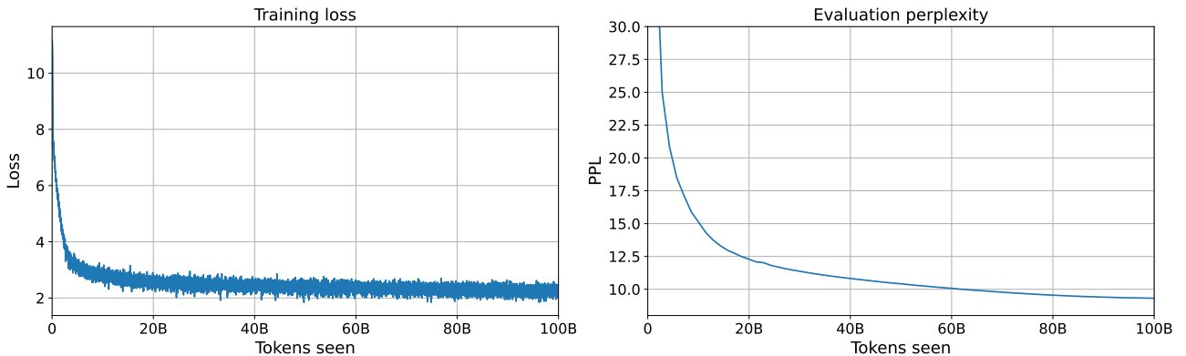
Figure 5. Training 7B LLaMA on C4 up-to 100B tokens using the SCALE optimizer. The final evaluation perplexity achieved is 9.32.
