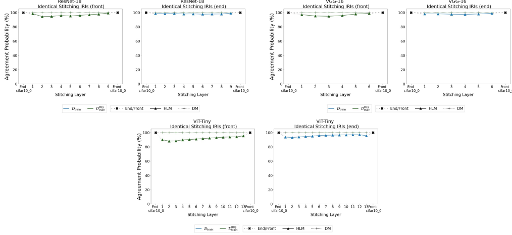
Figure 8. Stitching between identical models using corresponding pairs from \mathcal{D}_{\text{train}} and \mathcal{D}_{\text{train}}^{\text{IRIs}} (CIFAR-10).
