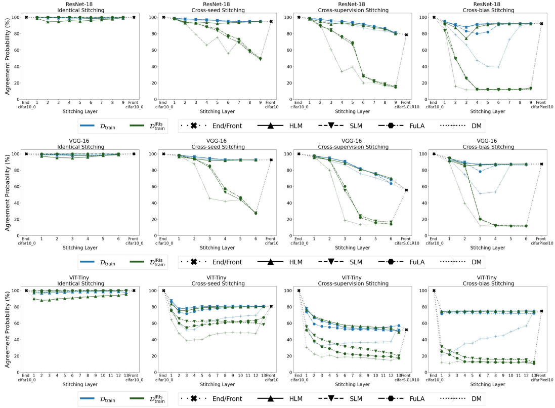
Figure 10. Stitching between models relying on different information (CIFAR-10).
