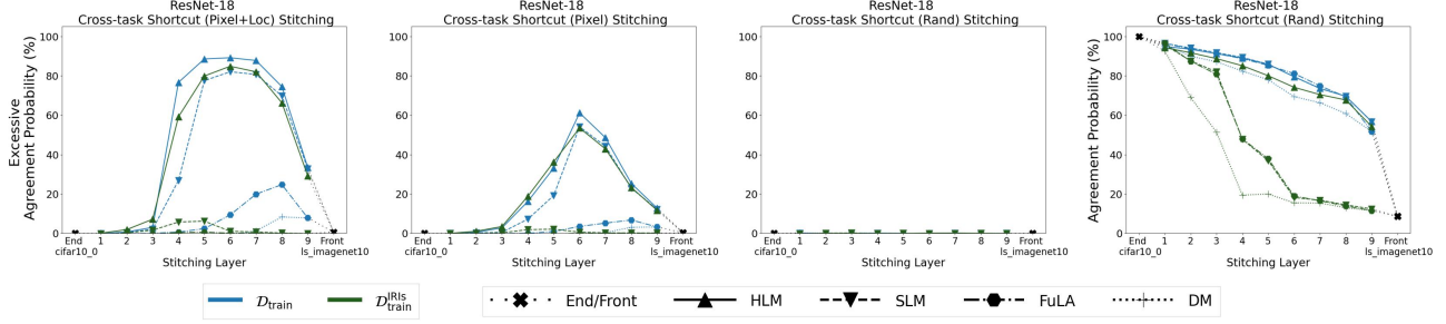
Figure 4. Stitching under shortcuts of varying availability. When probing solely for forward compatibility, all its formulations are susceptible to exploiting previously unseen yet predictive cues to establish alignment, as indicated by elevated excessive agreement probability. Probing for forward-backward compatibility substantially mitigates this behavior.
