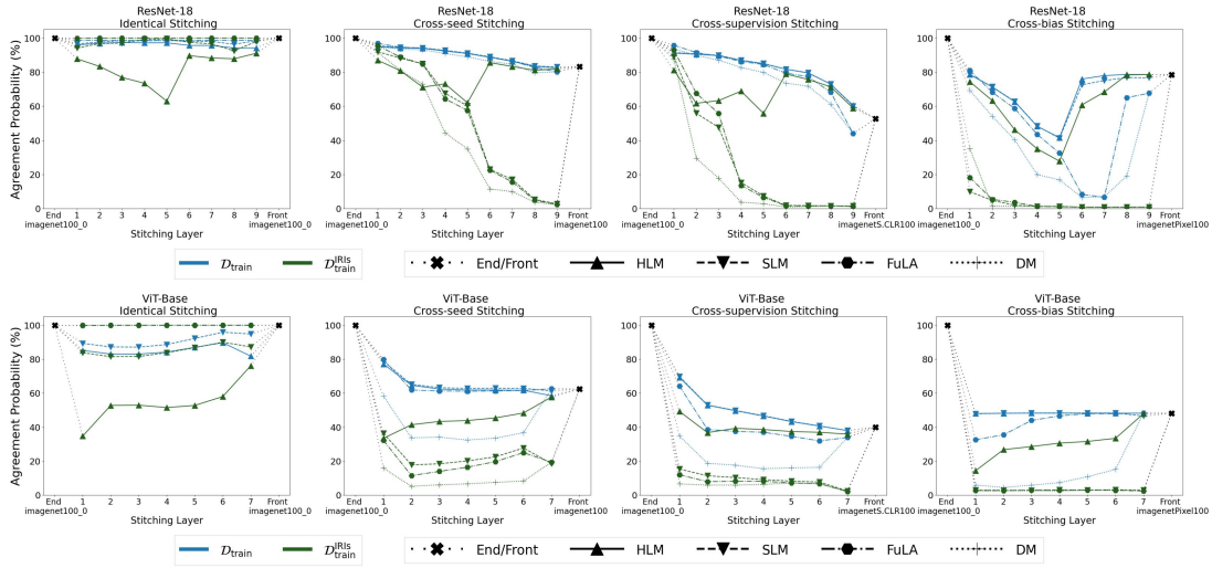
Figure 11. Stitching between models relying on different information (ImageNet-100).
