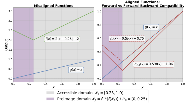
Figure 1. A toy numerical example on function alignment under L2 minimization. When two functions f(x) and g(x) are aligned through an affine transformation h(x) = W \cdot f(x) + b only on the accessible domain \mathcal{X}_a (forward compatibility), they appear perfectly aligned (see h_f(x) ). However, accounting for the preimage domain \mathcal{X}_p (forward–backward compatibility) reveals functional misalignment even within the accessible domain (see h_{f,b}(x) ). Note that the accessible domain and preimage domain are linked through function f .
