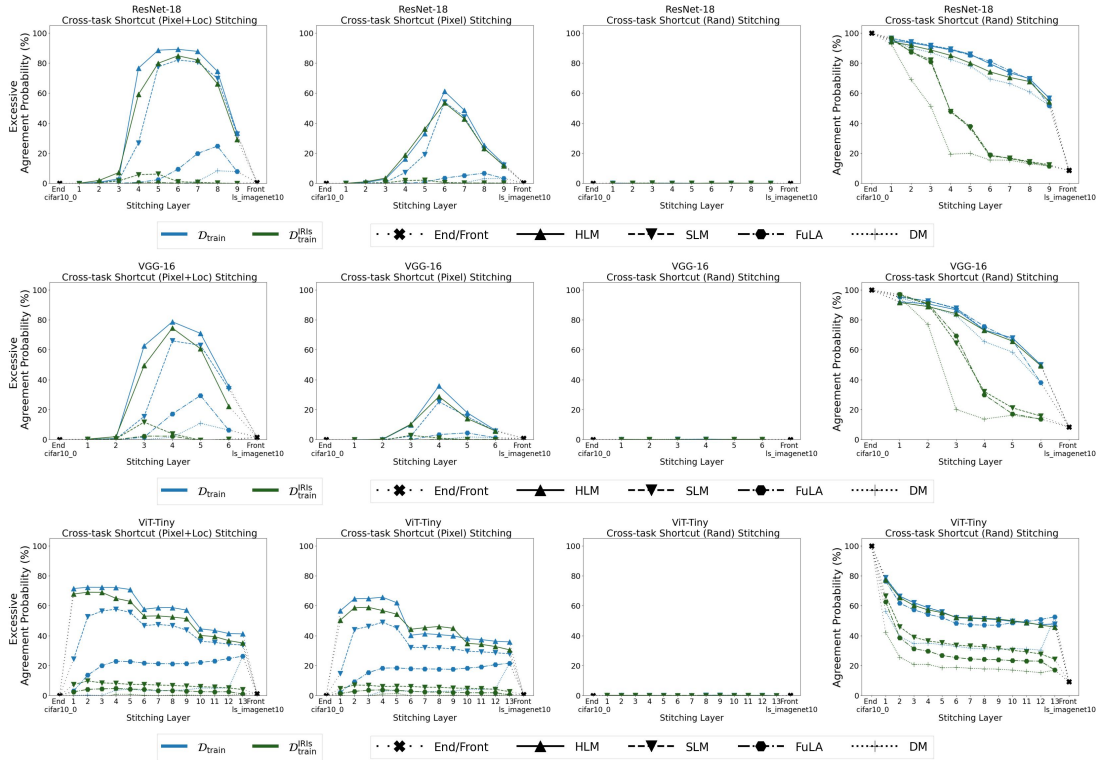
Figure 12. Cross-task stitching under shortcuts of varying availability (CIFAR-10).
