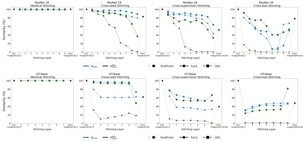
Figure 18. Comparing FuLA and CKA (ImageNet-100).
