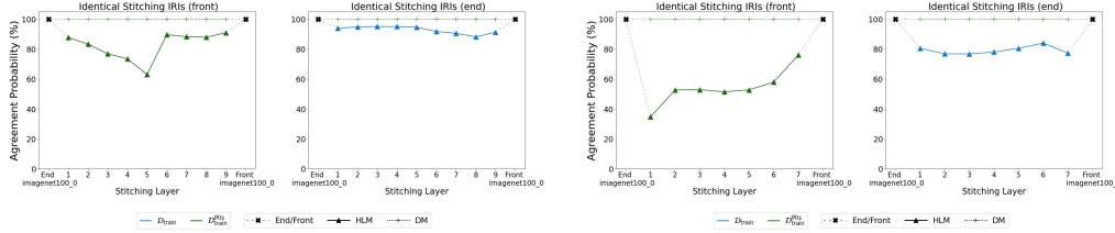
Figure 9. Stitching between identical models using corresponding pairs from \mathcal{D}_{\text{train}} and \mathcal{D}_{\text{train}}^{\text{IRIs}} (ImageNet-100).
