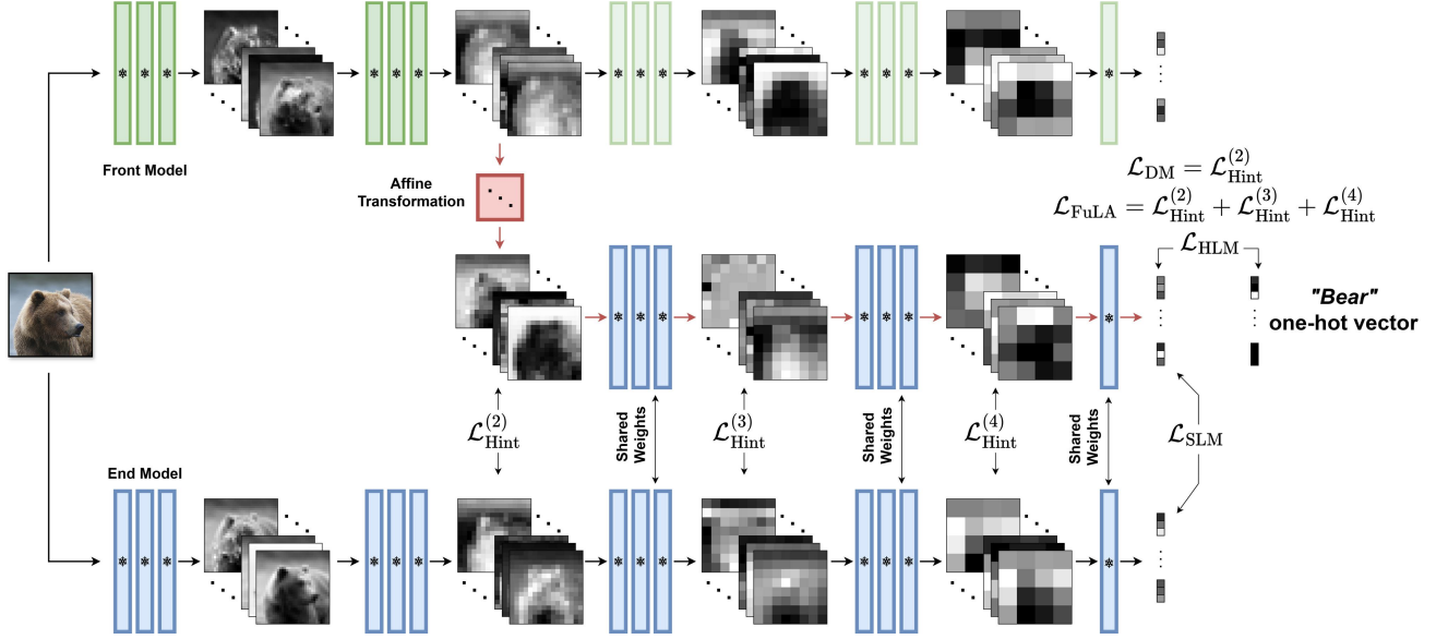
Figure 6. Overview of the different objectives in model stitching for functional similarity evaluation.
