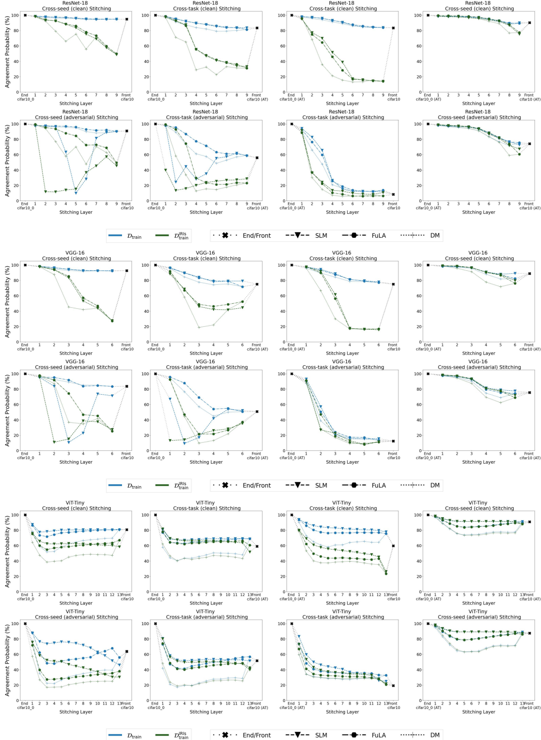
Figure 15. Stitching between robust and non-robust models (CIFAR-10).
