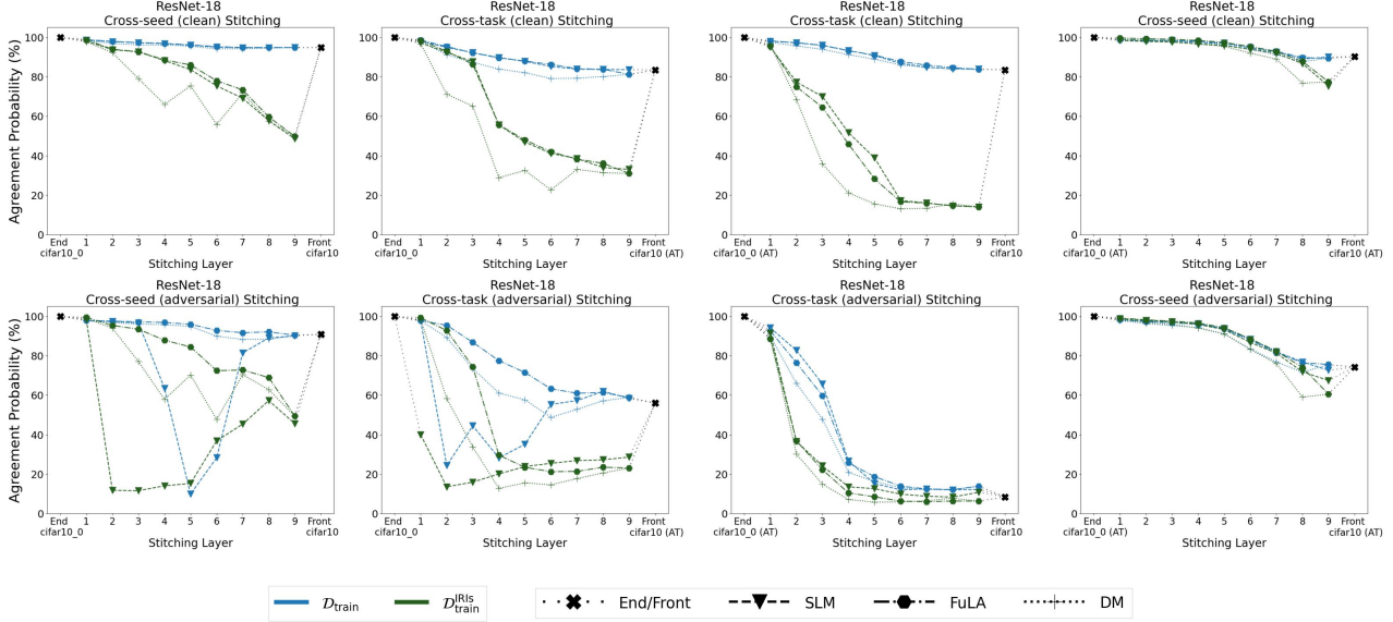
Figure 5. Stitching between robust and non-robust models. The “clean” and “adversarial” labels indicate that the stitching layer is optimized and evaluated using only benign or adversarial samples respectively. Probing for forward-backward compatibility reveals functional incompatibilities previously overlooked. For example, probing only for forward compatibility indicates that the robust and non-robust models are functionally similar with respect to benign samples (i.e., first row), with functional incompatibilities revealed upon probing for forward-backward compatibility.
