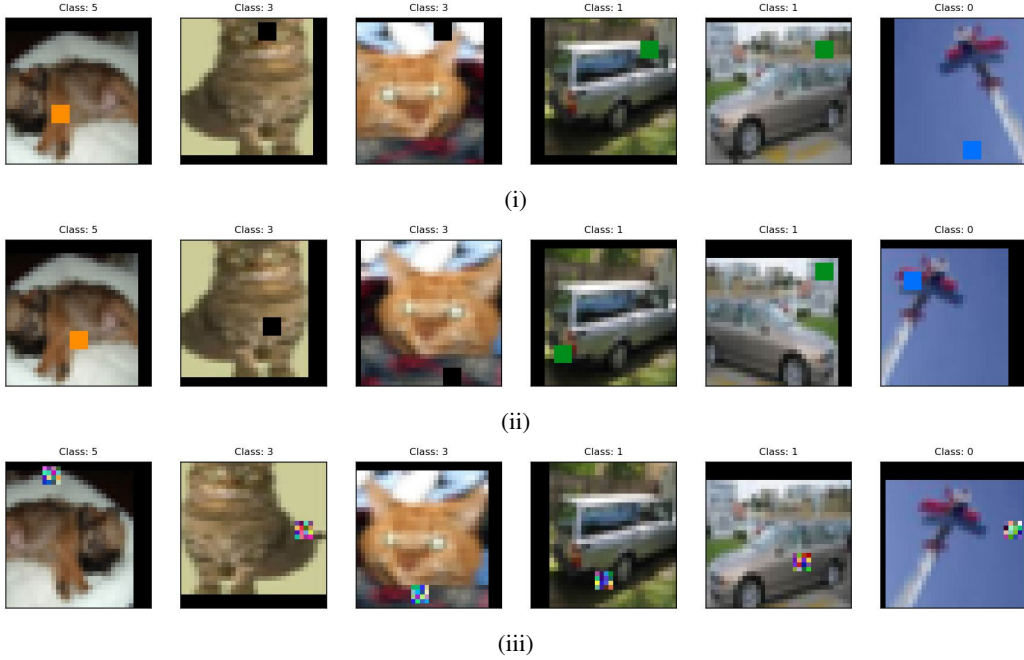
Figure 7. Pixel shortcuts of varying availability. Note that the shortcuts become less available as we transition from top to bottom row.
