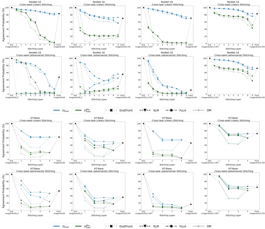
Figure 16. Stitching between robust and non-robust models (ImageNet-100).
