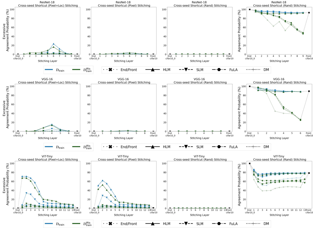
Figure 14. Cross-seed stitching under shortcuts of varying availability (CIFAR-10).
