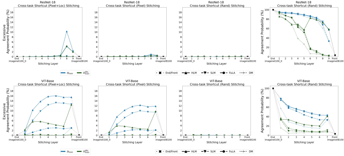
Figure 13. Cross-task stitching under shortcuts of varying availability (ImageNet-100).
