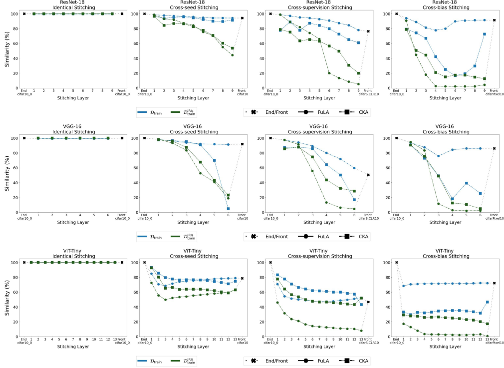
Figure 17. Comparing FuLA and CKA (CIFAR-10).
