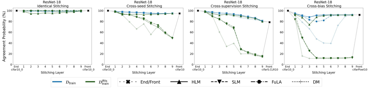
Figure 2. Stitching between models relying on different information. Probing for forward-backward compatibility leads to significantly different, and fundamentally more intuitive functional similarity trajectories compared to only probing for forward compatibility.
