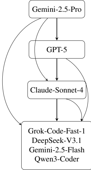
Figure 8. Safety hierarchy (filter present): arrow A \rightarrow B means Model A significantly safer than Model B (McNemar, p < 0.05 ).
