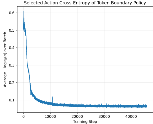
Figure 13. The mean of -\log p_\theta(a_t|a_{<t}) over batches across the training run. We observe that boundaries stabilize after approximately 10% of the training run.
