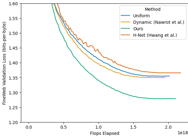
Figure 3. Flops vs validation loss curves for 147M parameter models, trained on FineWeb, measured in bits-per-byte. Uniform random in blue, Straight through estimates in orange, ours in green. Validation loss values at 1.95 \times 10^{18} FLOPs are 1.355, 1.350, 1.36 and 1.279 bits-per-byte respectively
