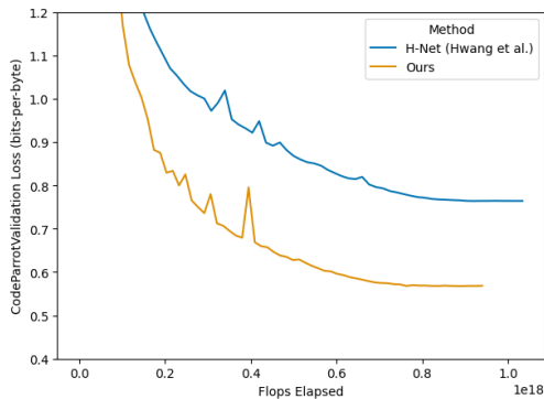
Figure 4. Flops vs validation loss curves for 90M parameter models, trained on CodeParrot, measured in bits-per-byte. H-Net in blue ours in orange. Validation loss values at 0.95 \times 10^{18} FLOPs are 0.769 and 0.568 bits-per-byte respectively
