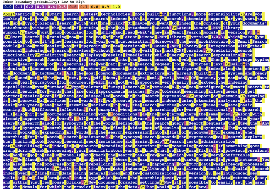
Figure 2. Token boundaries learned by our 147M-parameter model on a held-out sample of the FineWeb dataset. Yellow and blue characters indicate high or low values of \pi_\theta(a) respectively at the corresponding bytes.
