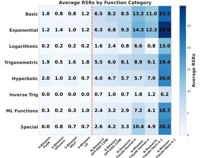
Figure 2. Performance heatmap of average verified RSRs across mathematical function categories. The dotted red line represents the boundary from symbolic to neural methods.
