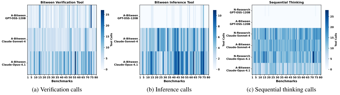
Figure 3. A-BITWEEN’s intensive tool usage across all the benchmarks. Particularly useful proved the sequential_thinking_tool for guiding the exploration and helping the LLM agent.
