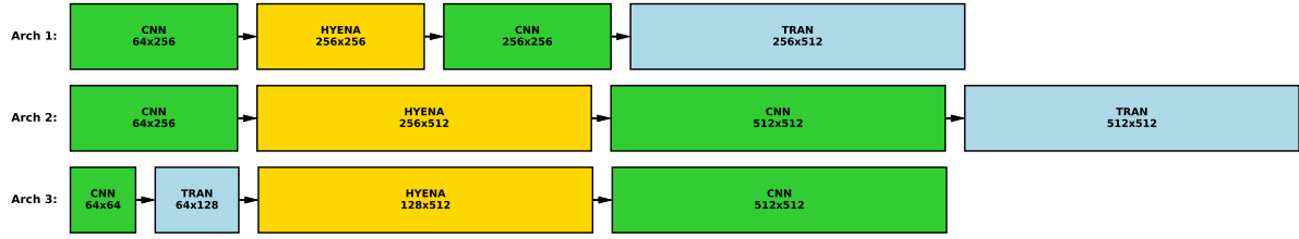
(b) Top-3 architectures with 4 layers.
