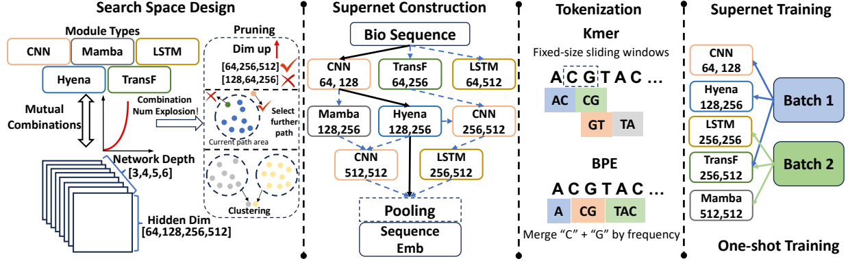
Figure 1. This figure provides an overview of the four core stages of the BioArc framework. (1) Search Space Design: Defines diverse block types, network depths, and hidden dimensions, using pruning and clustering strategies to manage the combinatorial explosion. (2) Supernet Construction: Encodes the vast search space into a single, weight-sharing Supernet, with each path representing a candidate architecture. (3) Supernet Training: Adopts a one-shot methodology, sampling and optimizing different paths across batches for efficiency.
