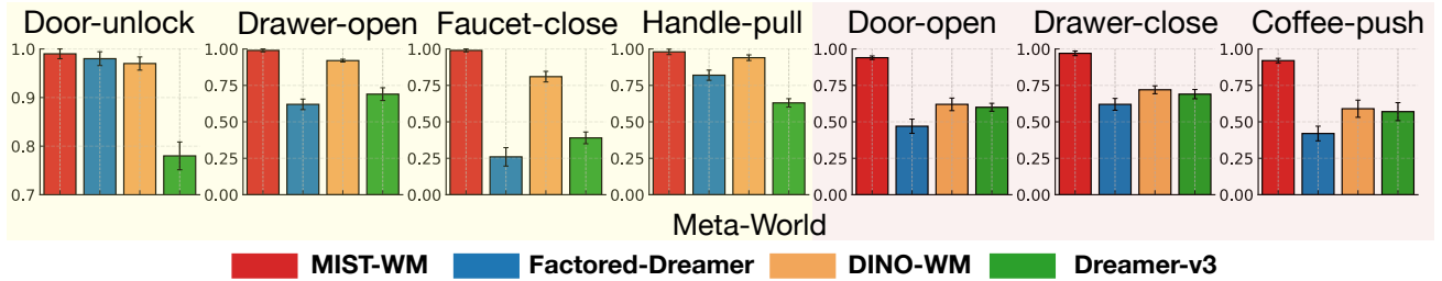
Figure A4. Success rate (across 5 seeds) on skill and compositional generalization, including tasks in Robosuite, Franka-kitchen, and Meta-World. Results in light yellow boxes are those on source tasks, and light pink are those on generalization tasks. Error bars indicate the standard deviation.
