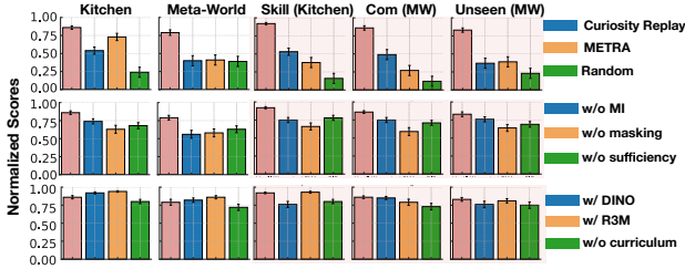
Figure 7. Ablation studies. We consider studies on exploration policy (Row 1); World model terms (Row 2); and Backbones and curriculum (Row 3). Pink bars are original MIST-WM and error bars indicate the standard errors.
