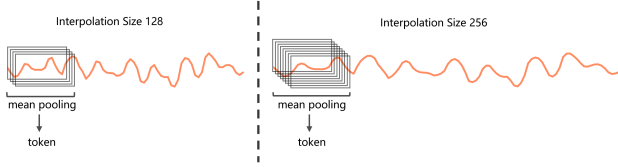
Figure 16. Motivation to look at different interpolation sizes that, in the context of our architecture, imply different degree of overlap between tokens.
