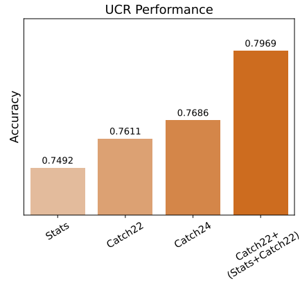
Figure 7. Catch22+ ablation study.
