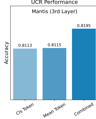
Figure 14. Ablation study on output-token aggregation.
