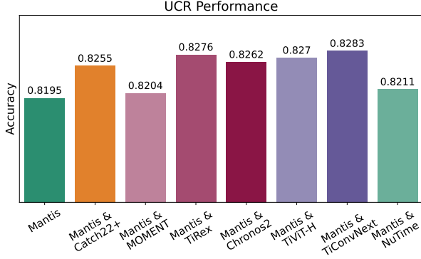
Figure 6. Combination of Mantis with other models.
