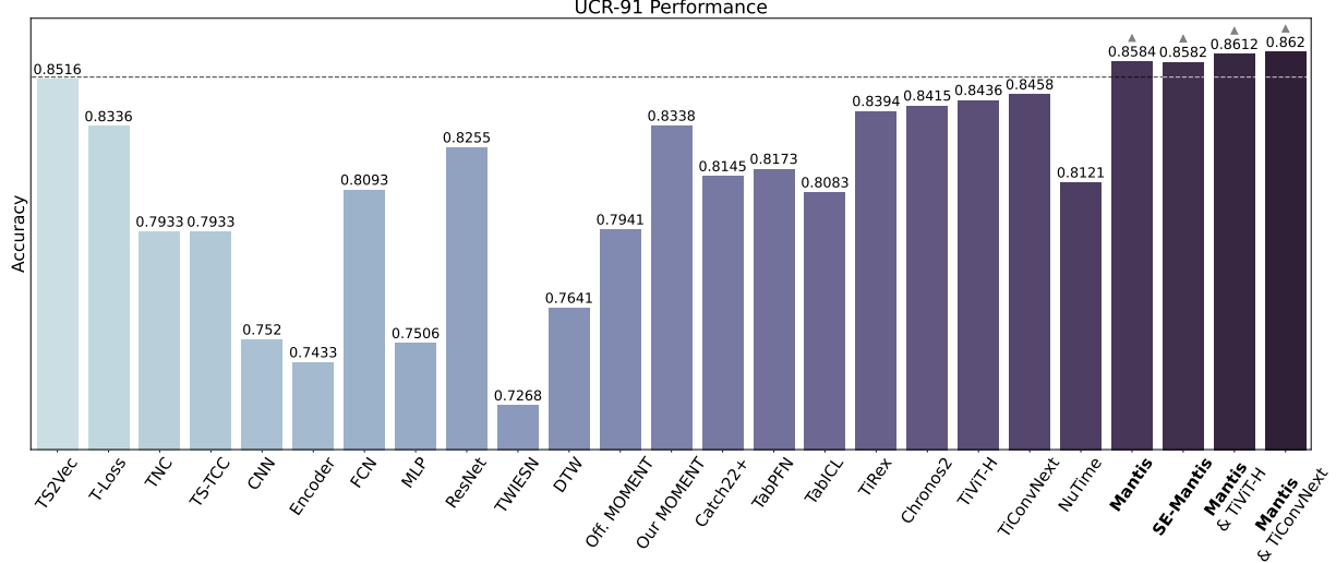
Figure 19. Average performance over 91 datasets from UCR.
