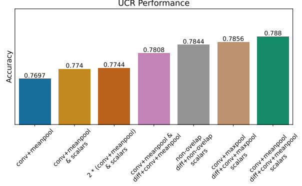
Figure 8. Ablation study for the proposed Token Generator Unit.
