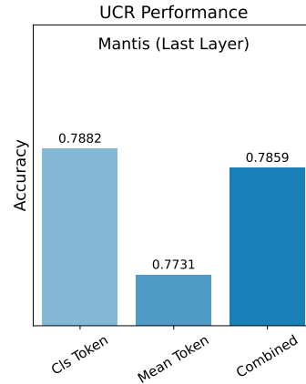
Figure 15. Ablation study on output-token aggregation.
