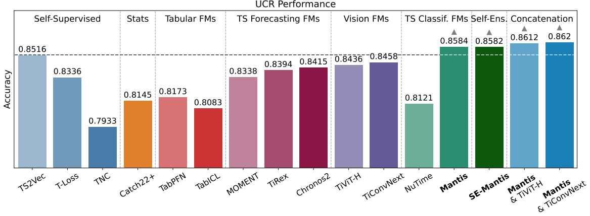
Figure 1. Final Performance on the UCR Benchmark.
