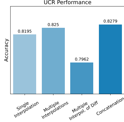
Figure 17. Self-Ensembling Ablation Study.
