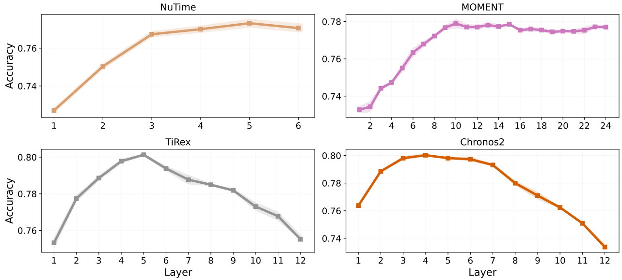
Figure 12. Layer-by-Layer for other models.
