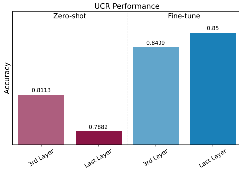
Figure 18. Performance of Mantis in zero-shot and fine-tuned regimes.
