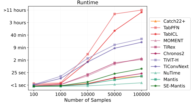
Figure 5. The inference time of the considered models as a function of the number of samples. The time is in log scale.
