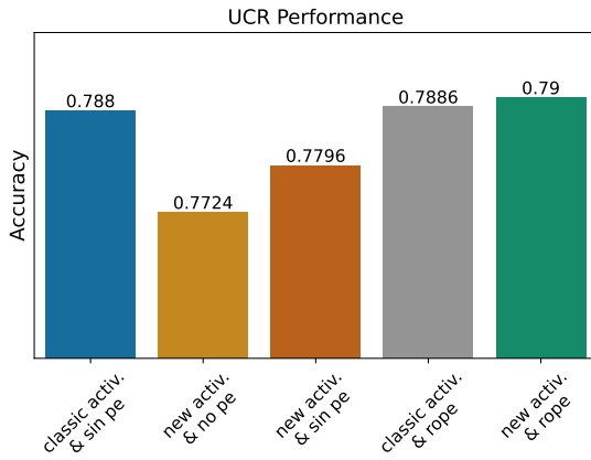
Figure 10. Comparison of different transformer configurations.
