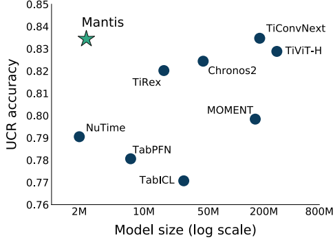
Figure 4. Mantis is the best performing and most lightweight model among the existing FMs.
