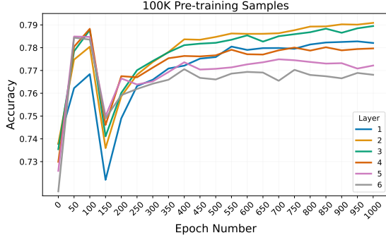
Figure 13. Layer by layer over 1000 epochs with 100K pre-training samples.
