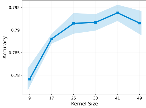
Figure 9. Ablation on convolution kernel size.
