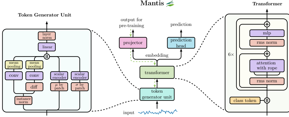
Figure 2. Architecture. By symbol + we denote the sum operator, while || designates the vector concatenation operator.
