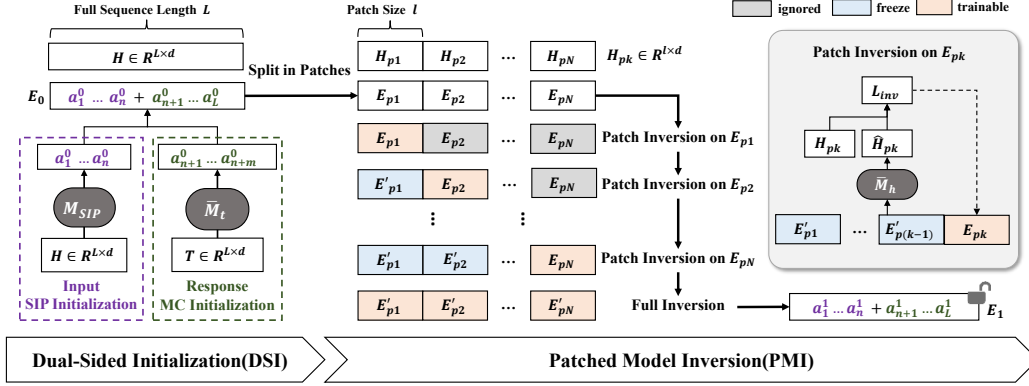
Figure 2. The Two-Stage Attack Methodology of PIDI
