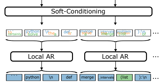
Figure 1. Our CoDiLA in action. a) An example of incoherent text generated by Dream-Coder-Instruct-7B in the first iteration. Due to independent modeling of marginal distributions, it predicts the incoherent token “problem” (Top-1). b) This work enforces local coherence using a block-wise AR model conditioned on soft local tokens. In this example, it recovers coherence by retrieving the correct token “(list” from the Top-3 candidates. Displayed prompt was simplified for illustrative purposes.
