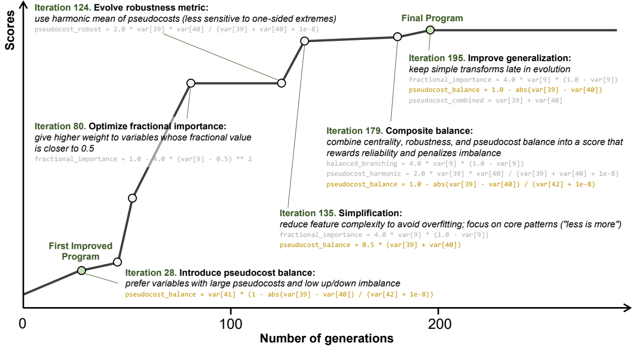
Figure 2. Evolutionary process of the branching policy in LLM4Branch. The curve tracks the solver’s performance improvement over 200 generations. We highlight the key evolutionary milestones, and provide code-level analyses of these corresponding program updates (see Appendix E for full details).
