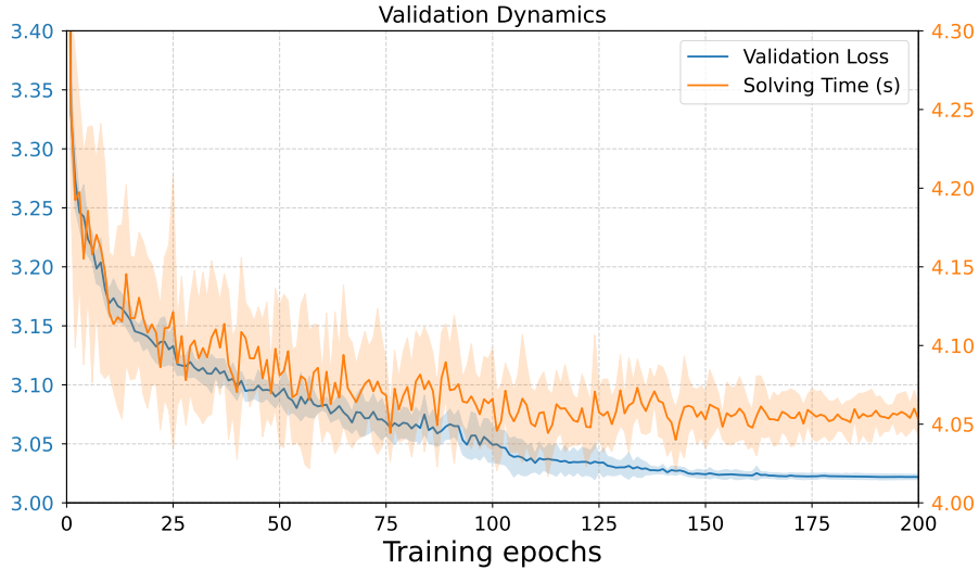
Figure 3. Training dynamics of the MLP policy. The blue curve represents the validation loss, while the orange curve shows the average solving time on the 80 validation instances (shaded areas indicate standard deviation across 10 runs). Although the loss consistently decreases, the solving time stagnates after epoch 100 and exhibits high variance, illustrating the gap between the surrogate objective and actual solver efficiency.
