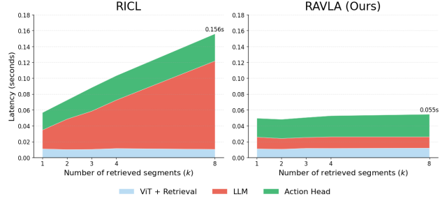
Figure 5. Inference scalability. The latency is averaged over 1,000 inference runs for the generation of a single action chunk. We use 4 denoising steps for the action head. Unlike existing ICIL approaches, RA-VLA enables the seamless integration of multiple expert segments. RAEA shows a similar trend to RICL, as illustrated in Figure 11.
