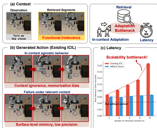
Figure 1. Adaptation bottleneck in existing ICIL frameworks. Existing ICIL methods (a) prioritize superficial visual similarity over functional intent in context retrieval, (b) fail to effectively leverage contextual guidance, and (c) exhibit significant computational overhead for larger contexts. While this overhead is plotted for RICL, other ICIL baselines follow a nearly identical trend.
