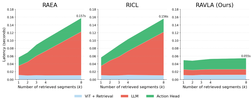
Figure 11. Inference scalability. The latency is averaged over 1,000 inference runs for the generation of a single action chunk. We use 4 denoising steps for the action head. Unlike existing ICIL approaches, RA-VLA enables the seamless integration of multiple expert segments.
