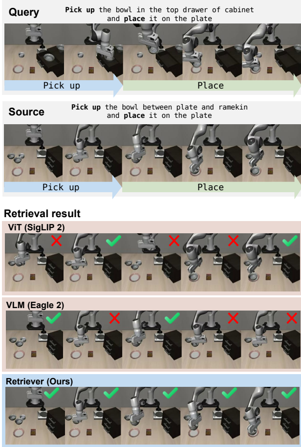
Figure 4. Visualization of segment-level trajectory alignment. For a given query segment, the retrieval model searches for the most relevant segment within the source trajectory. For instance, for the first segment of the query trajectory, the ViT-based retriever identifies the first image in the retrieval results as the most relevant match. However, while the query segment depicts the initial pick-up phase, the retrieved segment corresponds to a later transport phase, illustrating a failure in capturing behavioral relevance.
