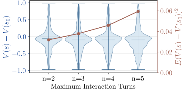
Figure 2. As the maximum interaction turns n grows, the mismatch between V_\pi(s_t) and the fixed baseline \bar{V}_\pi(s_0) can become increasingly severe.
