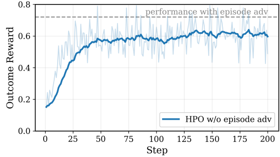
Figure 5. Training reward dynamics of HPO using only step-level advantages with Qwen2.5-3B. The dark blue curve is EMA-smoothed from the raw data. Without episode-level rewards, training remains stable and effective, indicating that step-level advantages provide a reliable learning signal.
