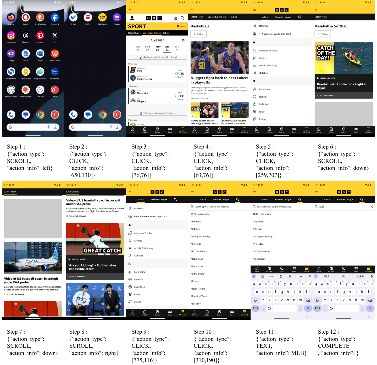
Figure 3. A successful trajectory example. By using Hindsight Goal-Shifting, the agent successfully discovers and executes a sequence of actions that complete the assigned task. The new task instruction is “Using BBC Sports, find out the next MLB game in the search bar.”
