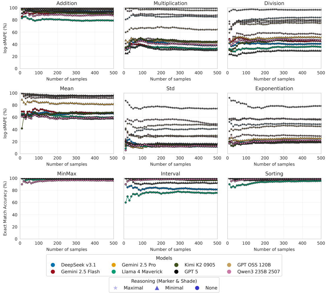
Figure 7. Due to cost constraints we had to subset the full set of 10,000 test samples to 500 samples per task when evaluating the frontier LLMs. We observe performance to already be stable at 500 samples.
