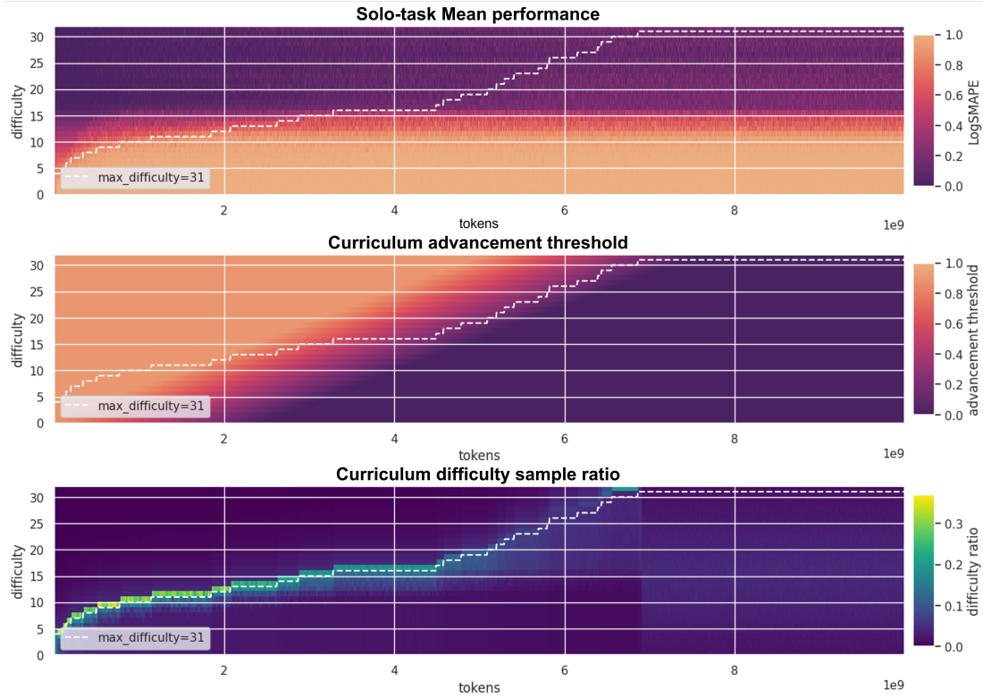
Figure 9. Visualization of the BitTokens curriculum training for the solo-task Mean setting. The difficulty metric does align with the model's performance, but progress plateaus once the model's single forward pass capacity is reached.
