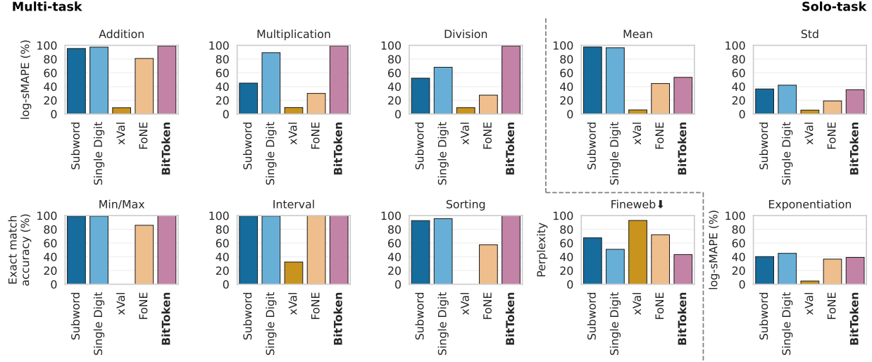
Figure 4. Our BitTokens outperform all other methods in the multi-task setting and is the superior single-token strategy for the multi-step tasks. Between the two multi-token strategies, single digit tokenization performs best, albeit with the highest token cost.
