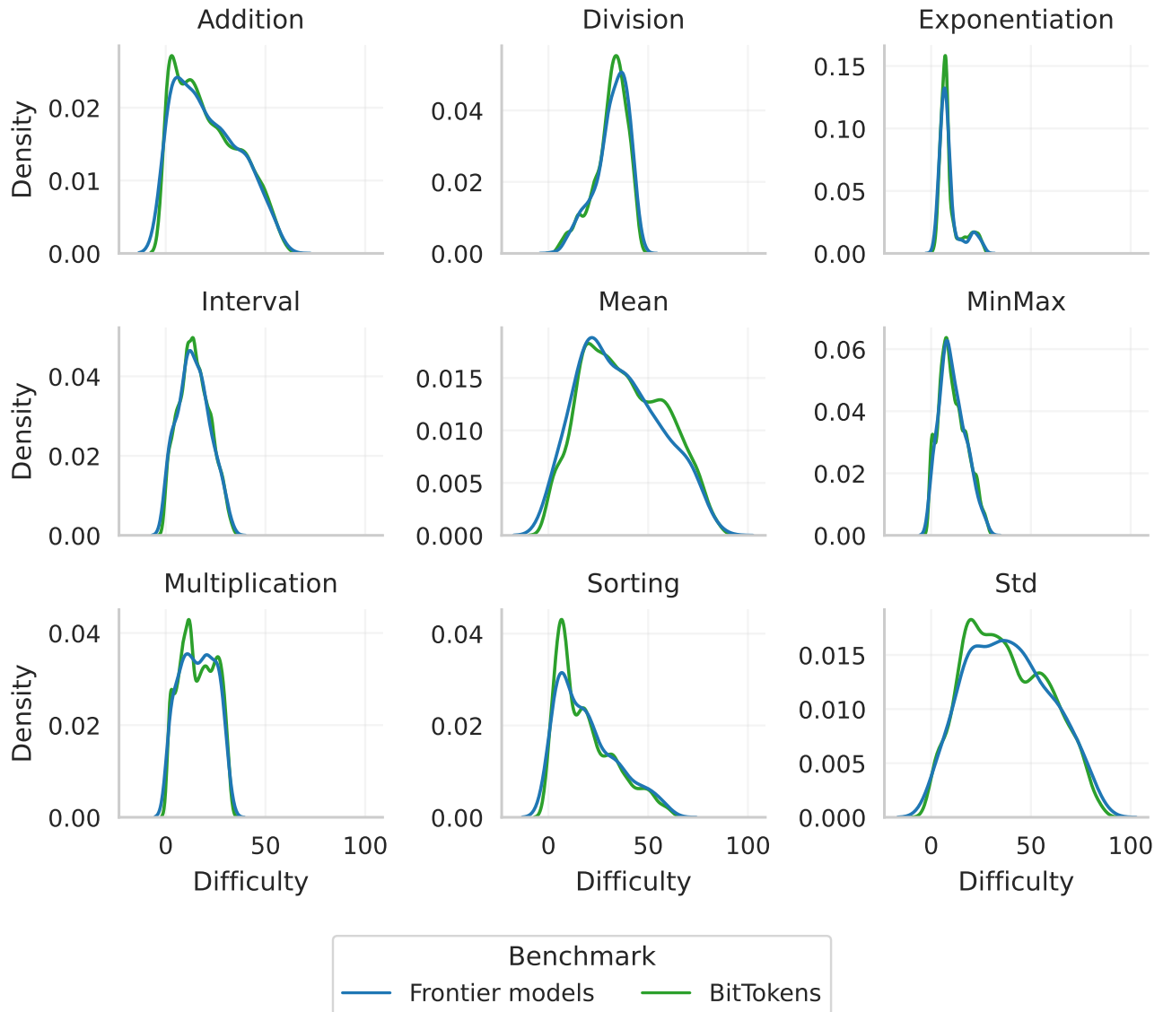
Figure 6. The benchmark for the frontier LLMs is a 500 sample subset of the BitTokens test, but follows the same difficulty distributions.
