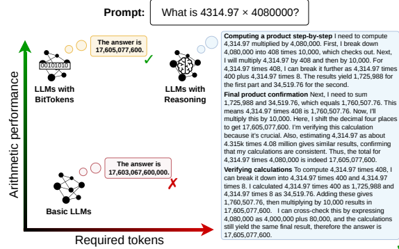
Figure 1. LLMs perform poorly on arithmetic tasks, requiring excessive reasoning tokens to achieve good performance. Our BitTokens tokenization strategy allows language models to solve arithmetic tasks both effectively and efficiently.
