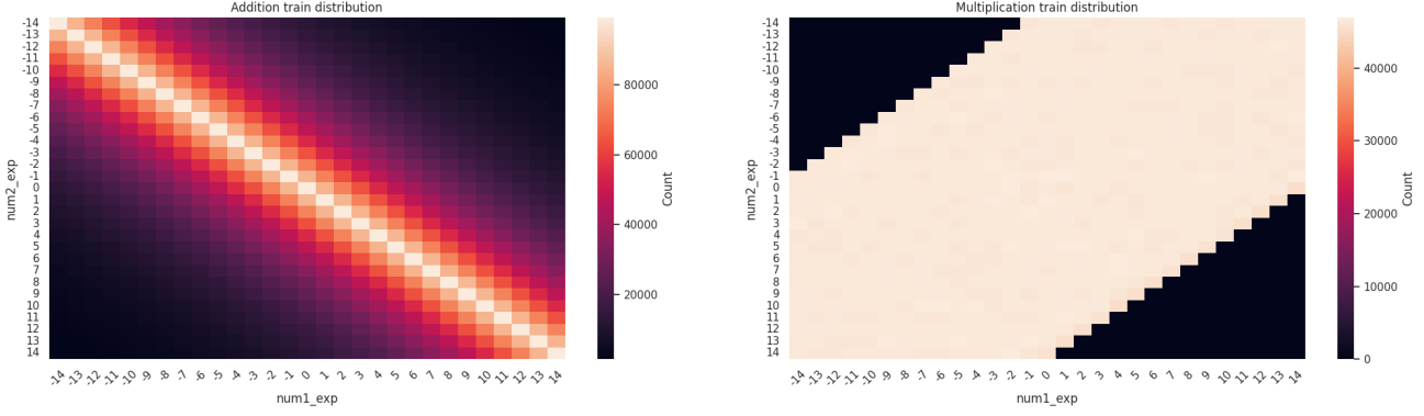
(a) Addition pairs. Operands with similar exponents are oversampled to increase difficulty.
