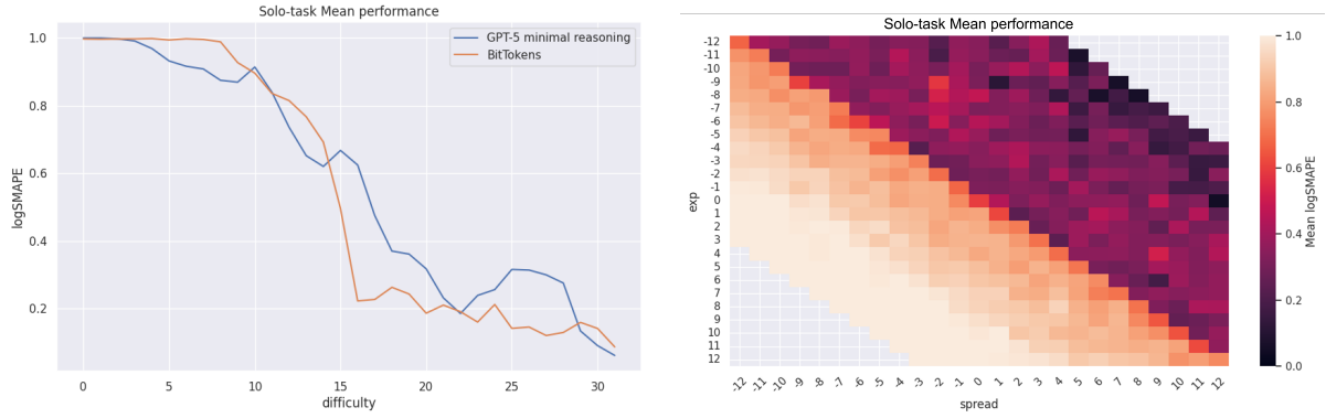
(a) The Mean task performance of BitTokens and GPT-5 with minimal reasoning show a similar performance curve. The chosen difficulty metric directly correlates with the models' performances.
