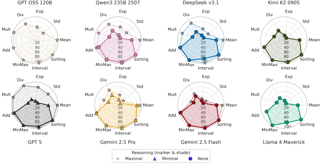
Figure 2. While simple tasks such as addition and sorting are almost perfectly solved by frontier LLMs, other tasks such as multiplication, division, calculating the standard deviation, or exponentiation remain difficult and require extensive reasoning tokens to solve.
