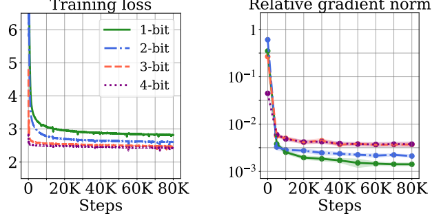
Figure 2. The convergence of the training loss and the relative gradient norm in quantization-aware training from 1-bit to 4-bit precision.
