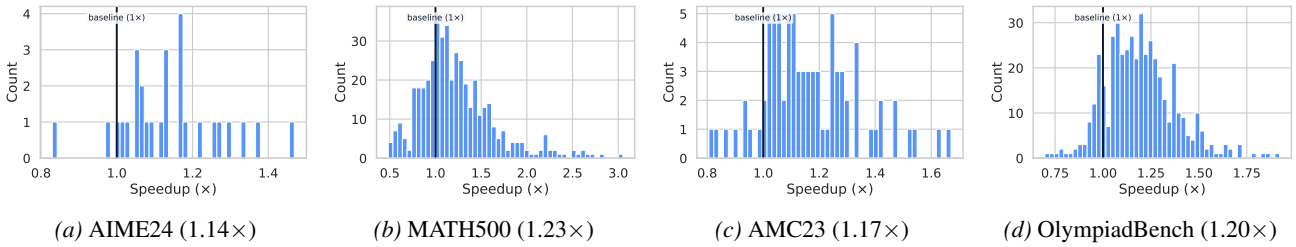
Figure 5. Per-problem speedup distributions on math benchmarks. The speedup is the ratio between the token latency of the sequential reasoning baseline and the token latency of ThreadWeaver. A vertical reference line at 1.0 \times marks parity with the sequential baseline. Parentheses show mean speedup per dataset.
