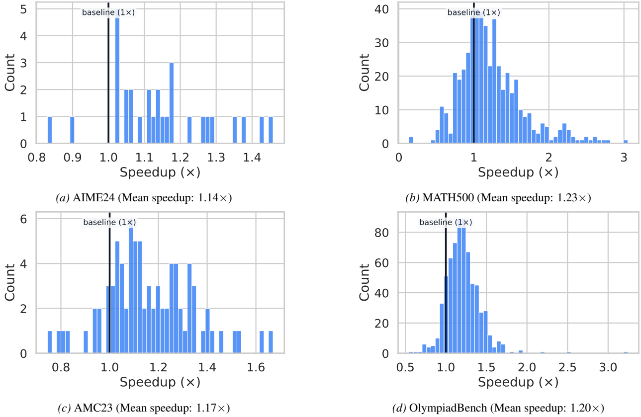
Figure 7. Per-problem speedup distributions on math benchmarks without filtering for correctness. The speedup is the ratio between the token latency of the autoregressive baseline and the token latency of ThreadWeaver. A vertical reference line at 1.0 \times marks parity with the sequential baseline. In contrast to Figure 5, these histograms include all rollouts rather than restricting to samples with correct final answers. However, taking both sets of histograms into account, we show that ThreadWeaver achieves substantial speedup on most problems no matter whether correctness filtering is performed.
