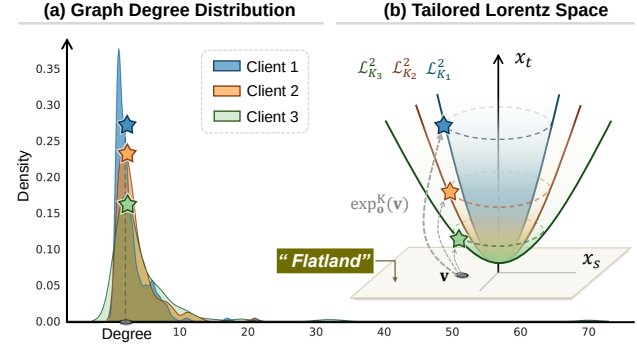
Figure 1. Example: (a) KDE of degree distributions from three CiteSeer clients (Davis et al., 2011), and (b) their respective 2D Lorentz Spaces with different Lorentz scale parameters K .
