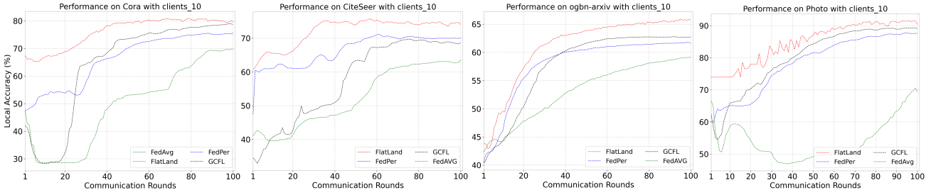
Figure 10. Convergence curves of FlatLand and strong baselines.
