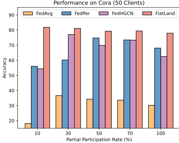
Figure 6. Performance comparison between FedAvg, FedPer, FedHGCN, and FlatLand under different client participation rates on Cora with 50 clients.
