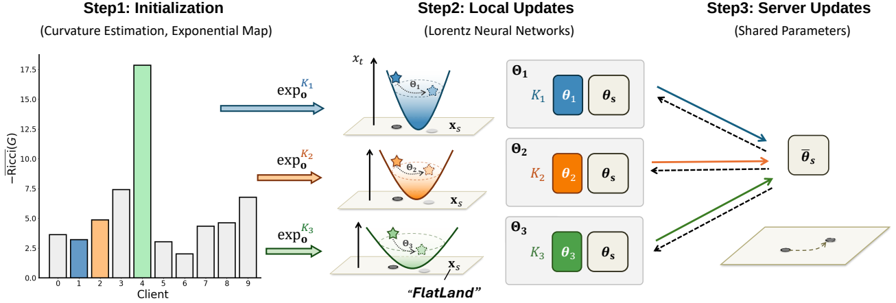
Figure 3. The FlatLand framework. It comprises three stages: (1) Initialization of the client-specific Lorentz scale (Section 5.1), personalized, and shared parameters; (2) Local updates within client-specific Lorentz spaces (Appendix C.2.3); and (3) Server updates, aggregating only shared parameters while preserving personalization by keeping personalized parameters locally (Section 5.2).
