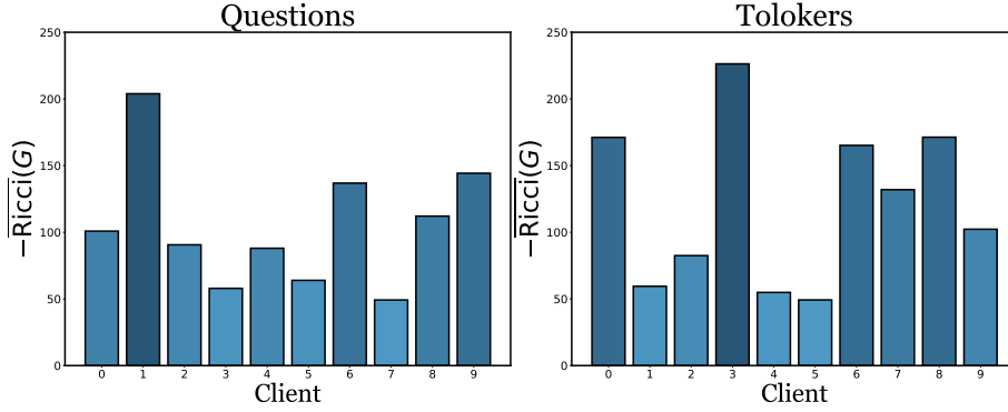
Figure 9. Averaged Forman-Ricci curvature across heterophilic datasets (Questions and Tolokers). Higher bars indicate more pronounced non-Euclidean characteristics in these datasets.
