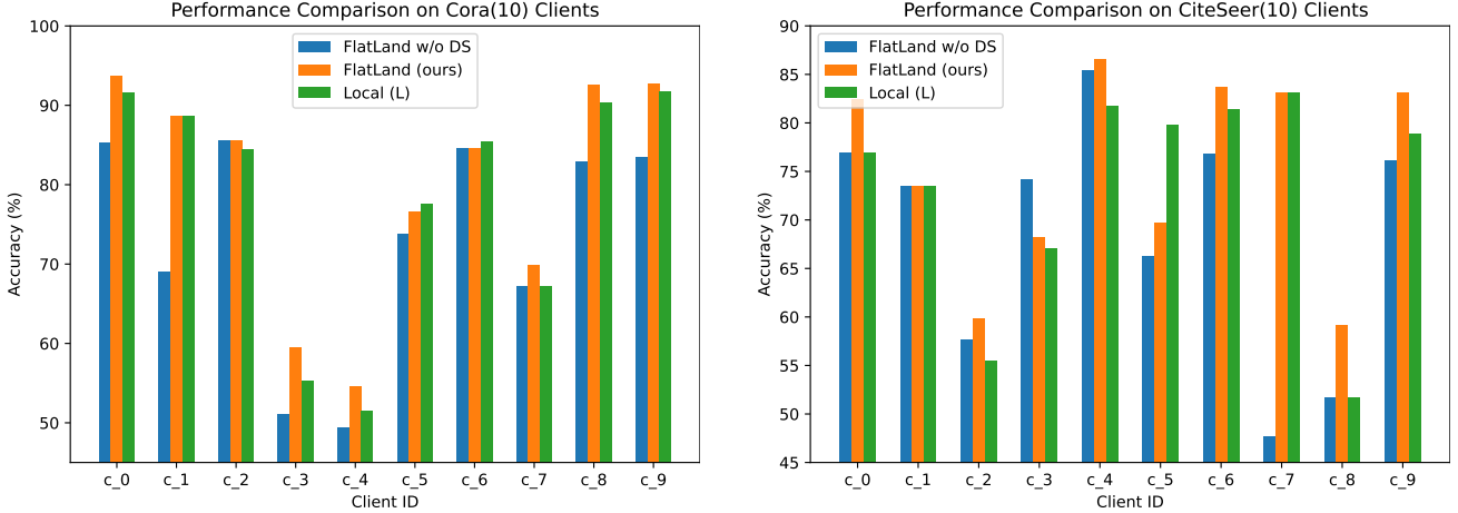
Figure 7. Client-level performance comparison on Cora (left) and CiteSeer (right) with 10 clients. Each group corresponds to one client and reports accuracy of FlatLand w/o DS, FlatLand, and Local (L). FlatLand improves most clients, while removing DS causes client-wise degradation, supporting the role of time-like parameter decoupling.
