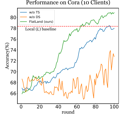
Figure 5. Ablation study of FlatLand on the Cora dataset.
