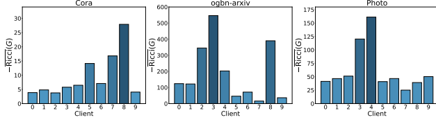
Figure 2. Averaged Forman-Ricci curvature across datasets (Cora, ogbn-arxiv, and Amazon-Photo). Higher bars indicate more pronounced non-Euclidean characteristics in these datasets.
