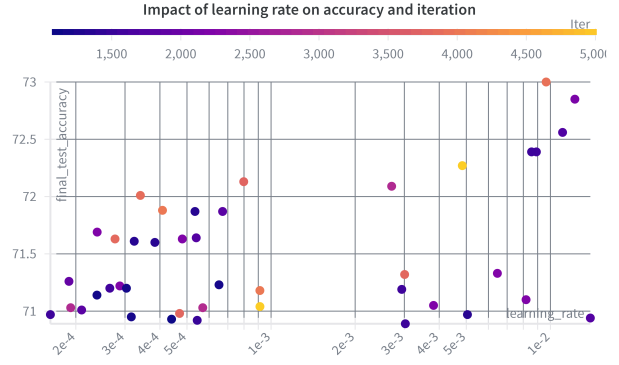
Figure 4. Impact of learning rate on accuracy and iterations on CNN model over CIFRA-10. The total steps are 10000. Darker points indicate faster convergence.
