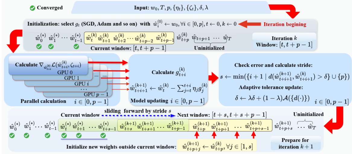
Figure 6. Illustration of Step-parallel Training Paradigm PASO. During iteration k , PASO performs simultaneous weight updates across steps within a p -size sliding window through parallel gradient computations. The process consists of: (1) computing update terms g^{(k)} based on current weights \hat{w}^{(k)} after calculating their gradients in parallel; followed by (2) determining new weights \hat{w}^{(k+1)} .
