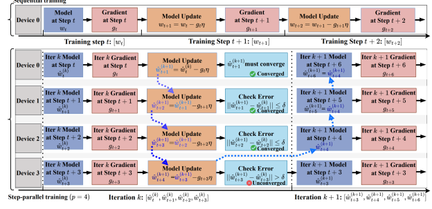
Figure 1. Illustration of our step-parallel training framework. PASO computes gradients in parallel within a p -sized window (here p = 4 ), followed by the communication of updated models. Throughout this process, each device maintains the computation graph for only a single step.
