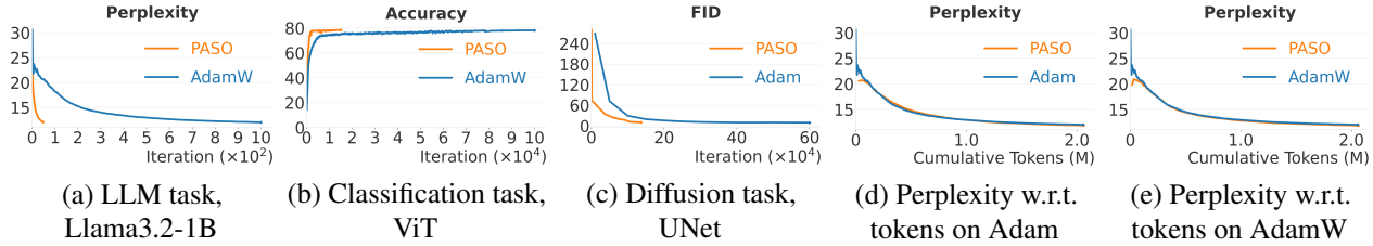
Figure 3. The comparison of perplexity, FID, and accuracy curves. Note that Figs. (d) and (e) give comparison of perplexity curves w.r.t. the cumulative token consumption on Llama 3.2-1B over WikiText-2.
