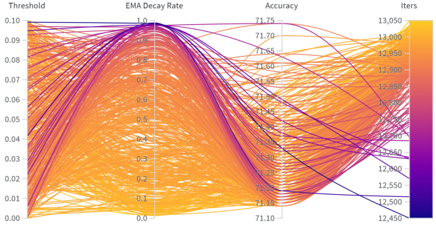
Figure 5. The impact of \delta and \lambda over CIFAR-10 by running 1200 experiments. We use PASO with p = 7 to accelerate Adam with 60000 steps. Darker lines indicate runs with fewer iterations.
