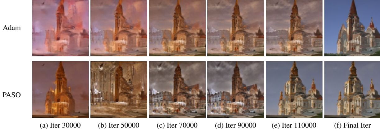
Figure 2. Visual comparison of sampling results across different training iterations for diffusion models from Adam and PASO plus Adam. Each column represents the same training iteration. Please refer to Fig. 7 in App. E.8 for more visual comparisons.
