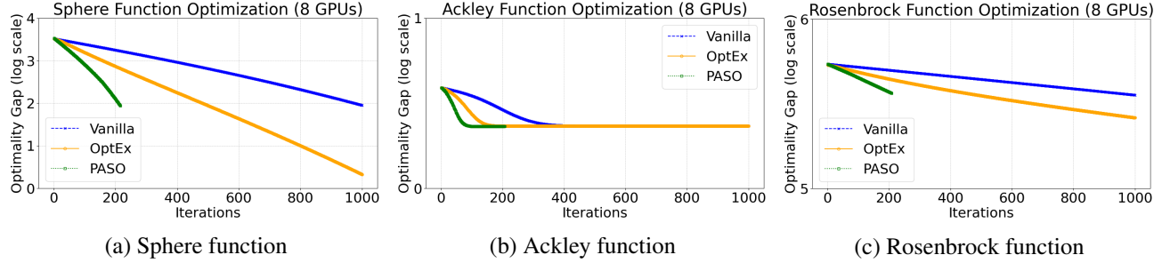
Figure 8. The comparison of optimality gap when optimizing the Sphere function, the Ackley function, and the Rosenbrock function.
