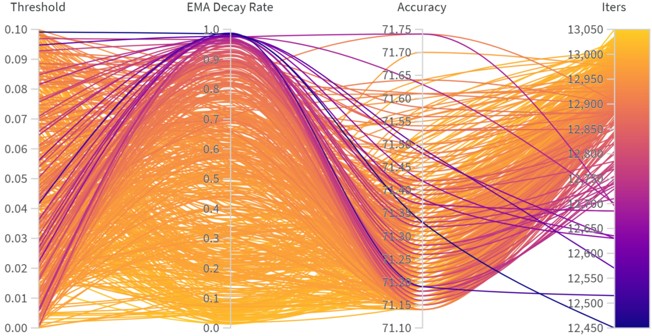
Figure 9. The impact of \delta and \lambda over CIFAR-10 by running 1200 experiments. We use PASO with p = 7 to accelerate Adam with 60000 steps. Darker lines indicate runs with fewer iterations.
