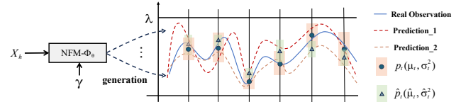
Figure 1. A single trained NFM \Phi_\theta can generate multiple forecasts from a fixed input X_h under various states \gamma and \theta . These forecasts are expected to follow the empirical process ( \hat{p}_t , t = 1, 2, \dots ) approximated by the NFM with the observed data. The model-estimated process is distinguished from the real data distribution ( p_t , t = 1, 2, \dots ) by a bias b_t .
