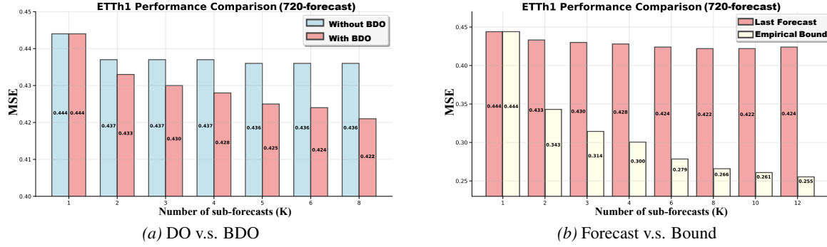
Figure 7. Performance variation with different numbers of sub-forecasts K. (a). Comparison of using DO or BDO. (b). Comparison between the last forecast and the empirical bound of ReNF.
