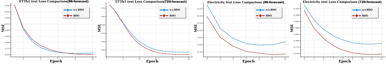
Figure 6. Effect of the BDO forecast.
