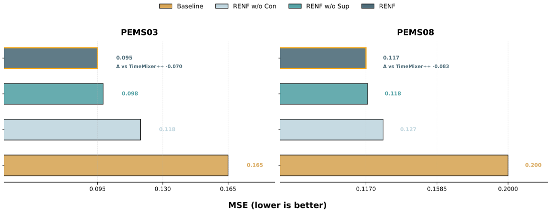
(b) Ablation of BDO on PEMS Datasets.
