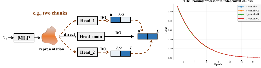
Figure 2. We compare the forecast by applying independent linear heads to predict several non-overlapped chunks of the horizon using a shared representation, with a main head for the whole horizon using the same representation. The right figure shows that the training loss curves in different settings are nearly identical under the DO strategy, indicating a lack of temporal dependencies.
