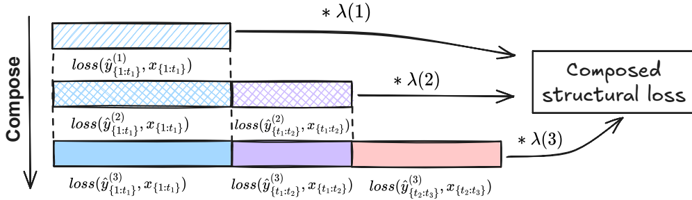
Figure 8. Illustration of the implicit structural loss of BDO, we exemplify it in the NF consisting of three sub-forecasters.
