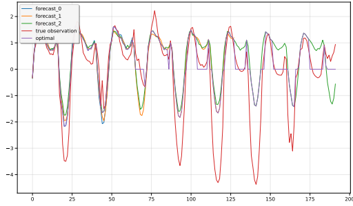
(e) 192-prediction on the ETTh1 dataset
