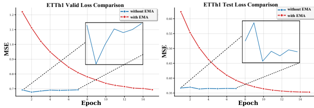
Figure 4. Variation of valid and test loss with and without applying EMA weight averaging. The valid loss and test loss manifest significant inconsistency during the learning process of NFs without smoothing, biasing the underlying evaluations of NFs.
