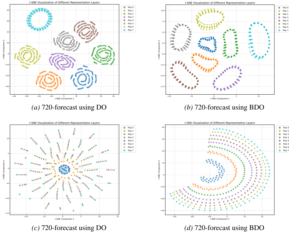
Figure 11. Visualizations of the representations of different layers/sub-forecasters. (a). representations of using DO with the ETTh1 dataset. (b). representations of using BDO with the ETTh1 dataset. (c). representations of using DO with the ETTm1 dataset. (d). representations of using BDO with the ETTm1 dataset. This indicates that BDO tends to form predictive representations that are homogeneous and hierarchical.
