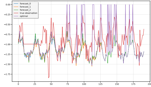
(f) 192-prediction on the ETTh2 dataset
