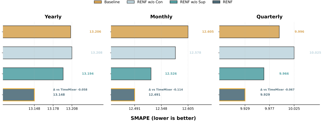
(a) Ablation of BDO on M4 Datasets.
