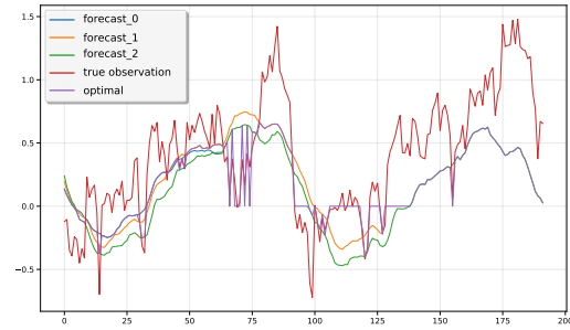
(h) 192-prediction on the ETTm2 dataset
