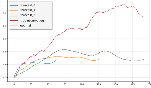
(a) 192-prediction on the weather dataset
