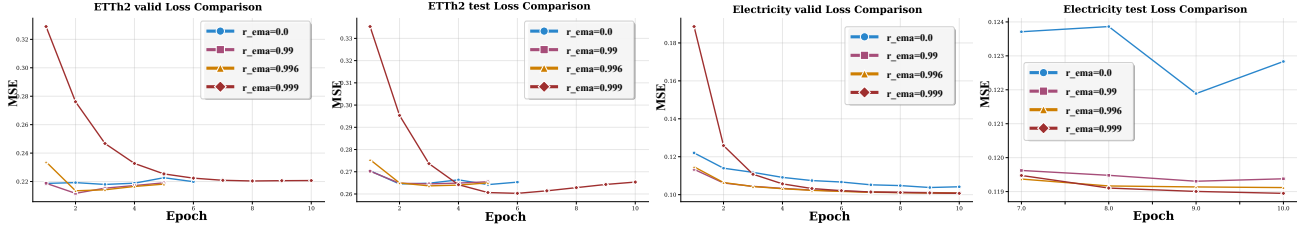
Figure 5. Effect of the EMA smoothing on training and test phase. "r_ema" denotes the applied ratio \alpha of EMA weighting.
