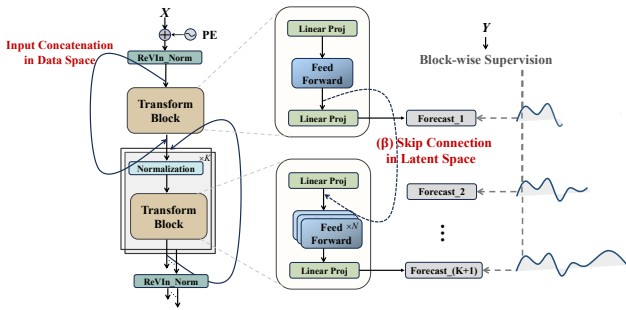
Figure 3. Model structure of ReNF. “PE” denotes optional temporal embedding, and the \beta version adds additional skip-connections for deeper representations.
