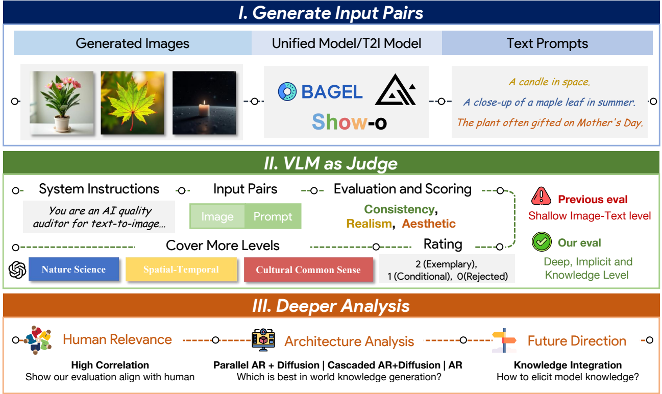
Figure 2. Illustration of the WISE framework, which employs a three-stage evaluation process (Panel I to III) to systematically evaluate generated content across three core dimensions. In the two representative cases, the science-domain input “candle in space” violates oxygen-dependent combustion principles, while the spatiotemporal-domain input “close-up of summer maple leaf” contradicts botanical seasonal patterns. Both receive 0 in consistency (see Evaluation Metrics in Panel II), confirming the benchmark’s sensitivity to world-knowledge conflicts.
