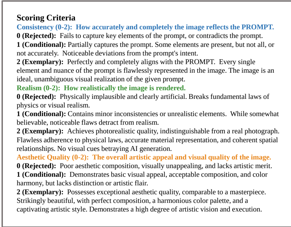
Figure 5. WISE assesses image quality using three criteria: how accurately the image aligns with the prompt (Consistency), its level of realism (Realism), and its overall artistic appeal (Aesthetic Quality). Each metric is scored on a scale from 0 (Rejected) to 2 (Exemplary), providing an evaluation of image fidelity, believability, and visual quality.
