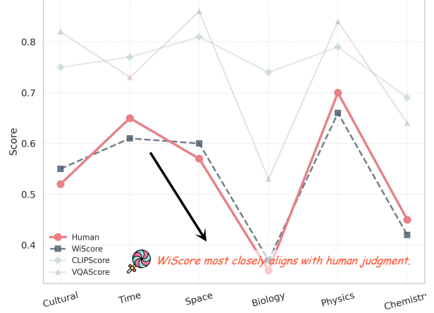
Figure 4. Evaluation results of different metrics, where WiScore most closely aligns with human assessment.
