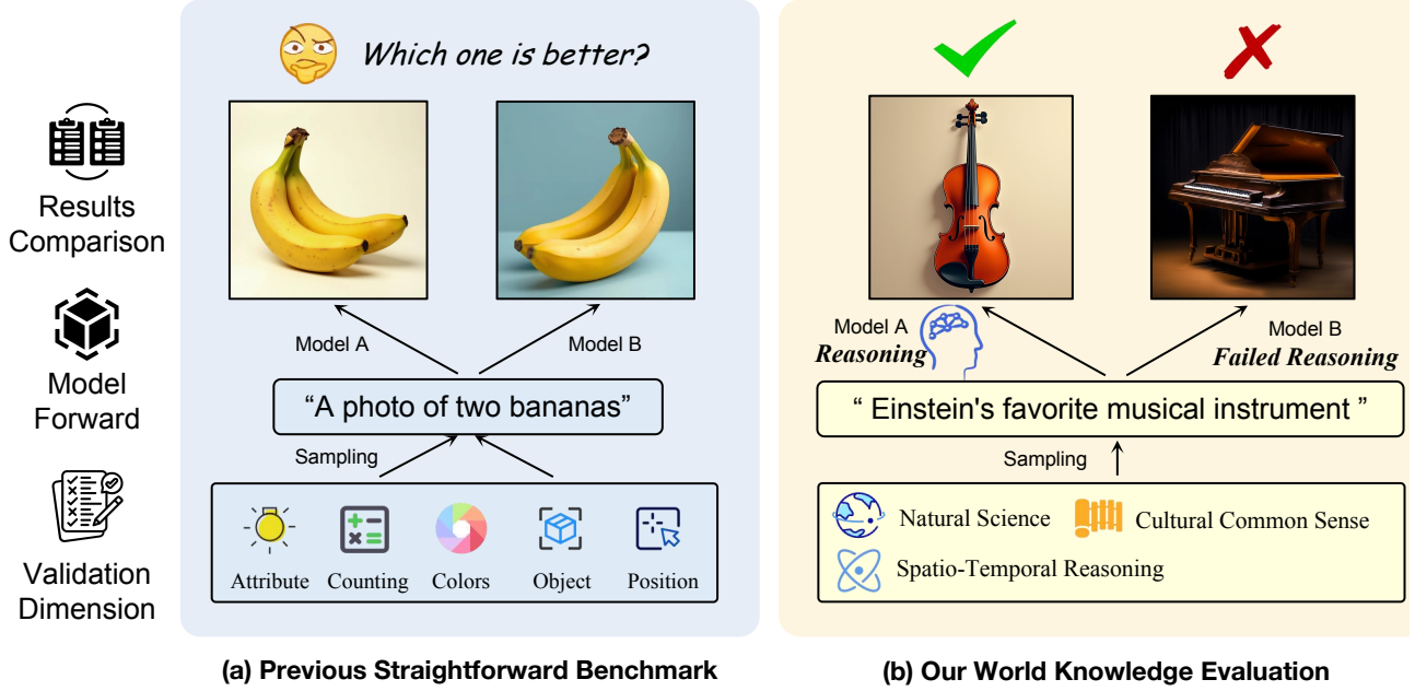
Figure 1. Comparison of previous straightforward benchmarks and our proposed WISE. (a) Previous benchmarks typically use simple prompts, such as “A photo of two bananas” in GenEval (Ghosh et al., 2024), which only require shallow text-image alignment. (b) WISE, in contrast, uses prompts that demand world knowledge and reasoning, such as “Einstein’s favorite musical instrument,” to evaluate a model’s ability to generate images based on deeper understanding.
