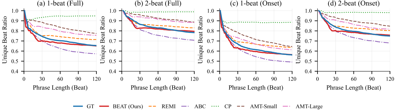
Figure 3. Unique beat growth curves for music continuation. The x -axis is beat position, i.e., the prefix length measured in beats; the y -axis is the cumulative unique beat ratio over the first t beats, averaged across the 200 continuations per method (same set as Sec. 4.3). BEAT (red) closely tracks ground truth (blue), while Compound Word (green) shows excessive diversity and Interleaved ABC (purple) shows excessive repetition.
