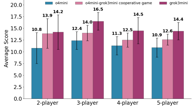
Figure 7. Average Hanabi score across 2–5 players for three team compositions: (left) all o4-mini, (middle) one Grok-3-mini agent and the remaining o4-mini agents, and (right) all Grok-3-mini agents. Error bars denote standard deviation.
