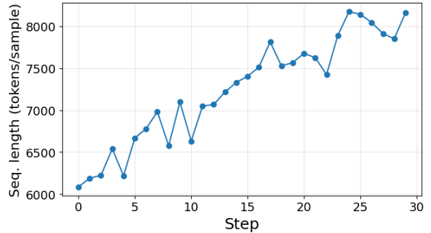
Figure 24. Mycroft mean sequence length vs steps. We stopped training at 30 steps and started a new run with this checkpoint as the max sequence length exceeded the context window.
