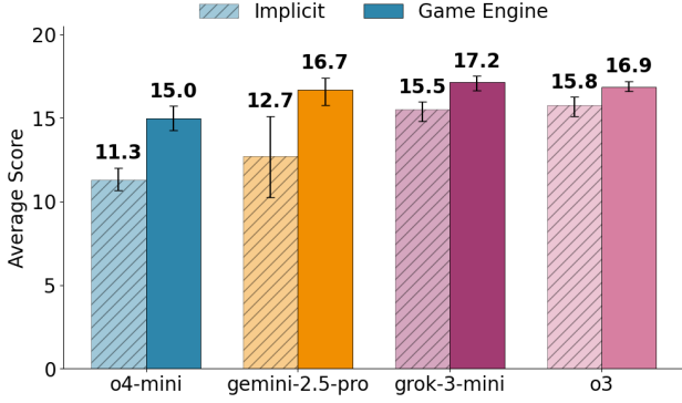
Figure 12. IQM Hanabi scores for the best reasoning LLM agents with Implicit deductions (Mycroft) vs Game Engine deductions (Sherlock) averaged across 2-5 Player settings. Error bars denote 95% CI.
