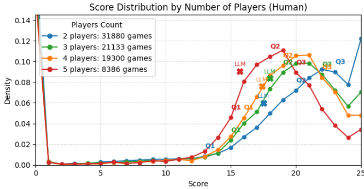
Figure 21. Distribution of human Hanabi scores (2–5 players) collected from BoardGameGeek. LLM markers show average scores of the best-performing model per player count in the Sherlock setting: o3 for 2p and 5p and grok3mini for 3p and 4p.
