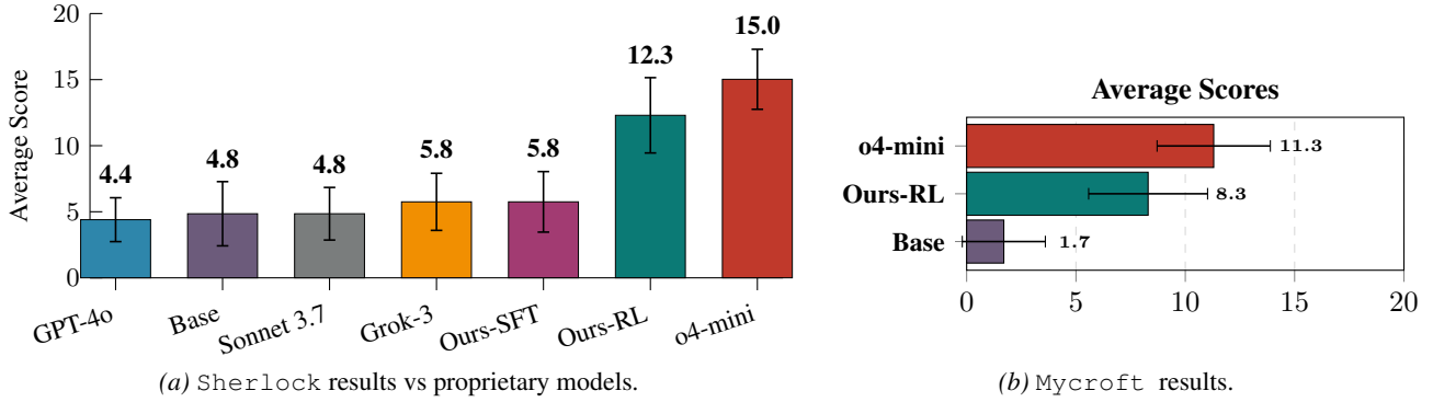
Figure 8. Left. Sherlock results: Average scores of Qwen3-4B-Instruct-2507 (Base) before and after instruction tuning on HanabiLogs (Ours-SFT) and RL on HanabiRewards (Ours-RL) versus Grok-3, Claude Sonnet 3.7, GPT-4o, and o4-mini, averaged over 5 games for each player count (2–5). Models were evaluated on different seeds to avoid potential leakage (see App. B). Right. Mycroft results: Average scores of Qwen3-4B-Instruct-2507 before and after finetuning on HanabiRewards versus o4-mini. Error bars denote SD.
