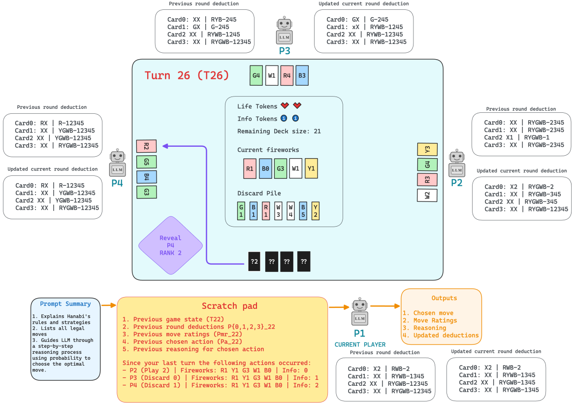
Figure 3. An example game state as viewed by Player 1 in the Mycroft setting. We note that each player has an independent deduction block for all other players hands. In this figure, we only show Player 1’s deduction blocks for all other players.
