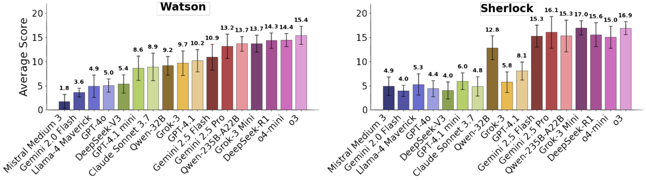
Figure 4. Scores of 17 state-of-the-art LLM Hanabi agents averaged over two to five-player settings. We show scores for each specific player count in both settings in Figure 18 (Appendix D.2). Error bars denote standard deviation.
