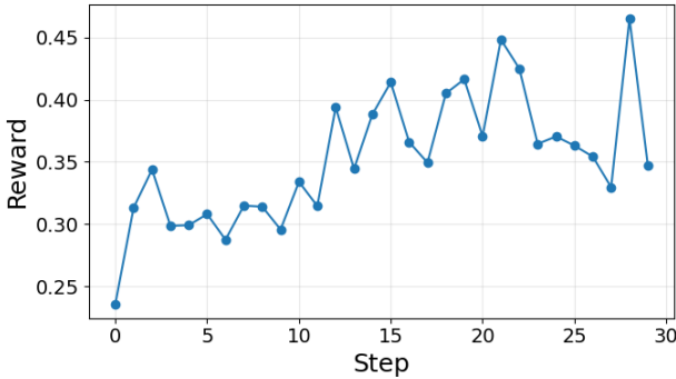
Figure 23. Mycroft reward vs steps. Note: We stopped the training at 30 steps and started a new run with this checkpoint as the max sequence length exceeded the context window.
