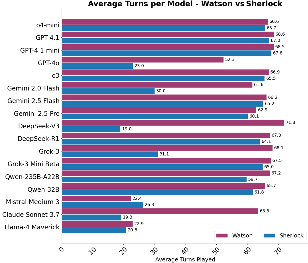
Figure 9. Average number of turns played by each model, averaged over the two- through five-player settings.
