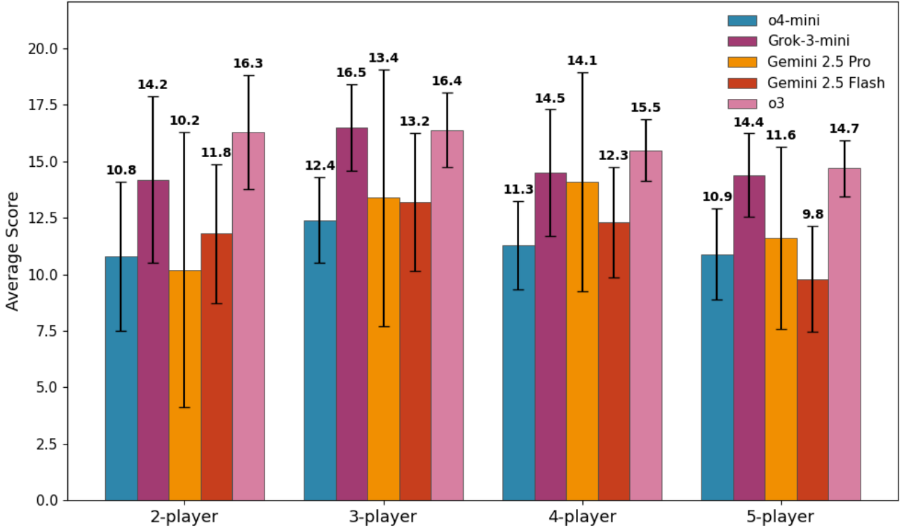
Figure 17. Mycroft scores of reasoning models across 2-5 player settings.
