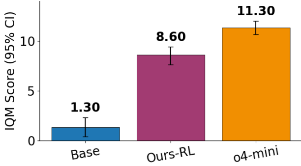
Figure 15. Mycroft : IQM scores of Qwen3-4B-Instruct-2507 before and after finetuning on HanabiRewards vs o4-mini. Note: We evaluated the Qwen3-4B-Instruct-2507 models on different seeds to avoid memorization effects. Error bars denote 95% CI.
