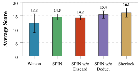
Figure 2. Average scores in 5 player Hanabi game for 10 runs of Grok-3-mini with different prompt strategies. Error bars denote standard deviation.
