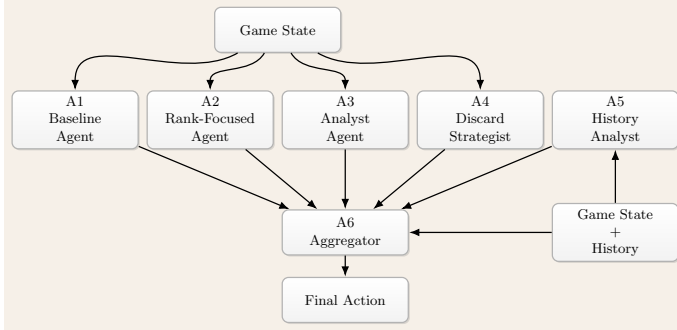
(a) The Mixture-of-Agents system utilizes five parallel agents with specialized roles to generate diverse reasoning outputs, which are then synthesized by an Aggregator Agent (Agent 6) to select the optimal move.
