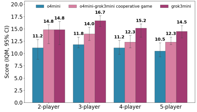
Figure 13. IQM Hanabi score across 2-5 players for three team compositions: (left) all o4mini, (middle) one Grok-3-mini agent and the remaining o4-mini agents, and (right) all Grok-3-mini agents. Error bars denote 95% CI
