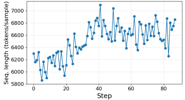
Figure 26. Sherlock mean seq. length vs steps.
