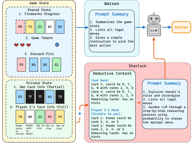
Figure 1. A comparison of the Watson : provides basic game state with only explicit knowledge and Sherlock settings, which scaffolds the agent by providing belief state: listing all valid color/rank possibilities for every card in a “Deductive Context” block and enforcing a step-by-step Bayesian reasoning process for a 2-player Hanabi game.
