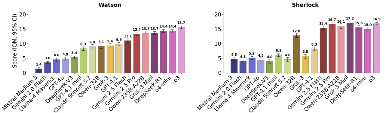
Figure 10. IQM Score of 17 state-of-the-art LLM Hanabi agents over two to five-player settings. Error bars denote 95% CI.
