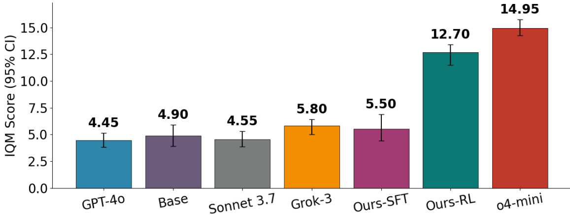
Figure 14. Sherlock: IQM scores of Qwen3-4B-Instruct-2507 (Base) before and after instruction tuning on HanabiLogs (Ours-SFT) and RL on HanabiRewards (Ours-RL) vs Grok-3, Claude Sonnet 3.7 GPT-4o and o4-mini. Note: We evaluated the Qwen3-4B-Instruct-2507 models on different seeds to avoid potential leakage (see App. B.2). Error bars denote 95% CI.
