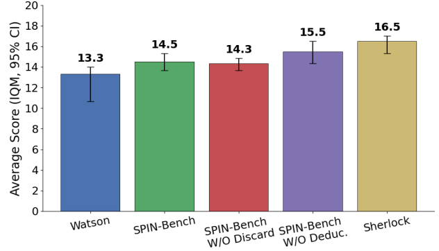
Figure 16. IQM score with different prompt strategies for 10 runs of a 5-player game with Grok-3-mini. Error bars denote 95% CI
