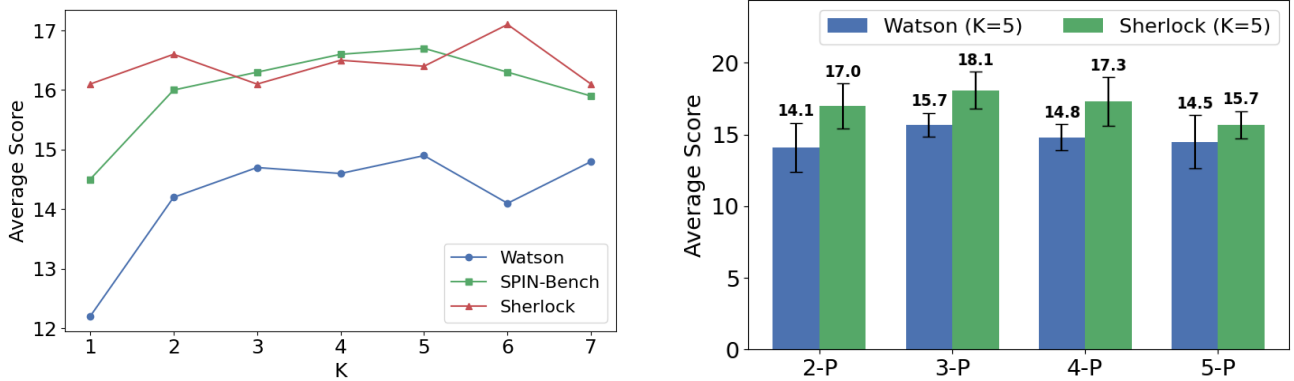
(a) Best-of-K average Hanabi score with the Watson prompt, SPIN-Bench prompt, and our Sherlock prompt, averaged over 10 runs on the 5-player Seed 3 setting.
