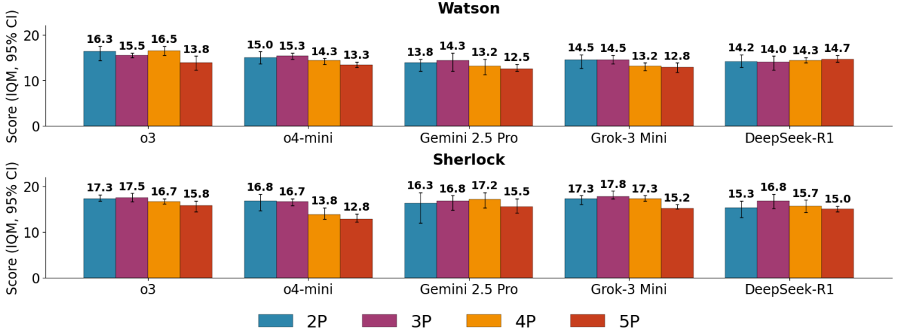
Figure 11. IQM score of top-performing reasoning LLM based Hanabi agents when varying player count from 2 to 5. Error bars denote 95% CI.
