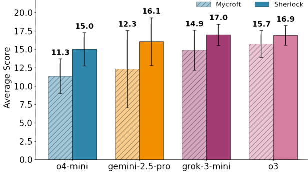
Figure 6. Average Hanabi scores for the best reasoning LLM agents with Implicit deductions (Mycroft) vs Game Engine deductions (Sherlock) averaged across 2–5 Player settings. Error bars denote standard deviation.
