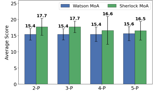
(b) Mixture of Agents (MoA) average score with the Watson and Sherlock prompting strategies across 2–5 player settings. All settings use six agents (Section E.2), except 2-player, which omits the History Agent.
