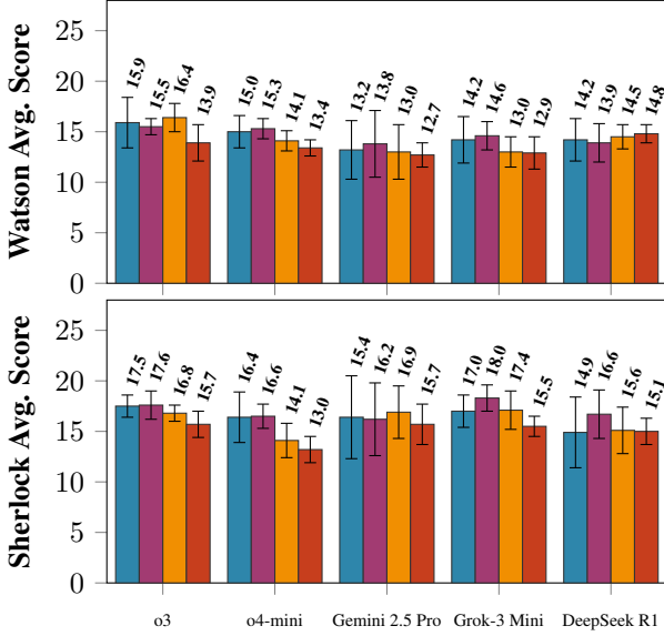
Figure 5. Average score of top-performing reasoning LLM based Hanabi agents when players count varies (2 Players, 3 Players, 4 Players, 5 Players). Error bars denote standard deviation.
