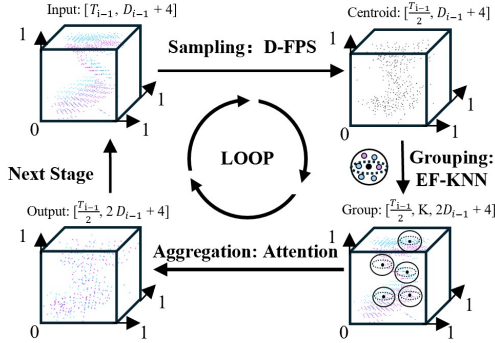
Figure 4. Visualization of Event Cloud’s coordinates and features dimension during hierarchy structure. The closer to the end of the loop, the fewer the number of events and the greater the feature dimension.
