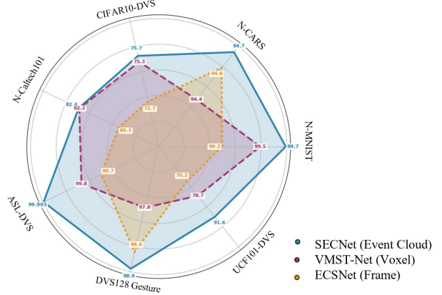
Figure 1. The comparison with the SOTA voxel-based VMST-Net (Liu et al., 2023) and frame-based methods ECSNet (Chen et al., 2022b) on seven classification datasets.
