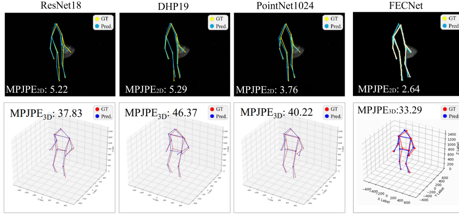
Figure 7. Human pose estimation results in visualization for different models. The first row shows the results in 2D (yellow for ground truth, blue for prediction). The second row shows the results in 3D (red for ground truth, blue for prediction).
