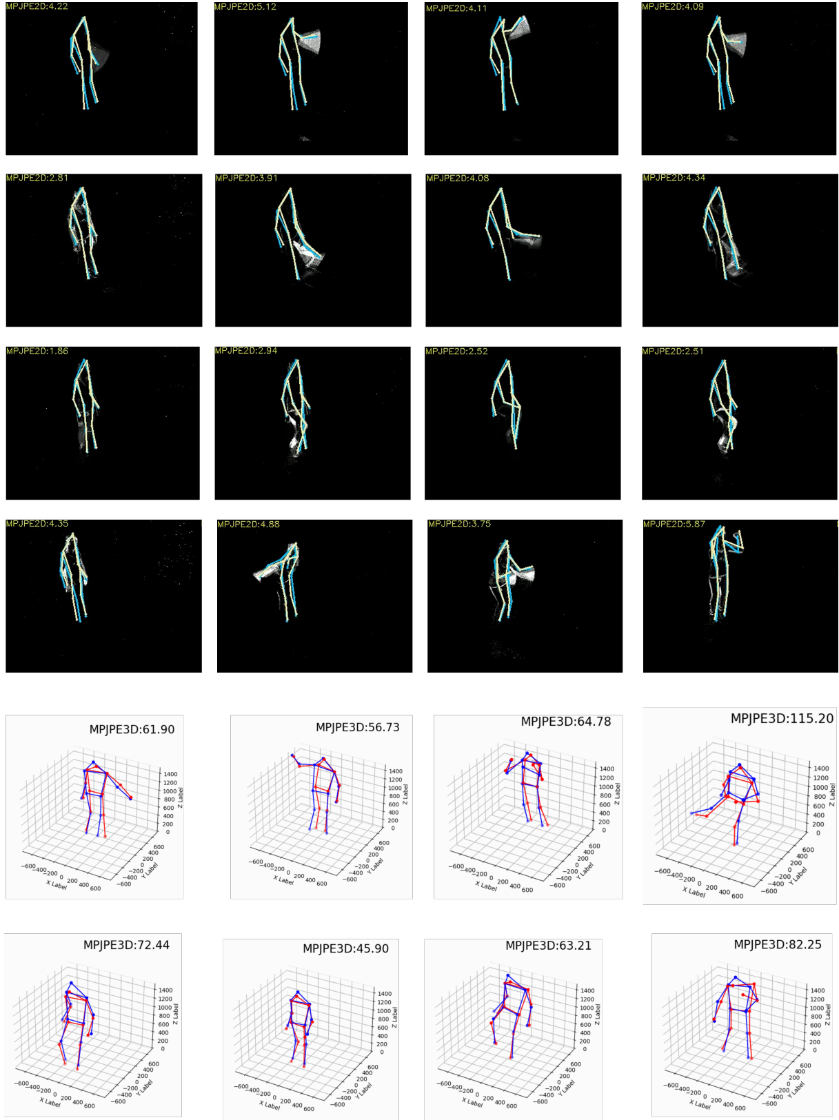
Figure 8. More 2D and 3D SECNet's results in DHP19 dataset.
