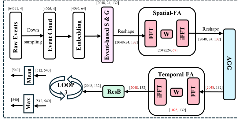
Figure 5. Specific variation of dimensions of a sample in SECNet.
