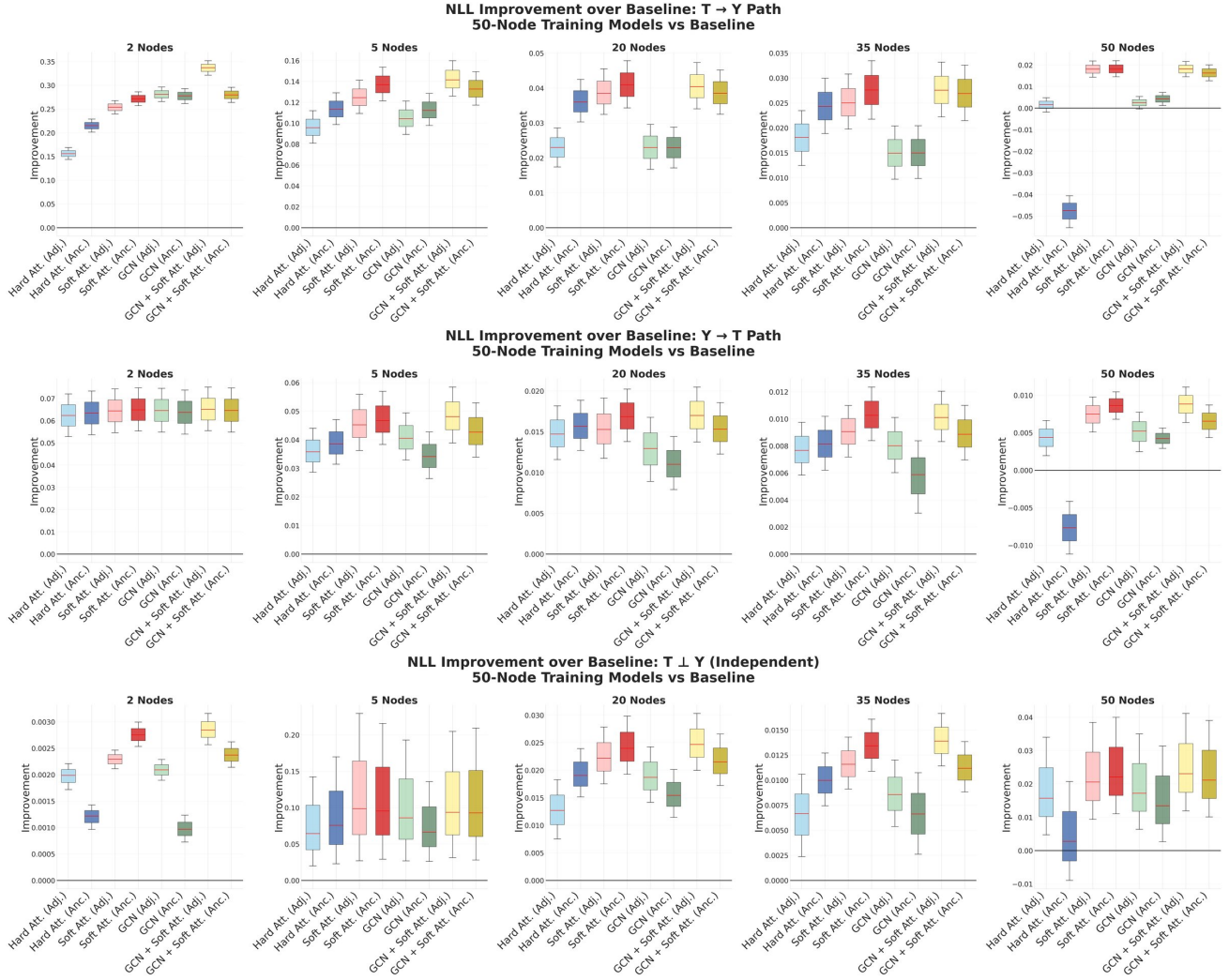
Figure 10. Results, measured in terms of negative log-likelihood (NLL) on held-out test data, for the different graph-conditioning methods evaluated on synthetic data generated from SCMs with linear mechanisms and Gaussian noise. Overall, the graph-conditioned models substantially outperform the baseline that does not use graph information. One notable exception occurs in the 50-node setting: using hard attention together with ancestry-based conditioning leads to very poor performance, indicating instability of this approach. Importantly, this failure mode does not appear for smaller numbers of nodes. Apart from this exception, we consistently observe that using soft attention alone, or soft attention combined with a GCN-based conditioning mechanism, yields the best performance across all node counts and across all SCM variants ( T \rightarrow Y , Y \rightarrow T , and T and Y independent).
