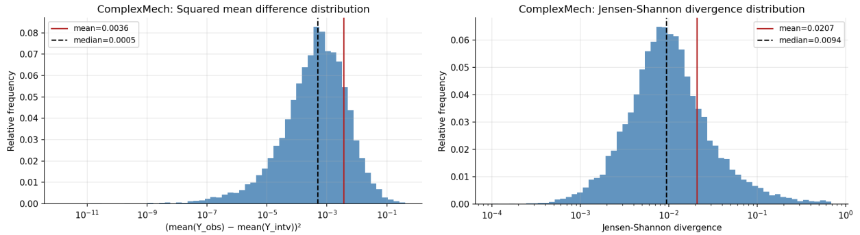
Figure 7. Distribution of squared mean differences (left) and Jensen–Shannon (JS) divergences (right) between p(y \mid \text{do}(t), \psi) and p(y \mid t, \psi) across 10,000 SCMs. Both axes are shown on a logarithmic scale. The mean squared difference is 0.0036 and the mean JS divergence is 0.0207. Both metrics exhibit heavy-tailed behaviour, indicating that while most causal effects are small, larger effects occur with non-negligible probability.
