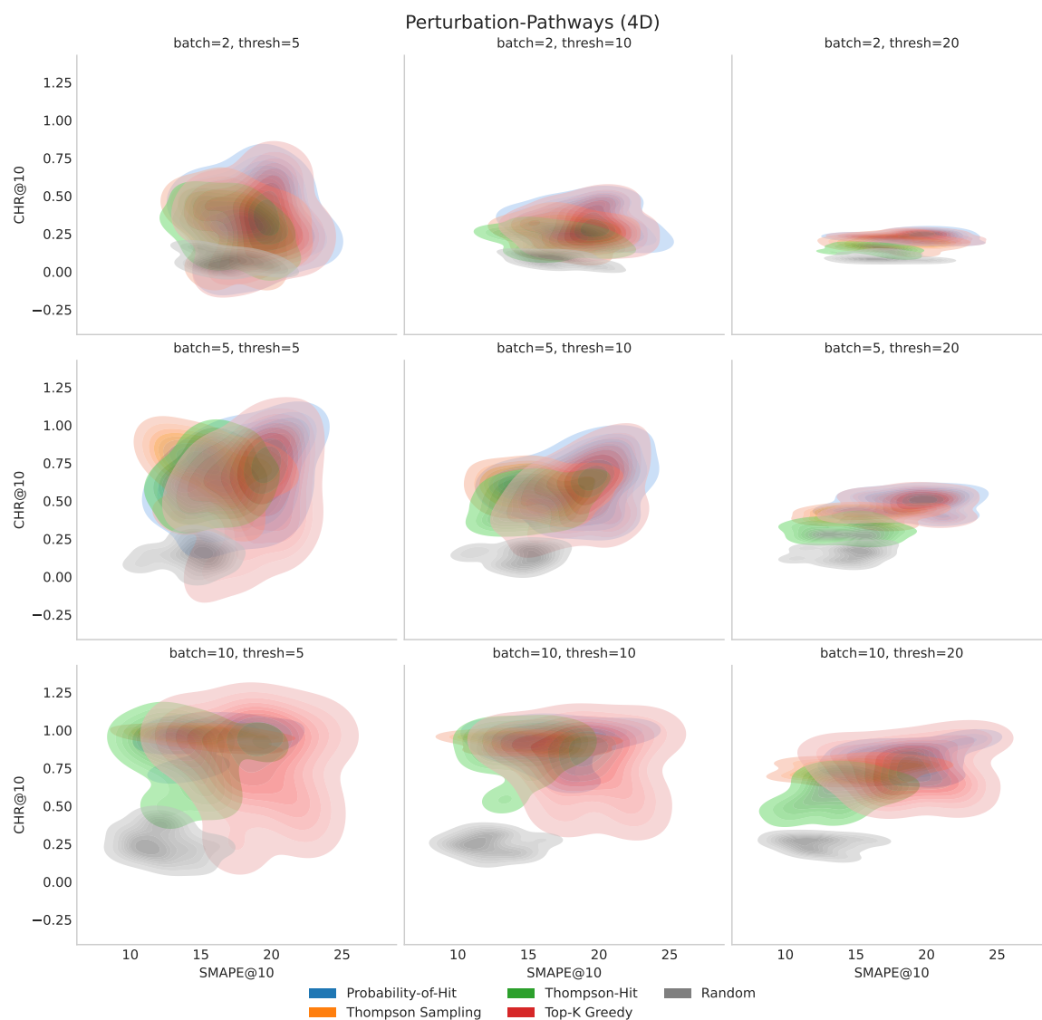
Figure 8. Trade-off between CHR@10 and SMAPE@10 on Perturbation-Pathways (4D) across acquisition functions, batch sizes, and thresholds.
