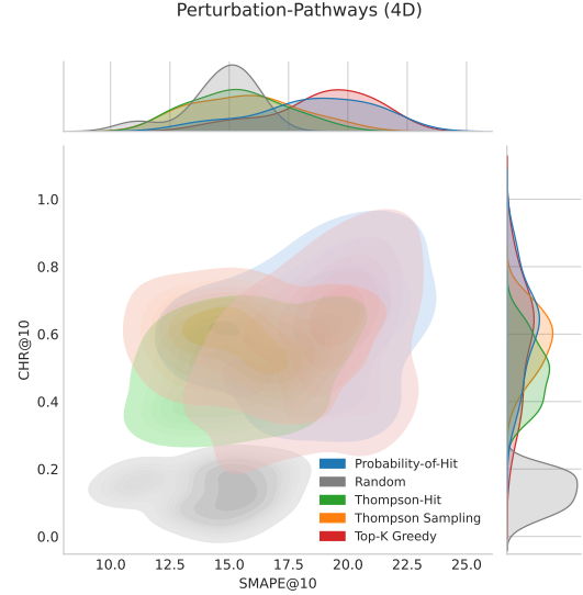
Figure 4. Trade-off at b = 5 between CHR@10 and SMAPE@10 on Perturbation-Pathways (4D) across acquisition functions.
