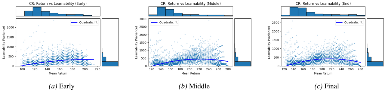
Figure 16. Learnability vs. return over training in Coordination Ring .
