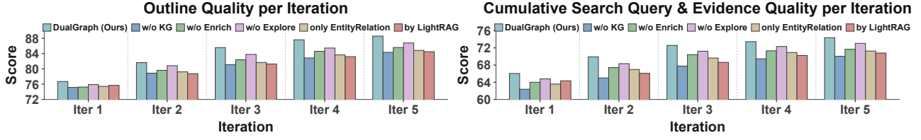
Figure 3. Comparison of DualGraph variants across iterations. Early stopping is disabled for all variants to ensure fair comparison. Left: Outline quality. Right: Search query and evidence quality.
