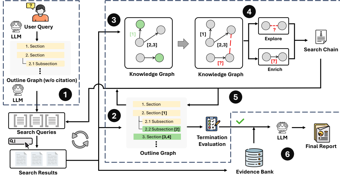
Figure 2. Overview of our DualGraph framework. ① shows the OG initialization, ②–⑤ show the co-evolving iteration of KG and OG, and ⑥ shows the report finalization after the iteration termination.
