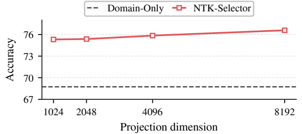
Figure 5. Average performance of NTK-Selector using different projected dimensions.
