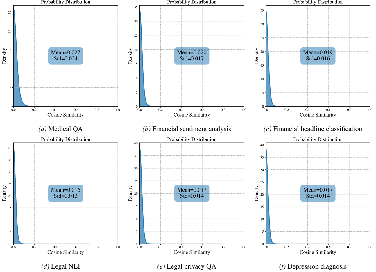
Figure 6. Gradient similarity of cross output of LLAMA3-8B-INSTRUCT on different tasks.
