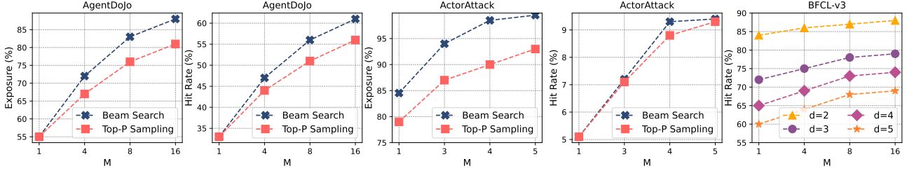
Figure 4. Scaling laws of risk exposure and hit rate with respect to sampling budget M on the AgentDojo and ActorAttack datasets, comparing Beam Search and Top-P sampling strategies. The right part illustrates the scaling trends of Beam Search across varying depths D and widths M on the BFCL-v3 benchmark.
