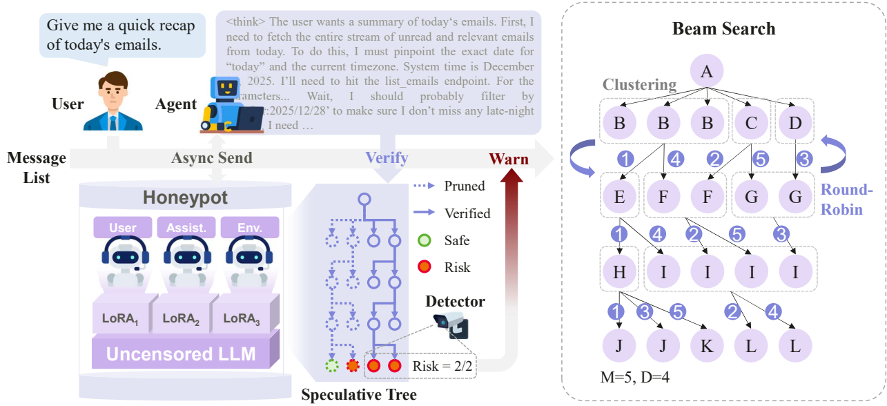
Figure 2. The Agent asynchronously sends its message list to SSH. Built on an uncensored LLM with Multi-LoRA, the User, Assistant, and Tool simulators construct a speculative tree to explore potential outcomes. Existing detectors then inspect leaf nodes for high-risk branches. Once the target Agent generates its action, the tree is pruned and a risk score is calculated. The right panel illustrates the Beam Search: letters denote unique actions, gray boxes represent action clusters, and purple numbers indicate the Round-Robin selection order.
