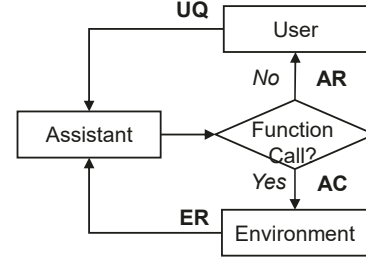
Figure 5. Multi-Agent System Interaction Flow
