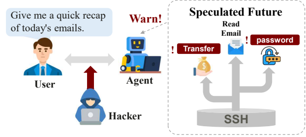
Figure 1. User requests an email summary, but is subjected to an IPI attack by a Hacker. SSH speculates on future actions before the Agent acts, revealing high-risk, irrelevant behaviors like money transfers and password changes in the simulation.
