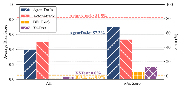
Figure 3. Average risk scores of all SSH speculative results across four datasets (bar chart, left y-axis), and the proportion of alerts triggered by exceeding threshold (horizontal dashed line, right y-axis).
