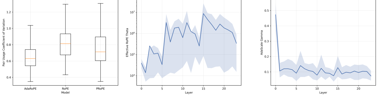
Figure 3. Left: AdaRoPE yields a lower coefficient of variation (CoV) across dimensions compared to RoPE and PRoPE, indicating a more balanced utilization of frequencies. The box plot represents the min, max, 25th and 75th percentiles, and the mean across all heads. Middle: The effective RoPE base \Theta exhibits an increasing trend with network depth, suggesting that deeper layers prioritize learning lower frequencies. Right: The AdaScale parameter \gamma peaks in the initial layer and rapidly stabilizes around 0.1 in subsequent layers. In the Middle and Right plots, we plot the mean value across heads in the same layer, and shaded regions denote the 0.1–0.9 quantile range.
