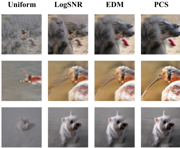
(b) ImageNet-iPNDM sampler with NFE=7.
