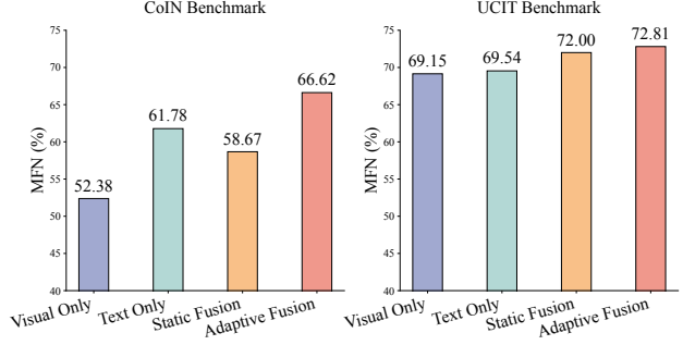
Figure 3. Ablation study on modality fusion strategies.
