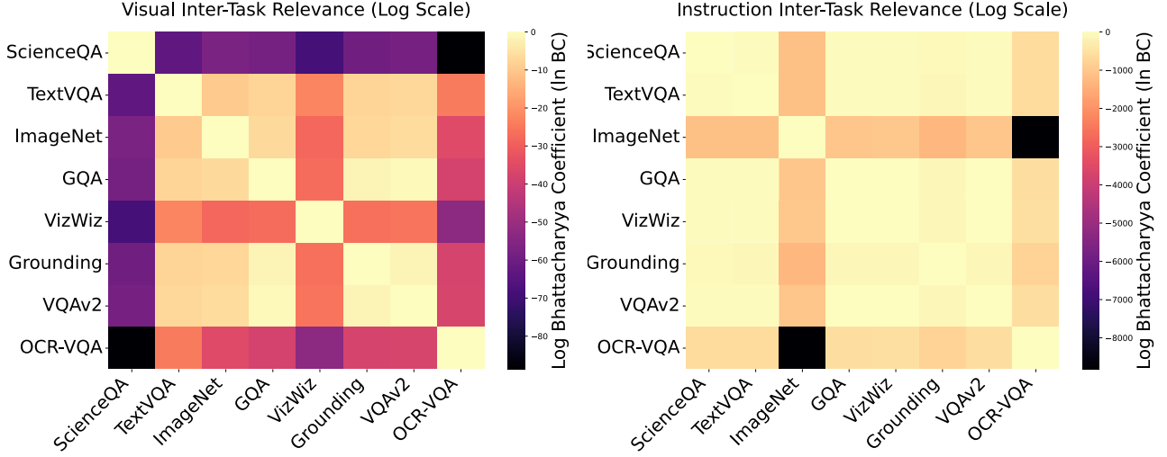
Figure 6. Log-scale Inter-task Relevance Matrices on CoIN Benchmark
