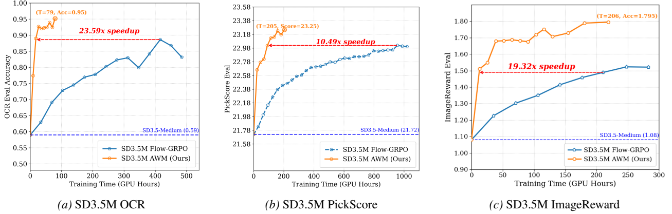
Figure 9. OCR, PickScore, and ImageReward training efficiency with early experiment configurations. Metric vs. GPU hours for SD3.5M. AWM (ours) exceeds Flow-GRPO with far less compute.
