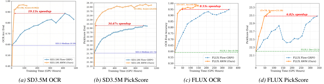
Figure 5. OCR and PickScore training efficiency. Metric vs. GPU hours for SD3.5M and FLUX. AWM (ours) exceeds Flow-GRPO with far less compute.
