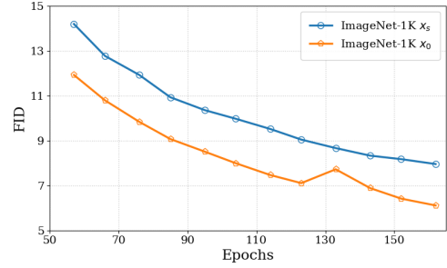
(b) FID on ImageNet-64
