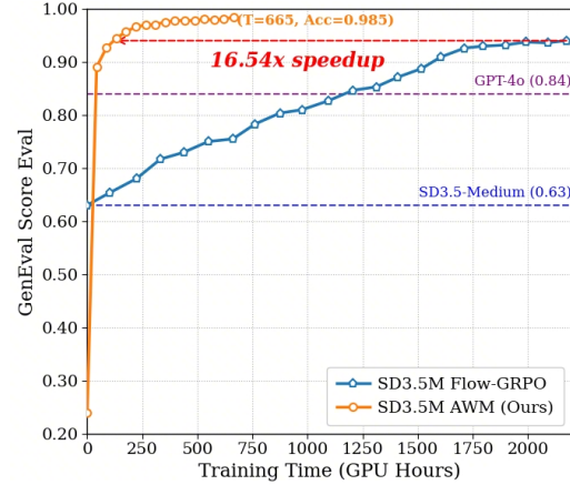
(a) Faster Convergence
