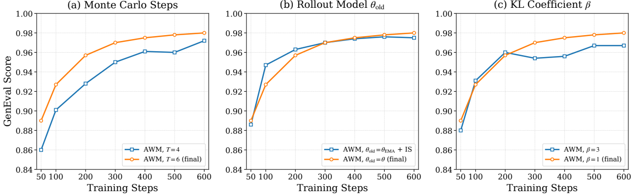
Figure 7. Ablations on SD3.5M and GenEval. (a) Number of Monte Carlo steps T ; (b) rollout model \theta_{old} , where \theta_{EMA} + IS denotes sampling from an EMA copy of the online model and applying the importance-sampling correction in Equation (15); (c) KL regularization coefficient \beta . Curves show GenEval score vs. training steps.
