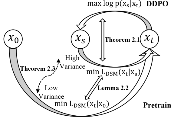
Figure 2. Overview of our analysis: DDPO is equivalent to denoising score matching with noisy target (Theorem 2.1); although the population minimizer is unchanged (Lemma 2.2), this noisy target introduces higher variance (Theorem 2.3), leading to slower optimization.
