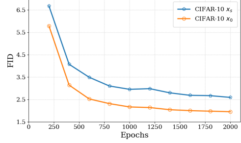
(a) FID on CIFAR-10
