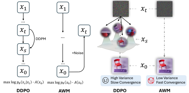
(b) Formulations: DDPO vs. AWM
