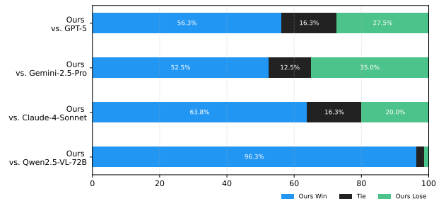
Figure 5. Human evaluation on Design2Code-HARD.
