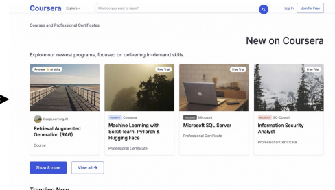
Figure 11. UI2Code N Demo Cases: UI Editing (1/2)
