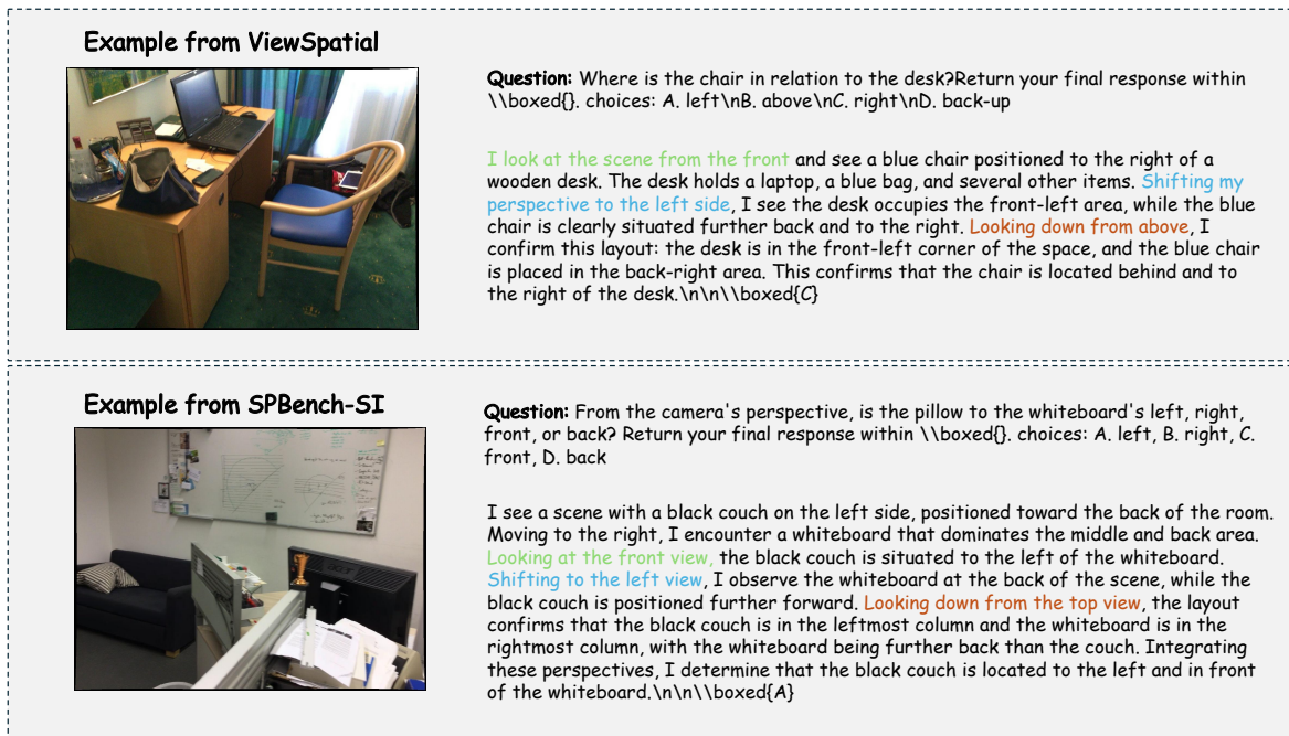
Figure 14. Case study of 3ViewSense reasoning on external benchmarks. We show qualitative examples from ViewSpatial and SPBench-SI, illustrating how 3ViewSense transfers the learned view-grounded reasoning process to external spatial reasoning tasks.
