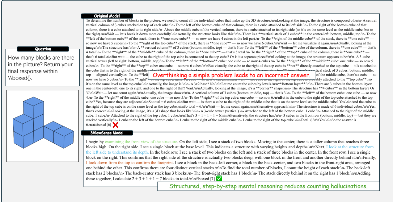
Figure 13. Qualitative examples of model responses on block counting under occlusion. Compared to the base model, 3ViewSense produces more concise and structured reasoning, improving robustness and accuracy.
