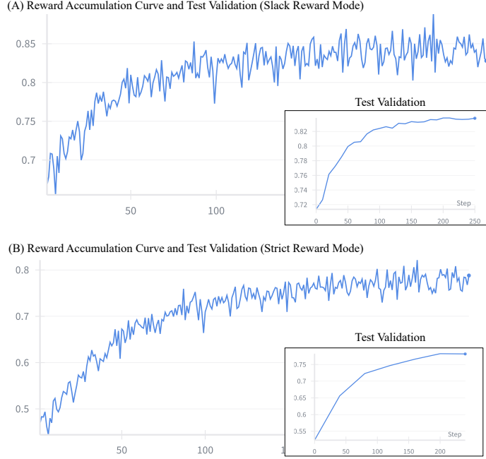
Figure 12. Cumulative reward curves during GRPO-based RL refinement. We report the training dynamics under two reward settings: strict reward (exact match) and slack reward (partial credit) as defined in Section 3.3.
