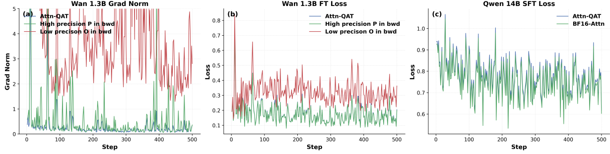
Figure 3. Training dynamics for diffusion and language models. (a–b) Gradient norm and loss during Wan 2.1 1.3B finetuning under different Attn-QAT configurations. (c) Finetuning loss curves of Qwen3-14B comparing BF16 attention and Attn-QAT.
