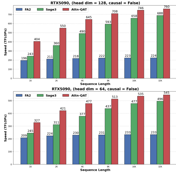
Figure 5. Kernel throughput on RTX 5090. We compare attention kernel performance with head dimensions 128 (top) and 64 (bottom), using a batch size of 16 and 16 attention heads. All results report end-to-end throughput.
