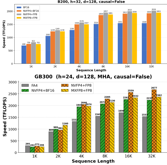
Figure 6. B200 ( h=32 , top) and GB300 ( h=24 , bottom) attention throughput (TFLOPS). NVFP4 + BF16 means NVFP4 QK + BF16 PV GEMMs. On GB300, peak NVFP4+FP8 is 1.74\times over BF16 FA4 at 32K.
