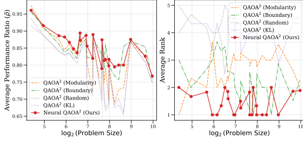
Figure 3. Problem Size Generalization. We evaluate Neural QAOA 2 on test instances ranging from N = 21 to N = 1000 (plotted on a \log_2 scale). The left panel shows the mean \bar{\rho} , and the right panel shows the average rank. Our method (red line) maintains superior ranking stability across the spectrum, effectively generalizing to instances with scales unseen during training.
