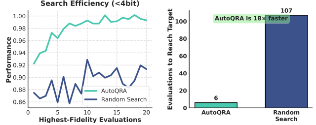
Figure 5. Search efficiency analysis. (Left) Best validation performance versus the number of evaluations at the largest search budget b_S . AutoQRA improves rapidly and consistently performs better than random search. (Right) Number of largest-budget evaluations required to reach a target accuracy. AutoQRA needs 6 evaluations compared to 107 for random search, yielding an 18 \times reduction in expensive evaluations.
