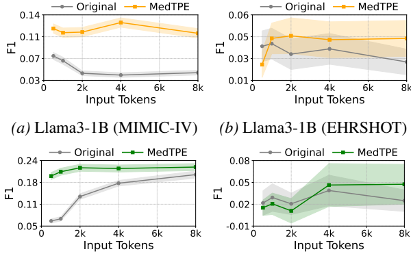
Figure 4. Context length robustness of MedTPE. Each plot shows the mean F1 score with 95% confidence interval (shaded areas).
