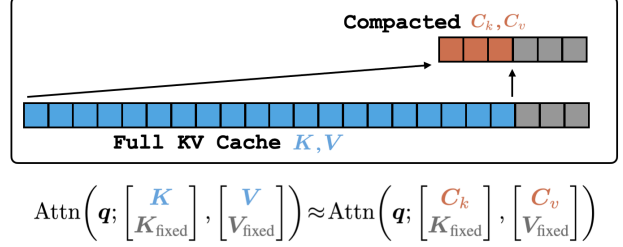
Figure 2. KV compaction via Attention Matching. We replace the full KV cache (\mathbf{K}, \mathbf{V}) with a smaller cache (\mathbf{C}_k, \mathbf{C}_v) chosen so that attention outputs are approximately preserved when the compacted prefix is concatenated with arbitrary fixed or future tokens (\mathbf{K}_{\text{fixed}}, \mathbf{V}_{\text{fixed}}) .
