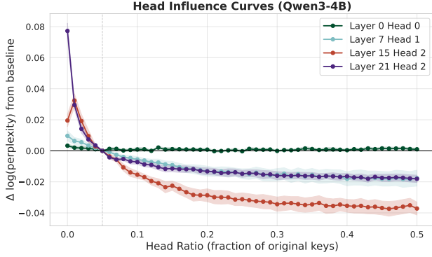
Figure 3. Head sensitivity curves in Qwen3-4B. We fix all KV heads to a baseline compaction ratio of 0.05\times and vary the compaction ratio of a single head. We report the change in loss relative to the baseline (lower is better) as a function of the varied head’s compaction ratio. Curves are averaged over 10 QuALITY articles; shaded regions denote \pm 1 standard error of the mean across articles. Some heads (e.g., L0H0) are largely insensitive to additional capacity, whereas others (e.g., L15H2) benefit substantially from storing more KV pairs.
