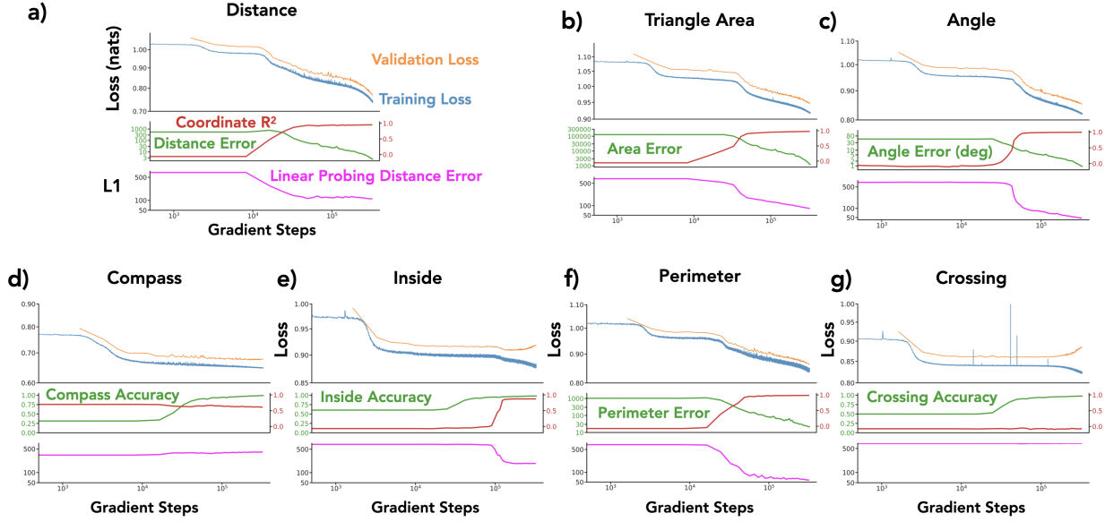
Figure 9. Training dynamics for all single-task models. (a) distance, (b) triangle area, (c) angle, (d) compass, (e) inside, (f) perimeter, (g) crossing. Each panel shows three rows: (top) training loss (blue) and validation loss (orange); (middle) task-specific metric (green, left axis) and linear probe coordinate R^2 (red, right axis); (bottom) linear probing distance error (magenta). All plots use log-scale x-axis for gradient steps.
