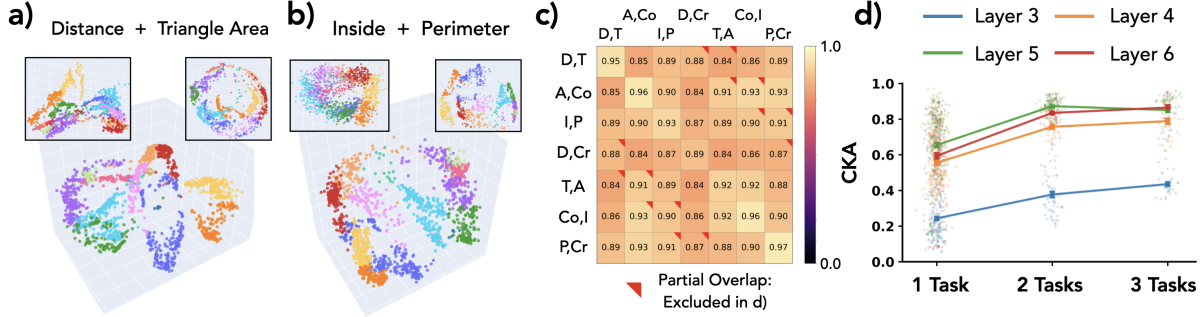
Figure 3. Multi-task pretraining drives representational convergence. (a,b) Two-task training creates more regular structures than single-task models. (c) CKA matrix (7x7) for two-task models shows higher alignment (see App. Fig. 12 for s.e.m.). (d) Average CKA increases with task count (1→2→3), saturating at \sim 0.85 for layers 4-6 while layer 3 continues improving (see App. Fig. 13 for s.e.m.). Crossing, which failed to learn in single-task training, is excluded; including it would only strengthen the convergence finding.
