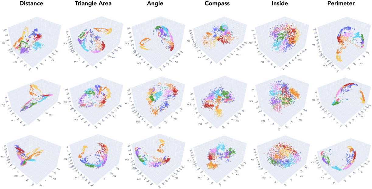
Figure 8. Representation visualizations for single-task models across multiple seeds. Each column shows a different task; each row shows a different random seed. Cities are colored by geographic region.
