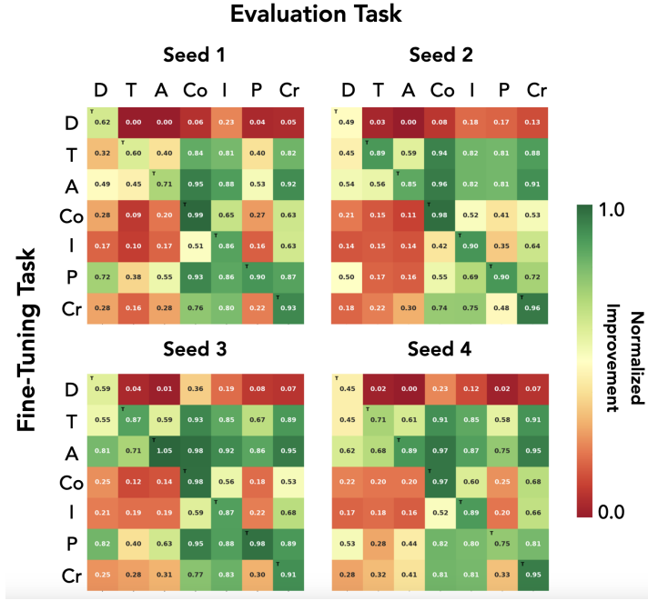
Figure 16. Single-task fine-tuning results for individual seeds. Per-seed version of Fig. 5(a), organized in a 2×2 grid.
