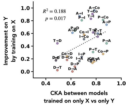
Figure 15. Annotated version of Fig. 5(b). Each point is labeled with its (train → eval) task pair. D=distance, T=triangle area, A=angle, Co=compass, I=inside, P=perimeter.
